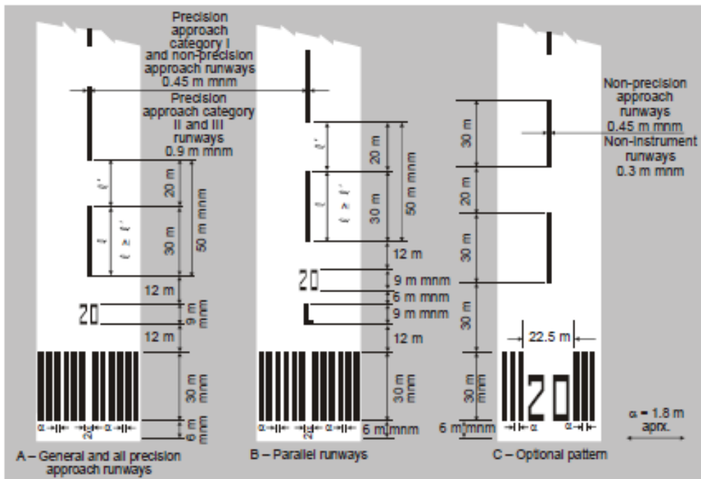
Figure 5-2. Runway designation, centre line and threshold markings
