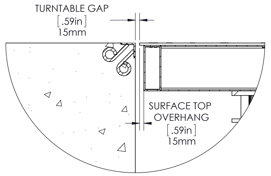
DETAIL J SCALE 1 : 8
