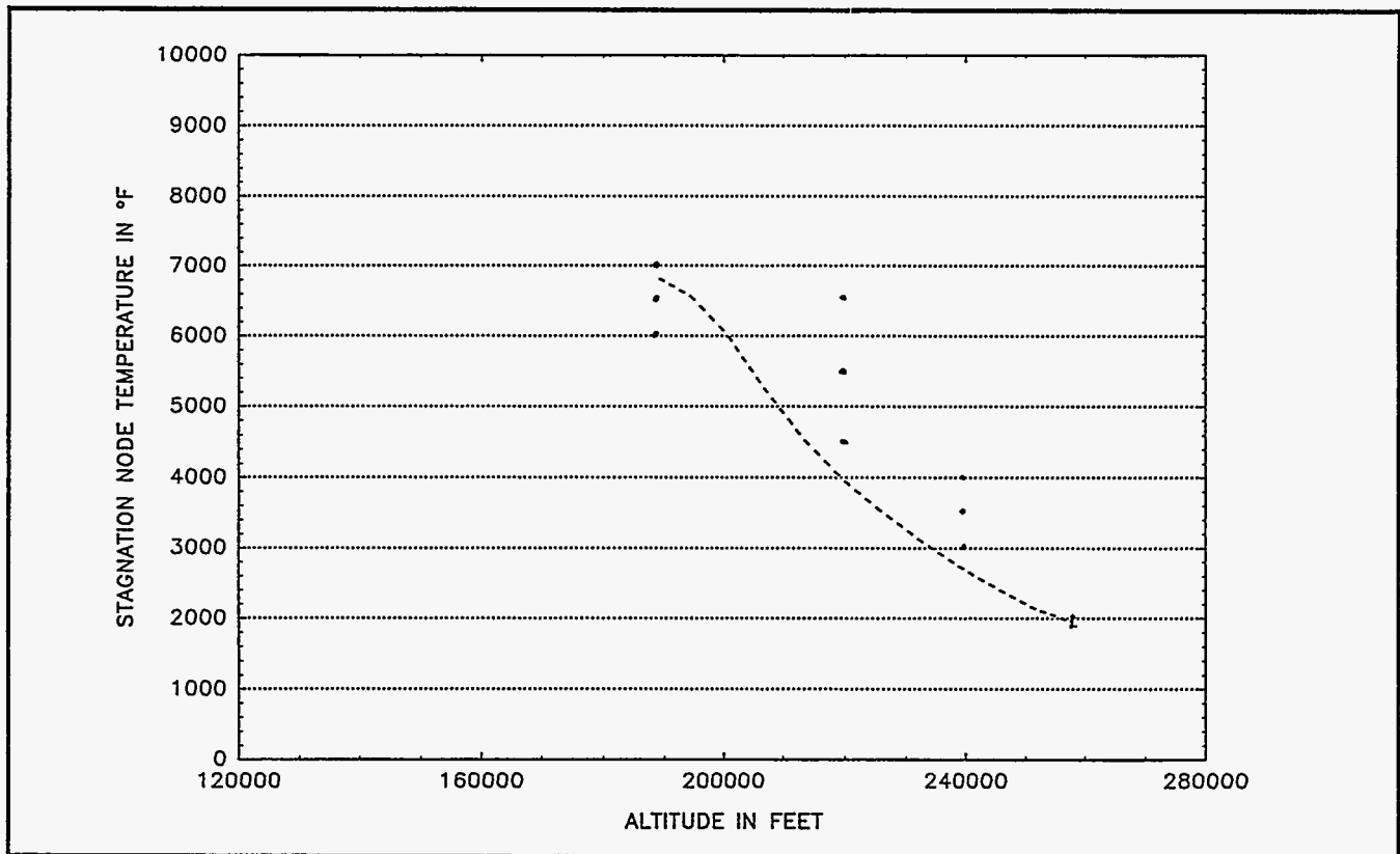
Figure 3-10. Stagnation Node Temperature Vs. Altitude
