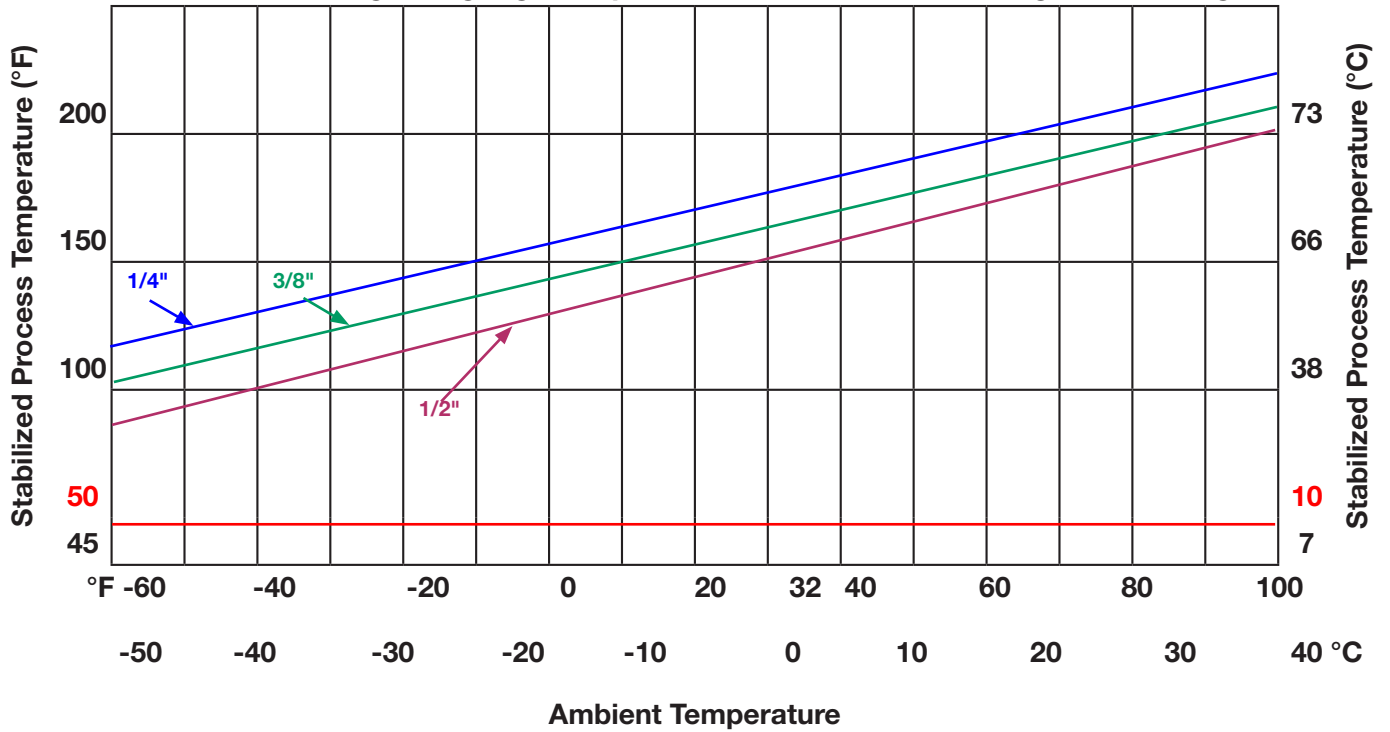
250 SH Self-Regulating High Temperature Heater 10 watt/ft - Single Tube Designs 121
