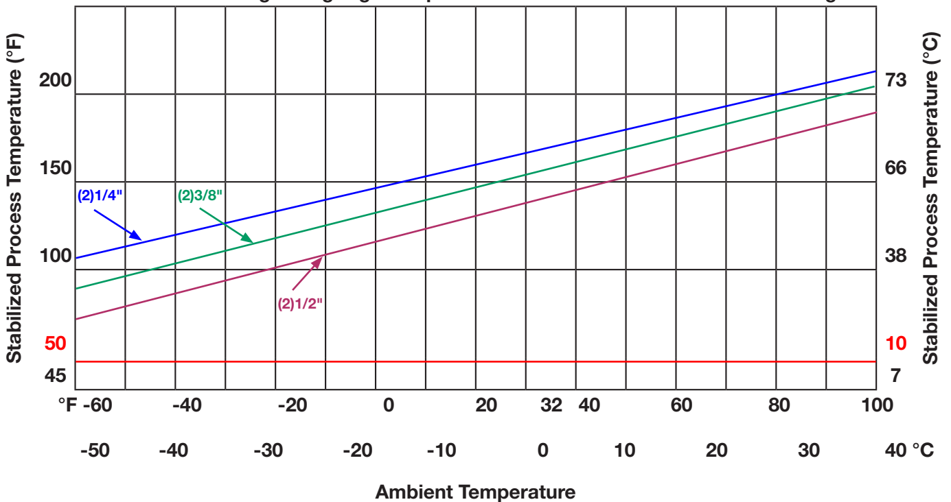
250 SH Self-Regulating High Temperature Heater 10 watt/ft - Dual Tube Designs 121
