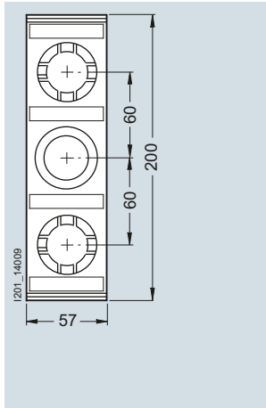
5SH2242 (1-fold: a = 57 mm)
