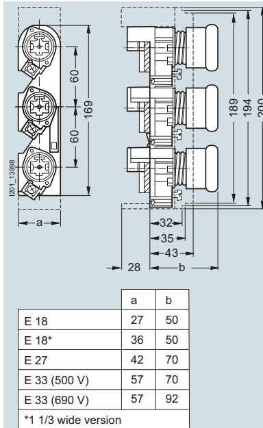
5SF6018, 5SF6020 (b = 70 mm)
