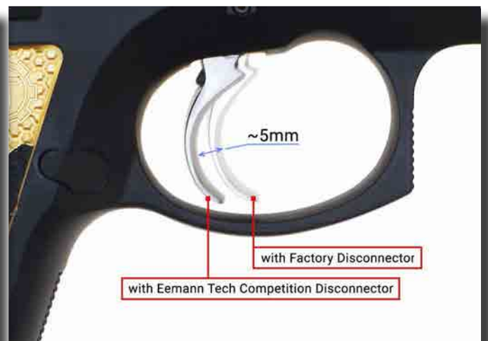
CZ 75 SP-01 Shadow
