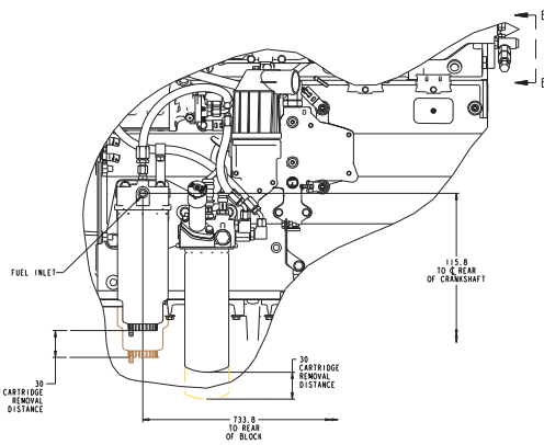
DETAIL OF FUEL FILTER HEAD ASM SCALE 1:2
