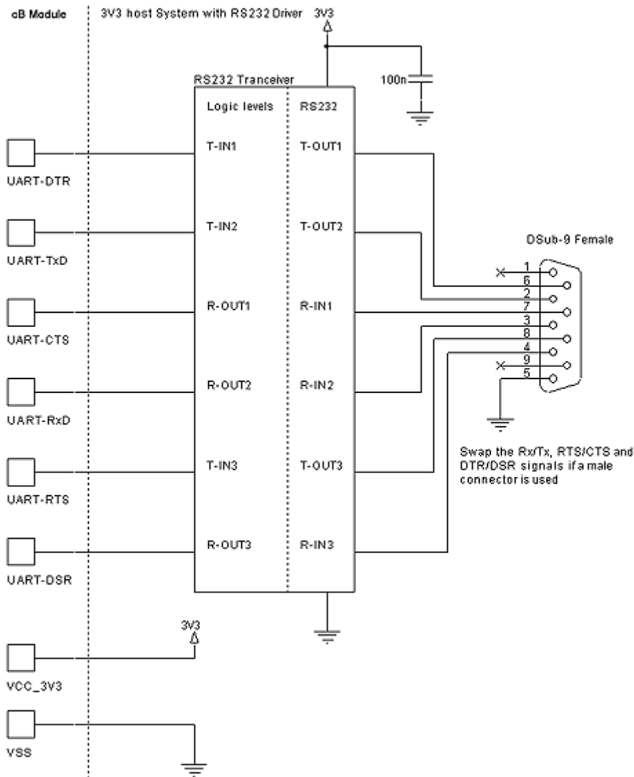
Figure 13: A complete RS232 interface.
