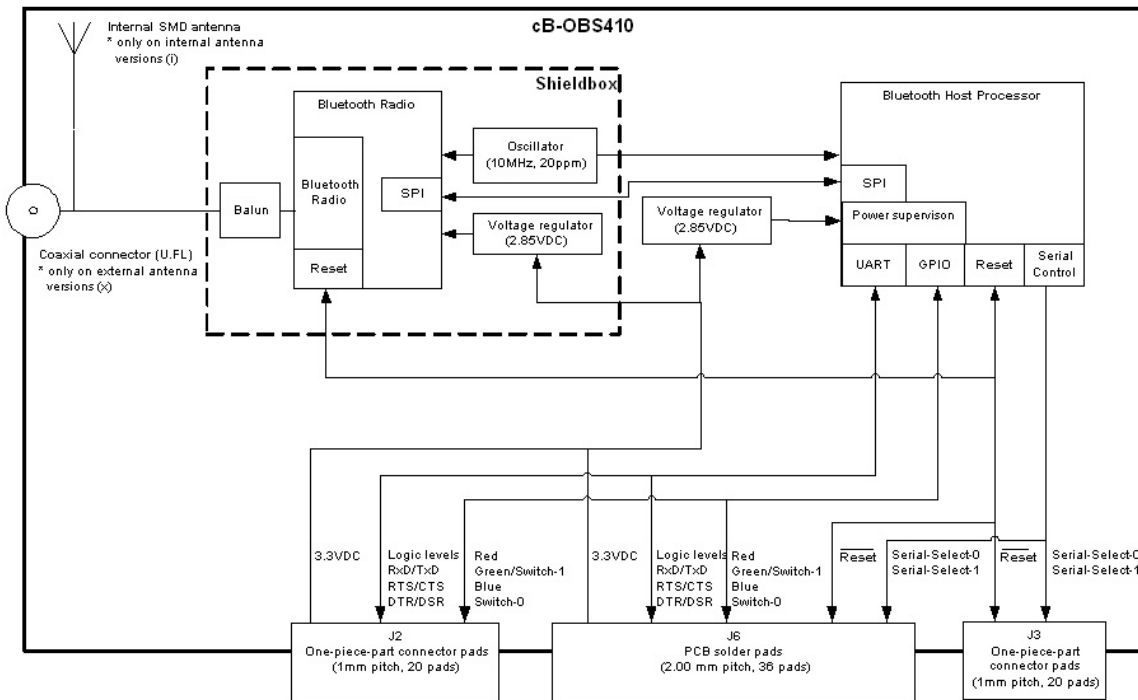
Figure 2: Block diagram of cB-OBS410
