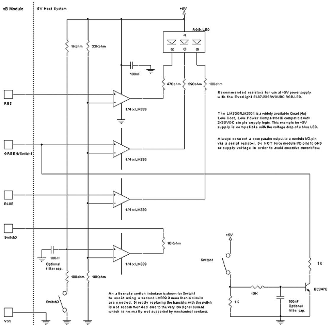
Figure 30: A complete 5V host interface with operational amplifier.
