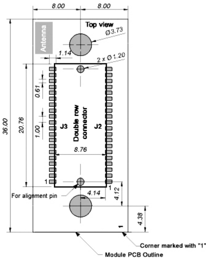
Figure 8: Host PCB layout [mm] for double row connector.
