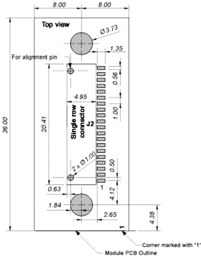
Figure 7: Host PCB layout [mm] for single row connector.
