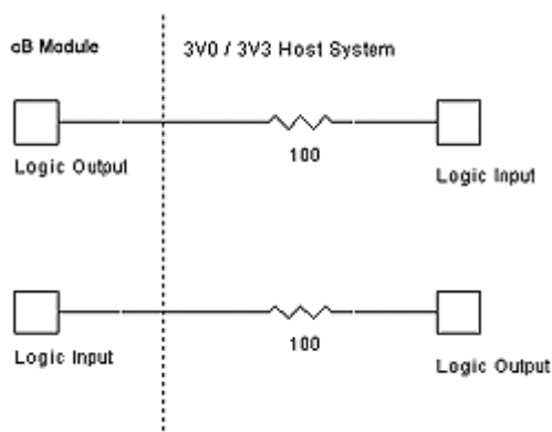
Figure 10: Logic levels interface to a 3/3.3V system. A protective 100Ohm resistor is used.
