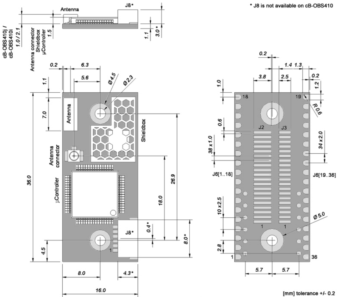
Figure 5: cB-OBS410 dimensions.
