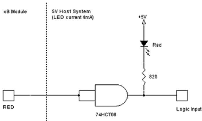
Figure 19: A red LED in a 5V host system. The status of the signal can also be used as input to a host controller.
