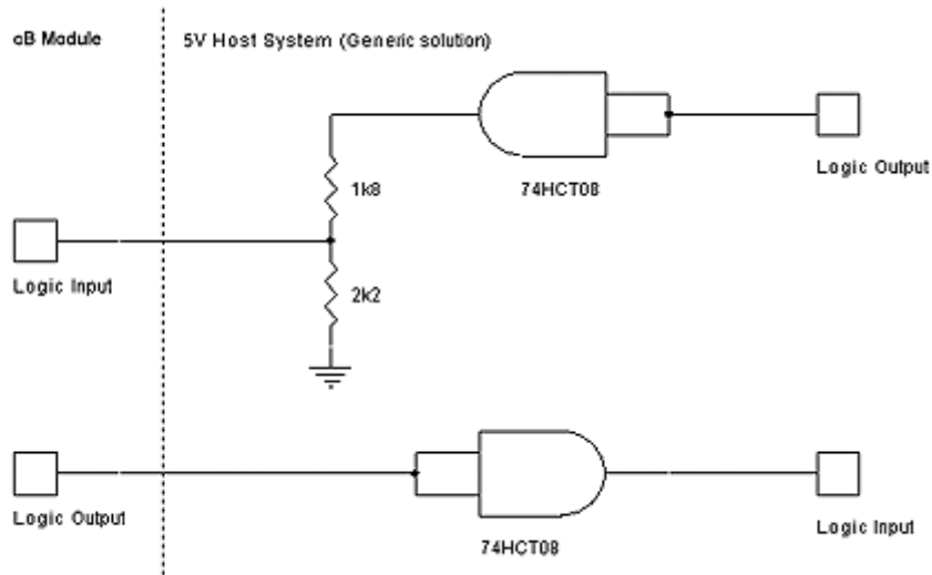
Figure 11: Interface example with logic levels to a 5V system. The gate converting from host 5V output to module input can be replaced with an LVC gate if the voltage divider is removed.
