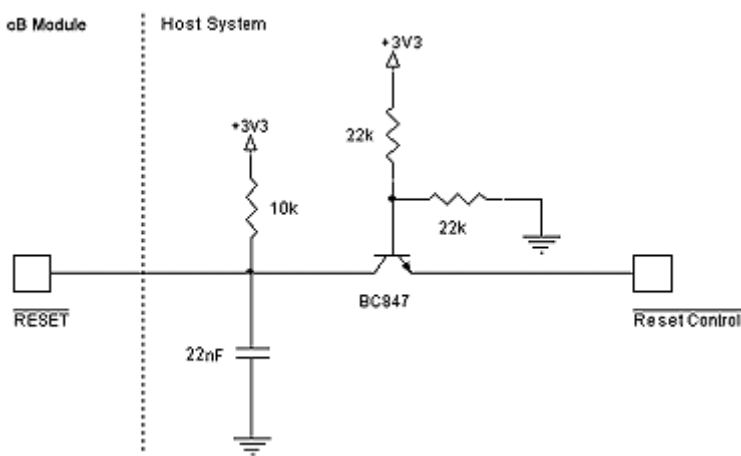
Figure 29: Design of an open collector reset from an active high output.
