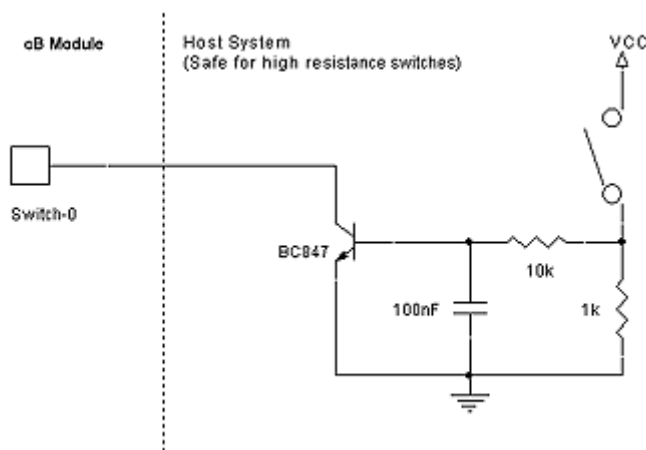
Figure 27: If the resistance in the switch is not guaranteed to be low enough, a safer design can be used.
