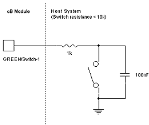
Figure 24: A low resistance restore switch used. Notice the 1kOhm serial resistor.
