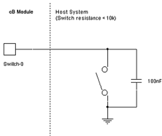
Figure 26: A low resistance function switch used.
