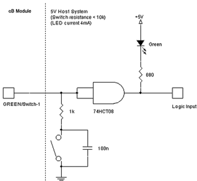
Figure 21: Switch-1 used together with a green LED in a 5V host system. The status of the signal can also be used as input to a host controller. Notice the 1kOhm serial resistor.
