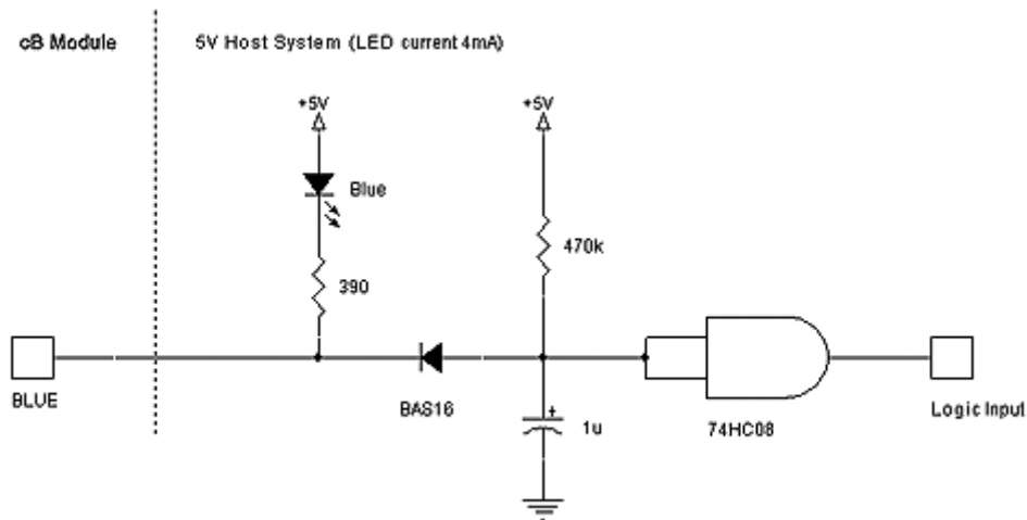
Figure 17: A Low pass filter and a 74HC08 suppresses the flashes when the module is sending and receiving data. The Blue LED can be removed if not required. The values are not suitable in all applications and need to be verified in a specific application.
