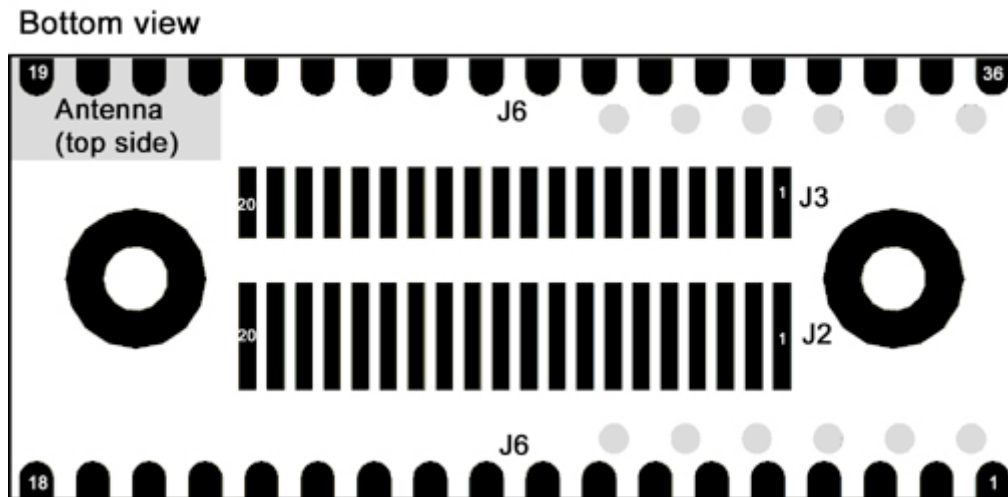
Figure 4: Bottom view of the PCB with the pin numbering of the J2, J3 and the J6 connectors.
