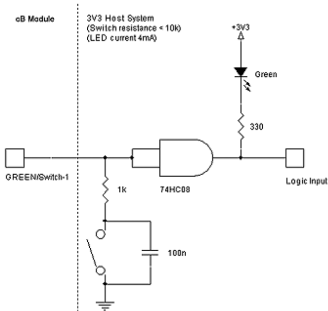
Figure 20: Switch-1 used together with a green LED in a 3.3V host system. The status of the signal can also be used as input to a host controller. Notice the 1kOhm serial resistor.
