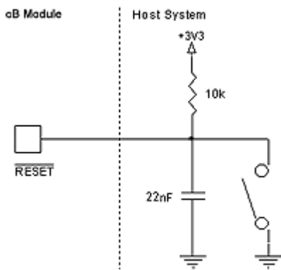
Figure 28: A reset switch.
