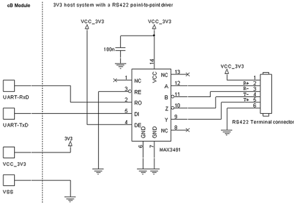
Figure 14: A complete RS422 interface.
