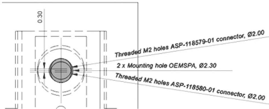
Figure 6: The 2.3mm mounting holes [mm].
