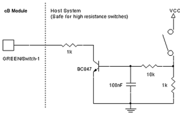
Figure 25: If the resistance in the switch is not guaranteed to be low enough, a safer design can be used. Notice the 1kOhm serial resistor.
