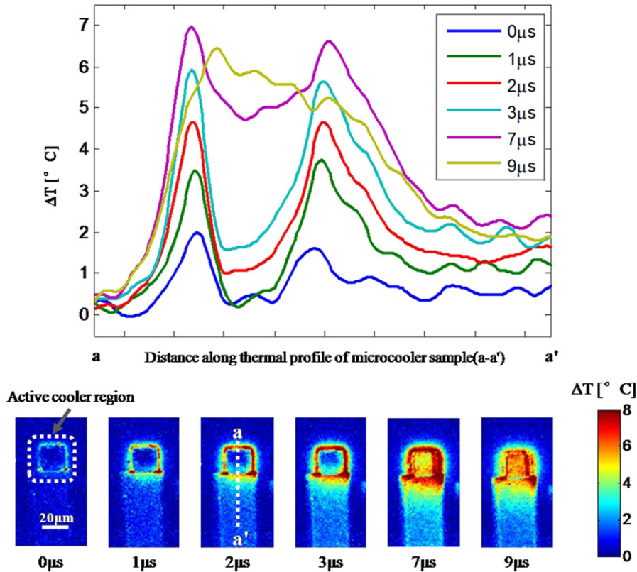
Figure 14. Fast TTR CCD images and profile for a 20 \times 20 \mu\text{m} thermionic micro-cooler. Image sequence shows transient thermal response in the sample during the first 9 \mu\text{s} of device excitation with a 700 mA pulse. Thermal images result from averaging over about 12 000 heating cycles or about 8 min of total accumulation time.
