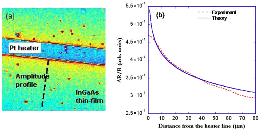
Figure 18. Determining thin film thermal conductivity using thermoreflectance imaging. (a) Thermoreflectance image showing the heat distribution from an active 30 \mu\text{m} wide metal heater line into an underlying InGaAs thin film. (b) Extracting thermal conductivity of thin film by fitting simulated thermal profile (perpendicular to heater axis) to thermoreflectance image data. Thermal images result from averaging over about 8000 heating cycles or about 40 min of total accumulation time. (Reprinted with permission from [73]. Copyright 2008 IEEE.)
