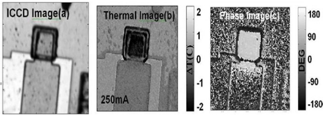
Figure 6. Thermoreflectance imaging using a CCD camera. (a) Blue LED microscope image of a 40 \times 40 \mu\text{m}^2 integrated micro-cooler. (b) Thermoreflectance temperature amplitude image and (c) phase image of the micro-cooler at 250 mA bias. The thermal image results from averaging over 25 000 heating cycles (about 15 min of total accumulation time). (Reprinted with permission from [3]. Copyright 2003 ASME.)
