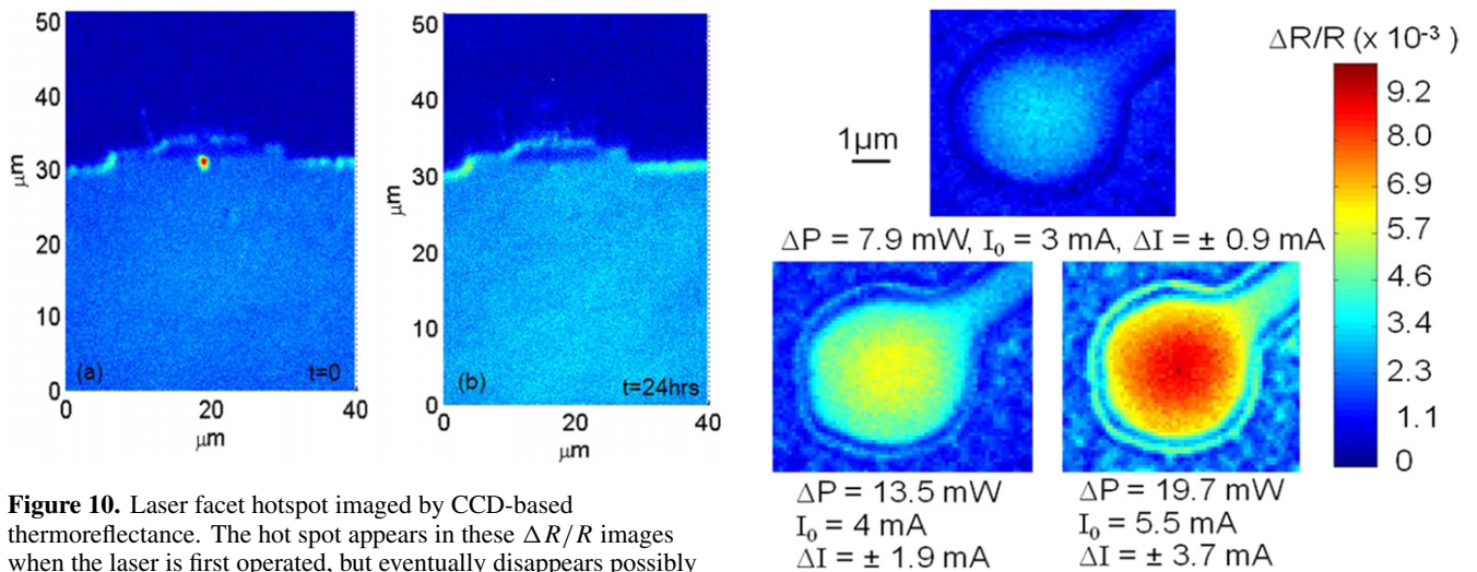
Figure 11. Typical thermoreflectance images of the oxide-confined SM VCSEL at three different dissipated power values. The images result from 6000 heating cycles at f = 15 Hz. (Reprinted with permission from [9]. Copyright 2007 IEEE.)
