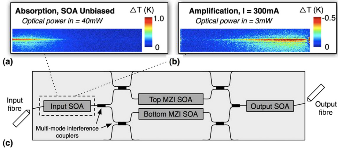
Figure 12. (a) Thermoreflectance image of heating in an unbiased SOA due to optical absorption. Change in temperature is proportional to absorbed optical power, which is largest at the SOA input (left side of image). (b) Thermoreflectance image of cooling in an SOA under normal biasing conditions. Cooling increases near the output of the SOA on the right, as the light is amplified. (c) Schematic of the SOA-MZI PIC from which the measurements were taken. The thermal images in parts (a) and (b) result from 5 \times 10^5 heating cycles at f = 15 Hz, for a total accumulation time of 10 h.
