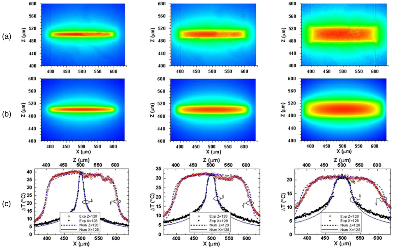
Figure 7. Comparison of experimental and numerical results for a micro-heater device at optimal parameters (a) measured temperature field on gold surface; (b) numerical solution over corresponding area; (c) line slices along mid-planes on the surface of the heater. From left to right: 14 \times 200 , 26 \times 200 and 50 \times 200 \mu\text{m} . The thermal images in part (a) result from averaging over about 1000 heating cycles. (Reprinted with permission from [50]. Copyright 2007 IEEE.)
