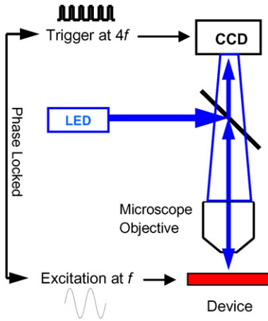
Figure 1. Schematic depiction of a homodyne thermoreflectance microscopy setup.
