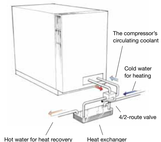
Air-cooled compressor with water-based recovery system
