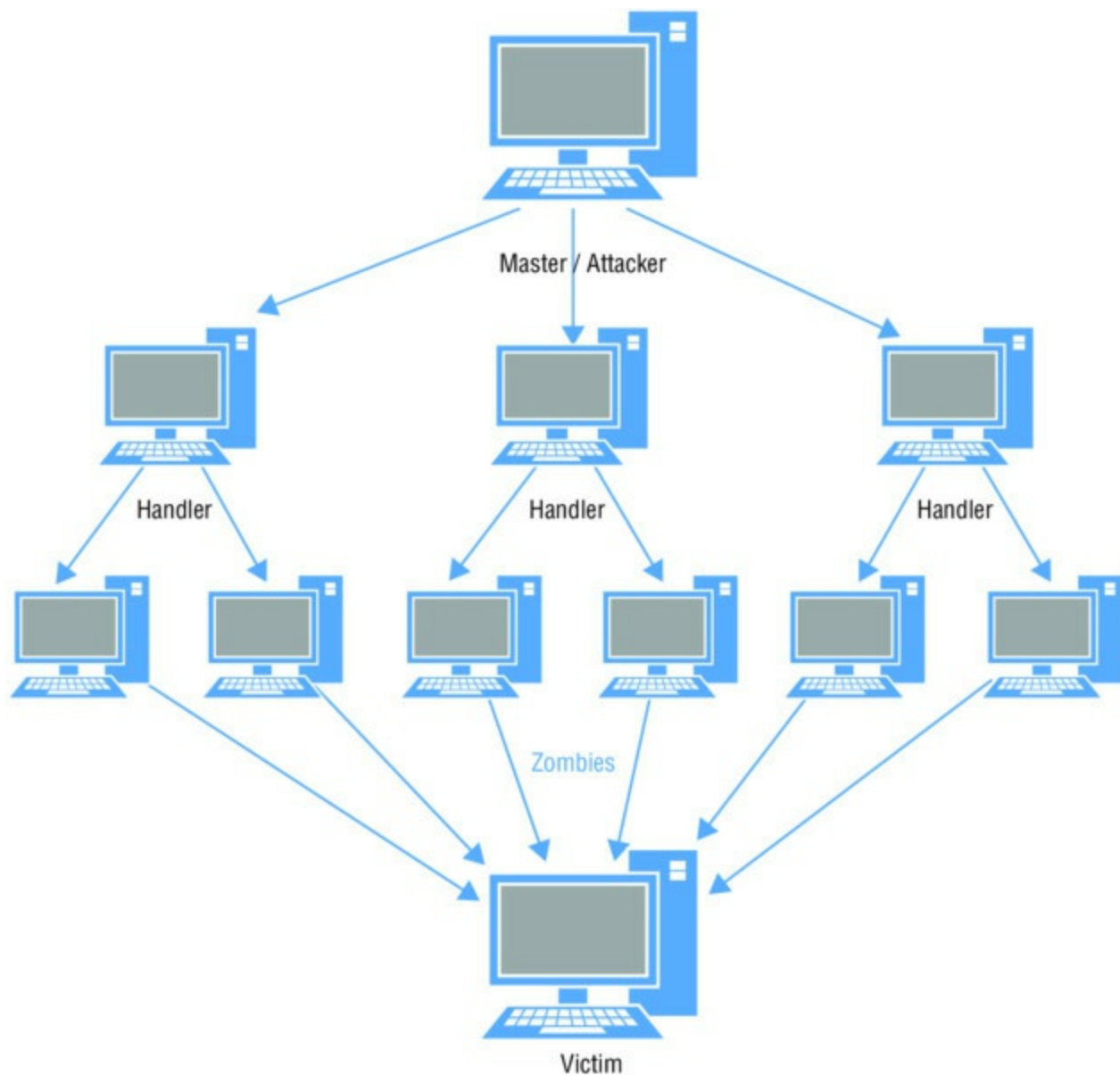
Figure 11.3 DDoS attack setup
