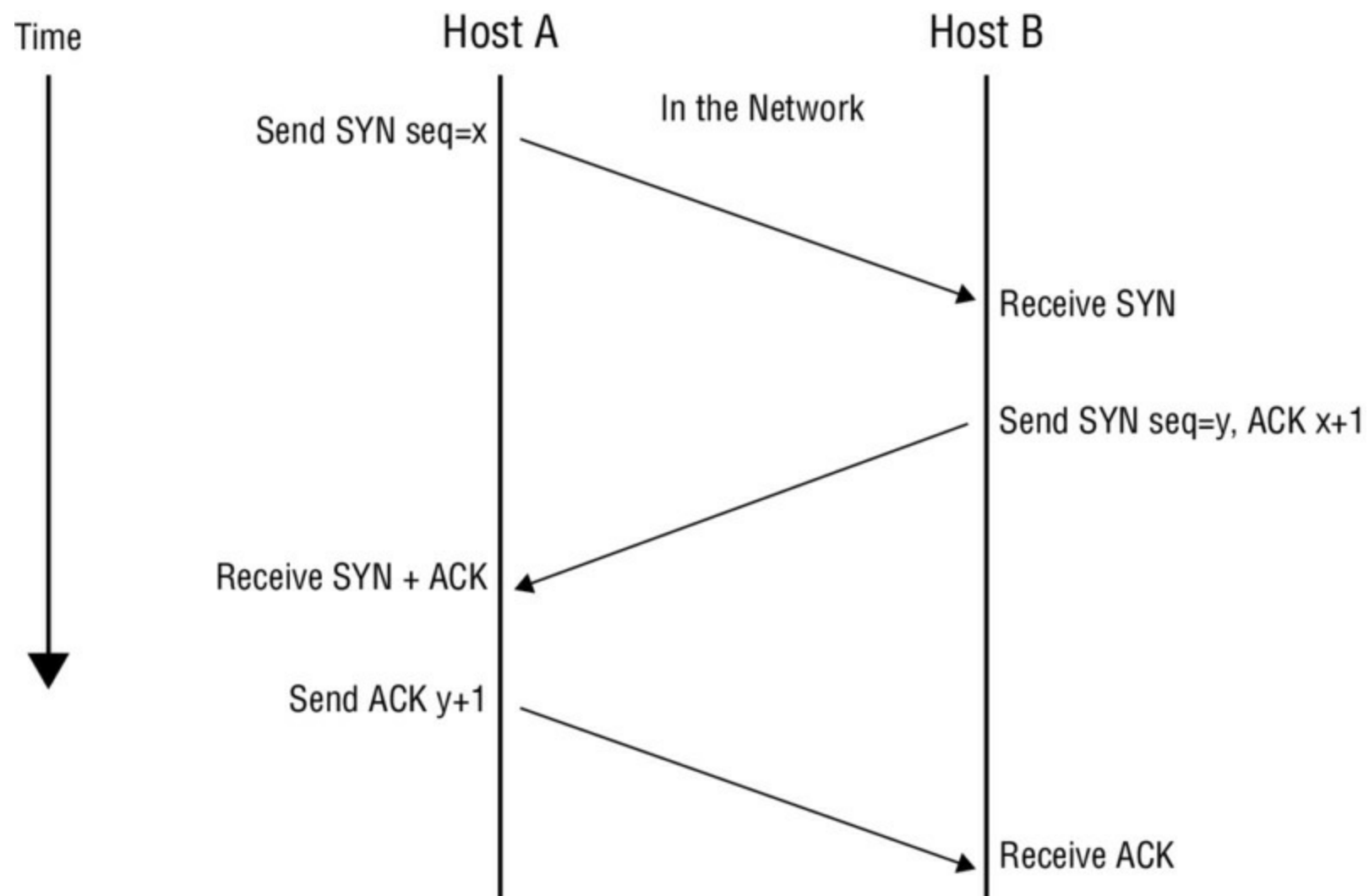
Figure 5.1 The three-way handshake
