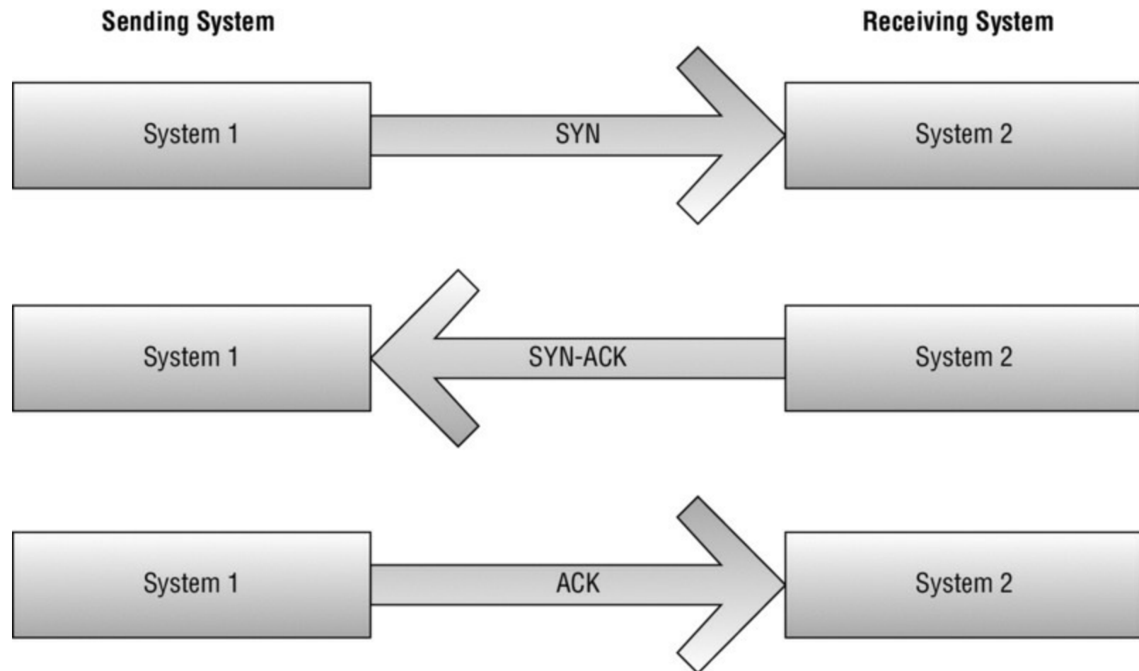
Figure 12.7 TCP three-way handshake
