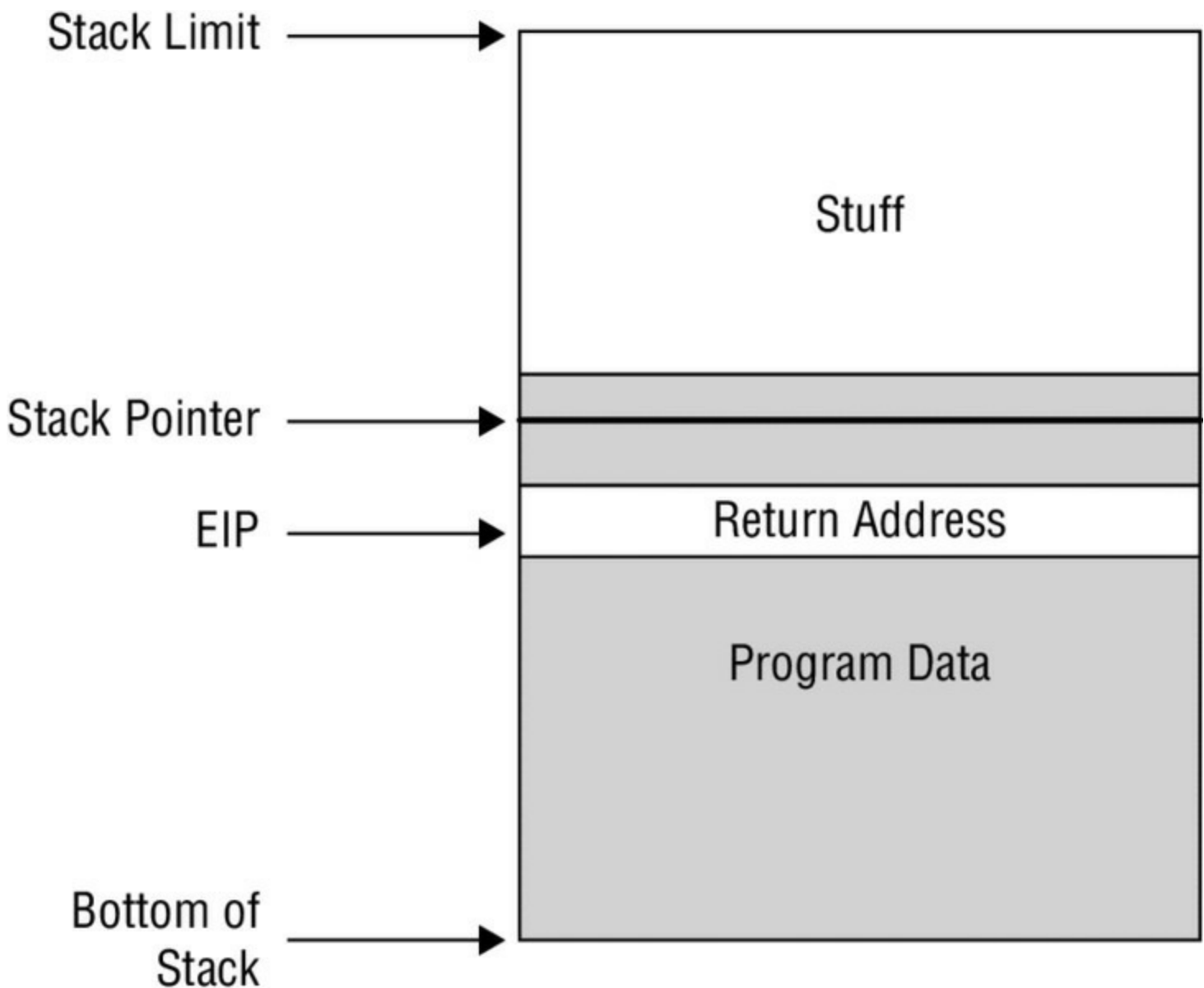
Figure 11.1 Basic program stack
