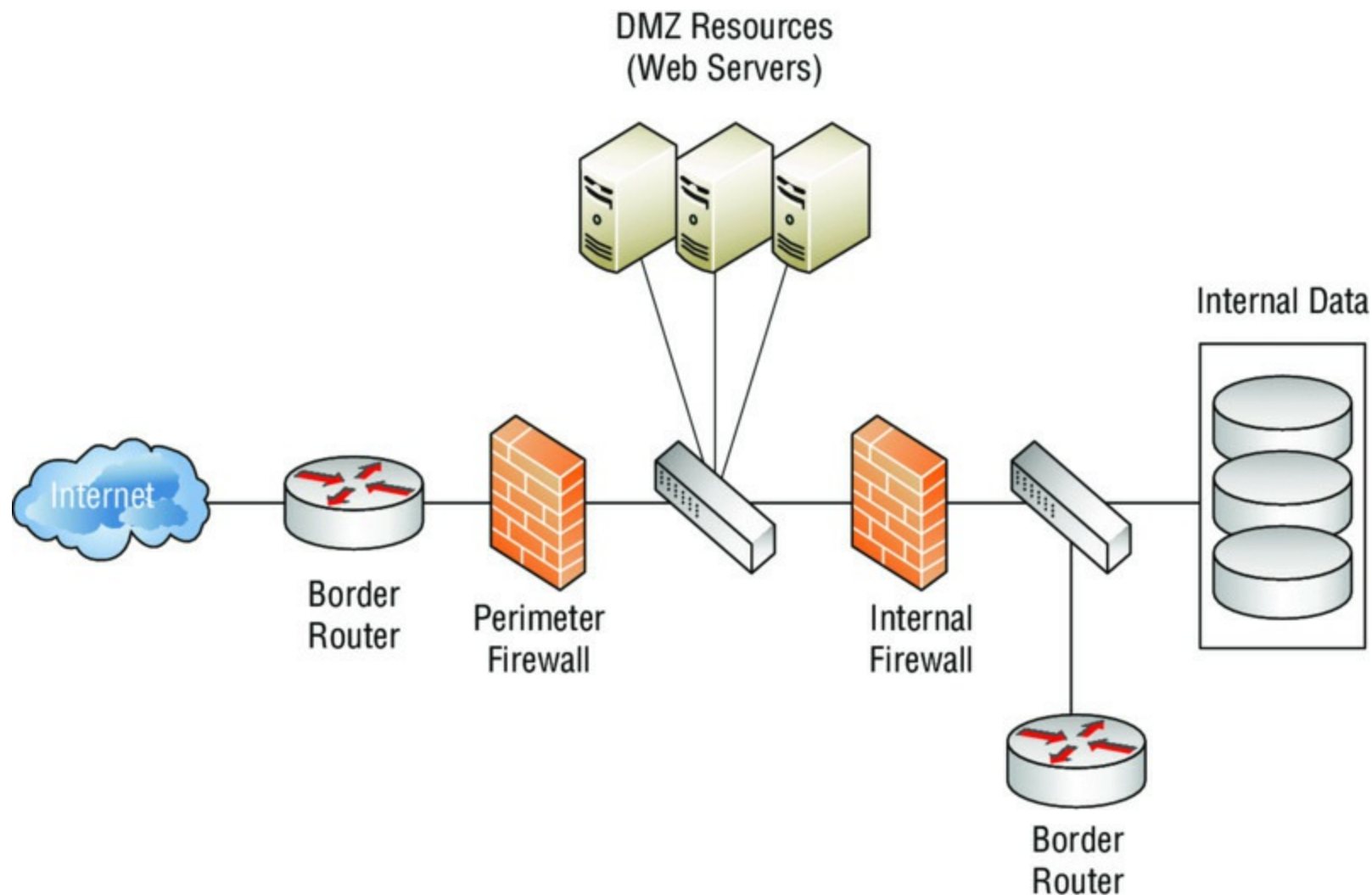
Figure 2.10 Typical enterprise network
