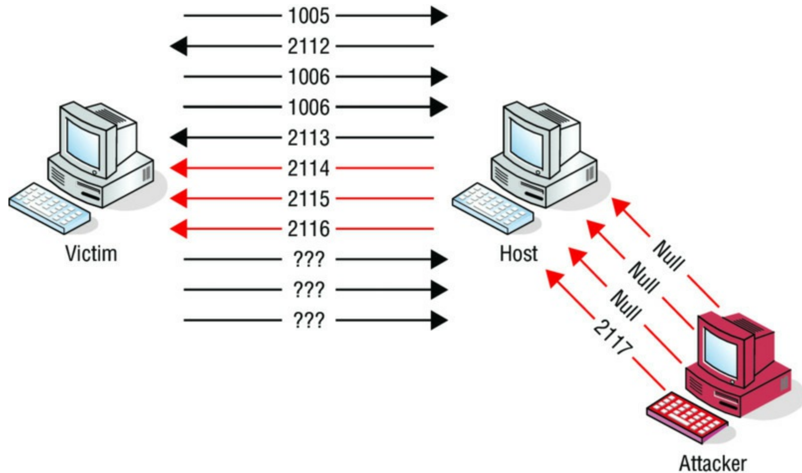
Figure 12.6 Desynchronizing a connection
