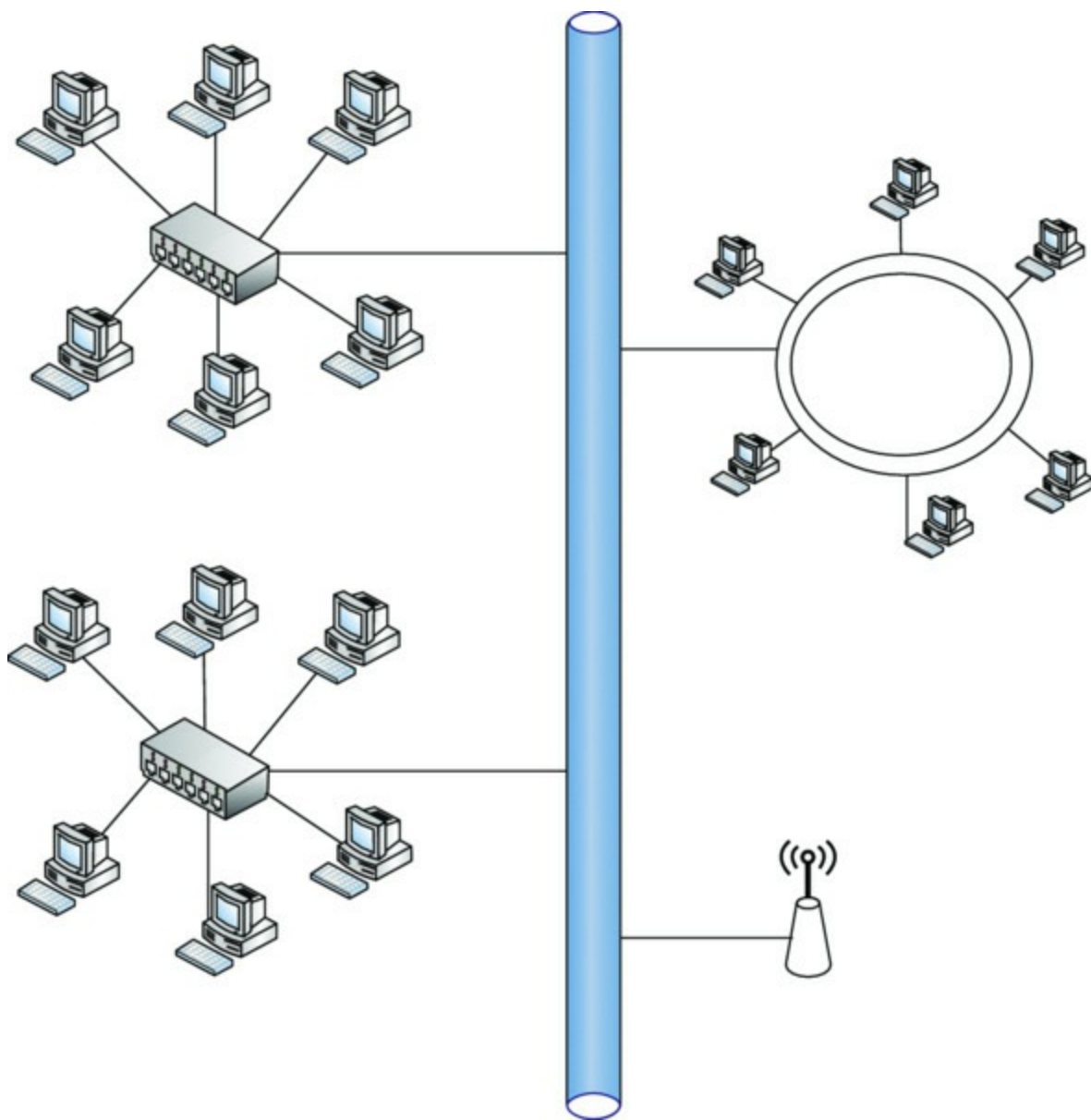
Figure 2.5 Hybrid topology
