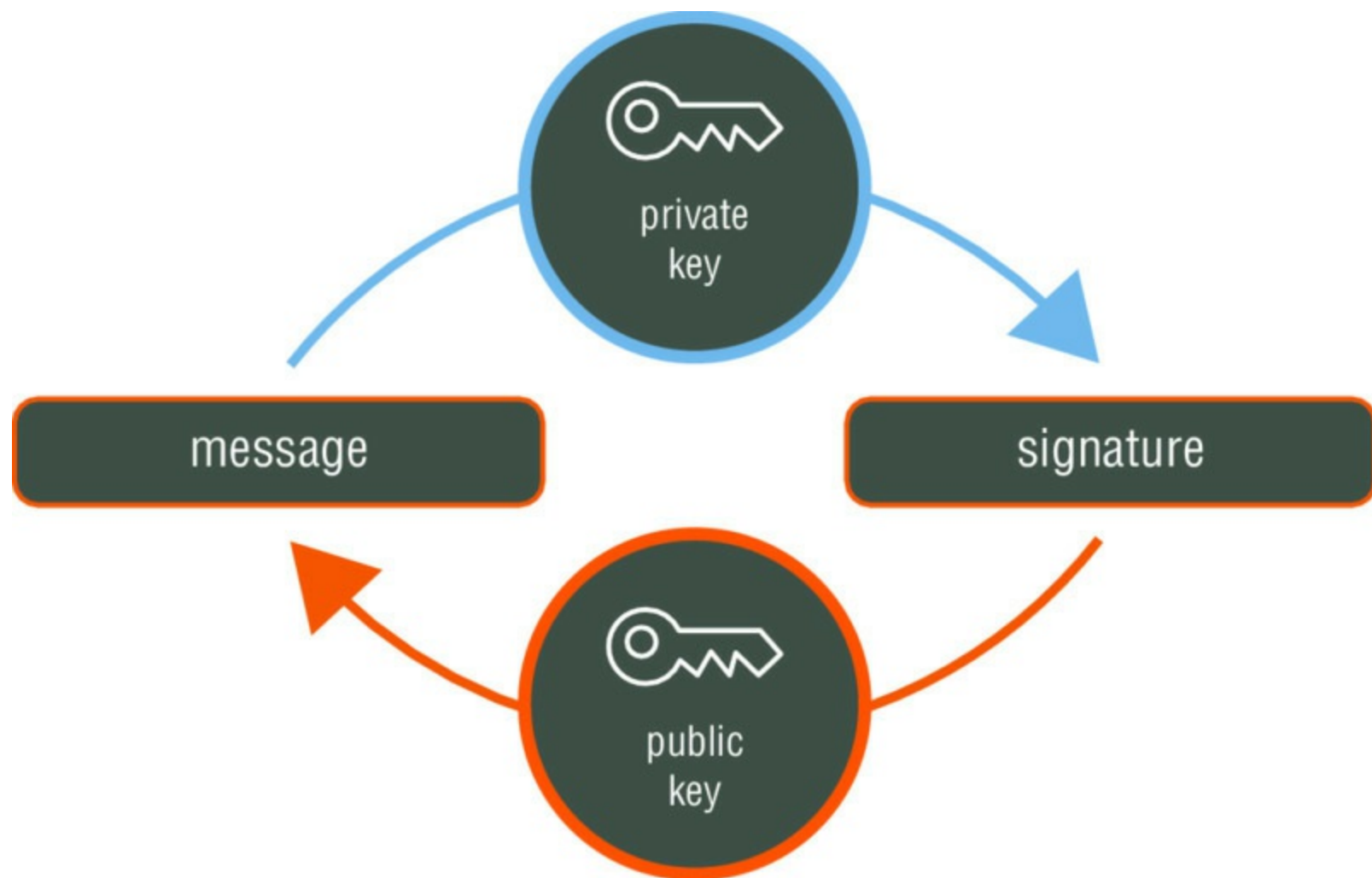
Figure 3.4 A digital signature in use
