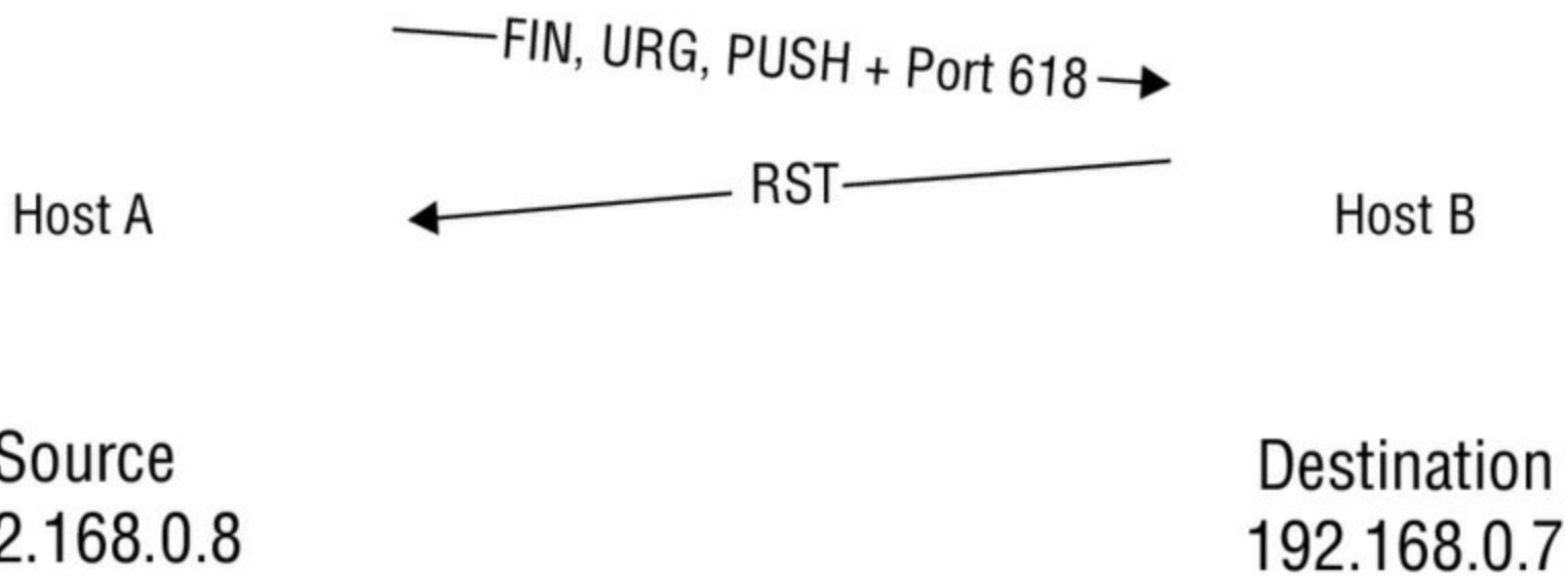
Figure 5.3 Xmas tree scan
