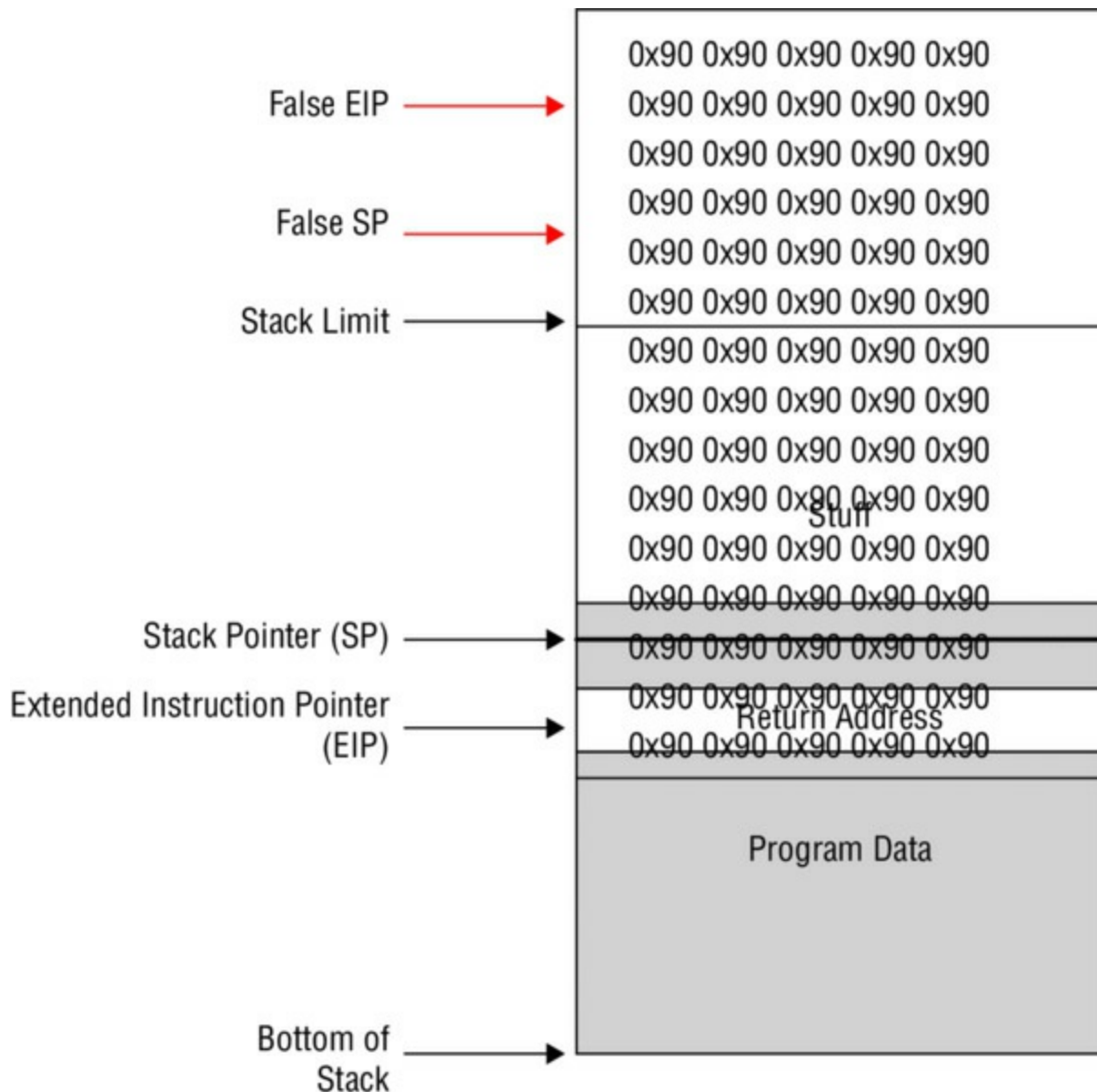
Figure 11.2 Smashing the stack
