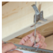
2 Suspend main beams with hanger wire or NEW QuickHang™ hardware* (shown above: QuickHang hooks and brackets)
