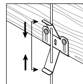
4 Level grid by squeezing tabs & moving hook up or down
