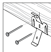
1 Attach bracket to joist using hammer tabs & nails*
