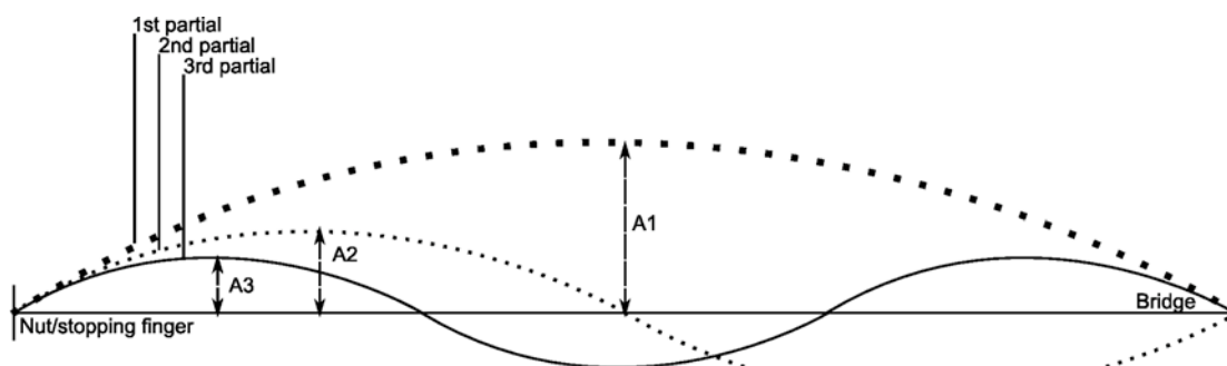
Figure B1c The amplitude of the first three partials in an ideal string.
