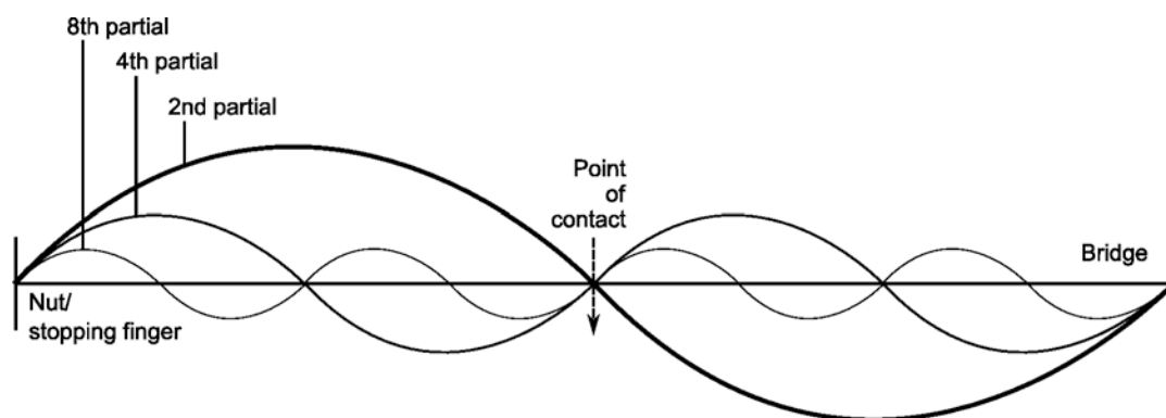
Figure A1.2e A contact point at a node of the 2 nd , 4 th and 8 th partials.
