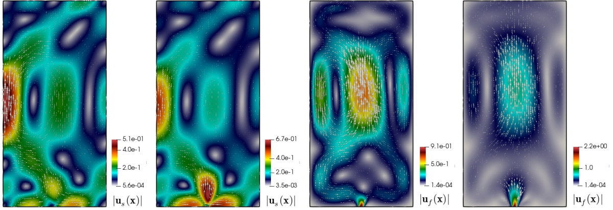
Figure 6.3: Example 2. From left to right: Magnitudes of the particle and fluid velocities for two different magnitudes of the inlet fluid velocity.
