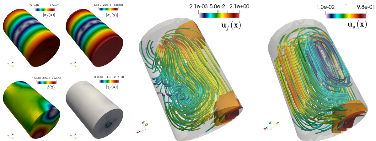
Figure 6.4: Example 3. Magnitude of fluid and particle pseudostress (left top), particle distribution and magnitude fluid vorticity (left bottom), and fluid (center) and particle (right) velocity streamlines showing also contour plots of the particle distribution. The simulations were performed with the lowest-order PEERS ℓ method.
