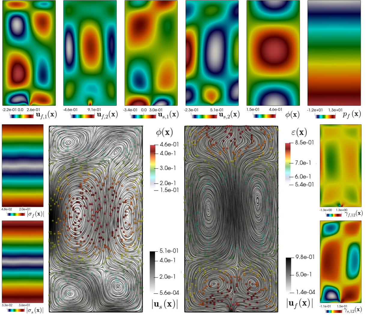
Figure 6.2: Example 2. Approximate solutions obtained with a lowest-order \text{AFW}_\ell method. Velocity components and postprocessed pressure (top), magnitude of fluid and particle pseudostress (bottom left), synthetic particle distribution with particle velocity line integral contours and sample of distribution of \varepsilon and fluid velocity (bottom center panels), and entry (1,2) of the fluid and particle vorticity fields.
