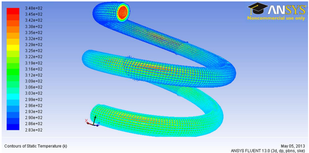
Figure 10 Contours of Static Temperature in K
