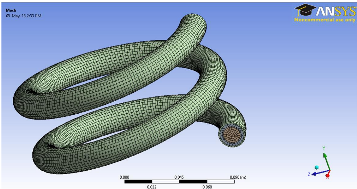
Figure 5 Mesh
