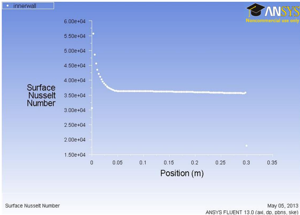
Figure 23 Surface Nusselt Number Plot for Inner-wall
