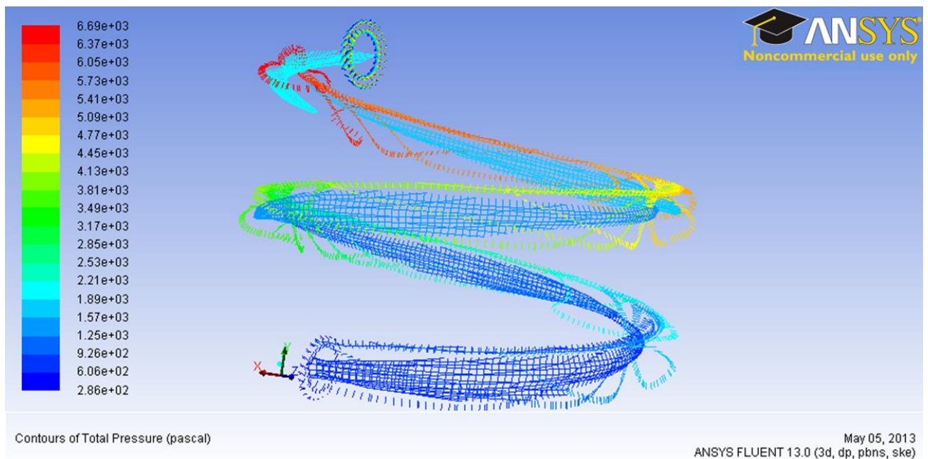
Figure 9 Contours of Total Pressure in Pascal
