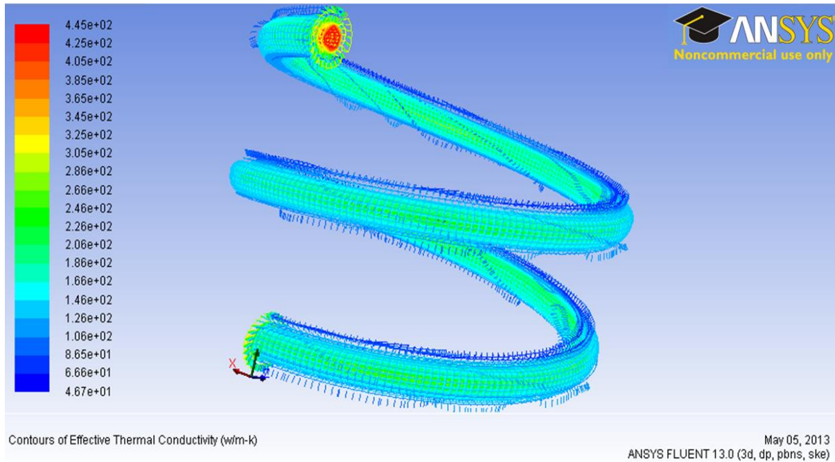
Figure 13 Contours of Effective Thermal Conductivity (w/m-K)
