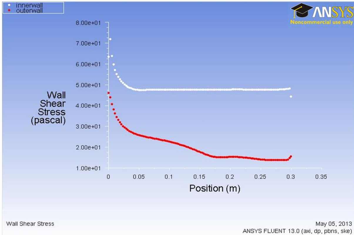
Figure 21 Wall Shear Stress Plot for Inner-wall And Outer-wall
