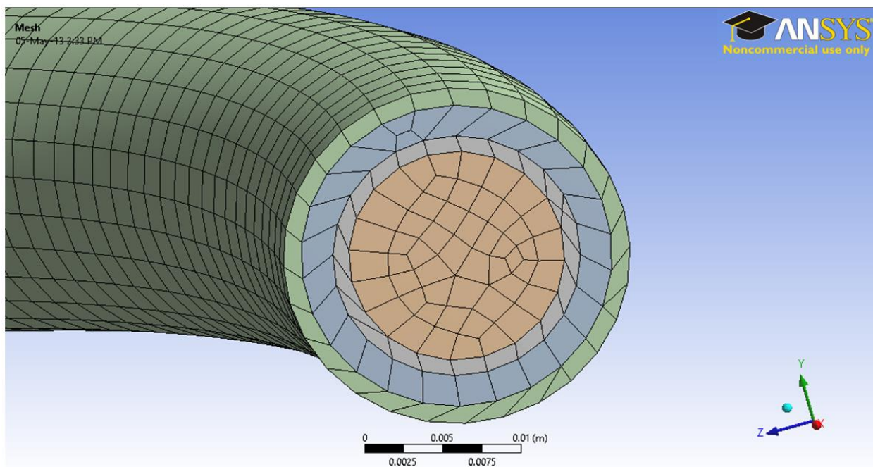
Figure 6 Close View of the Meshed Parts
