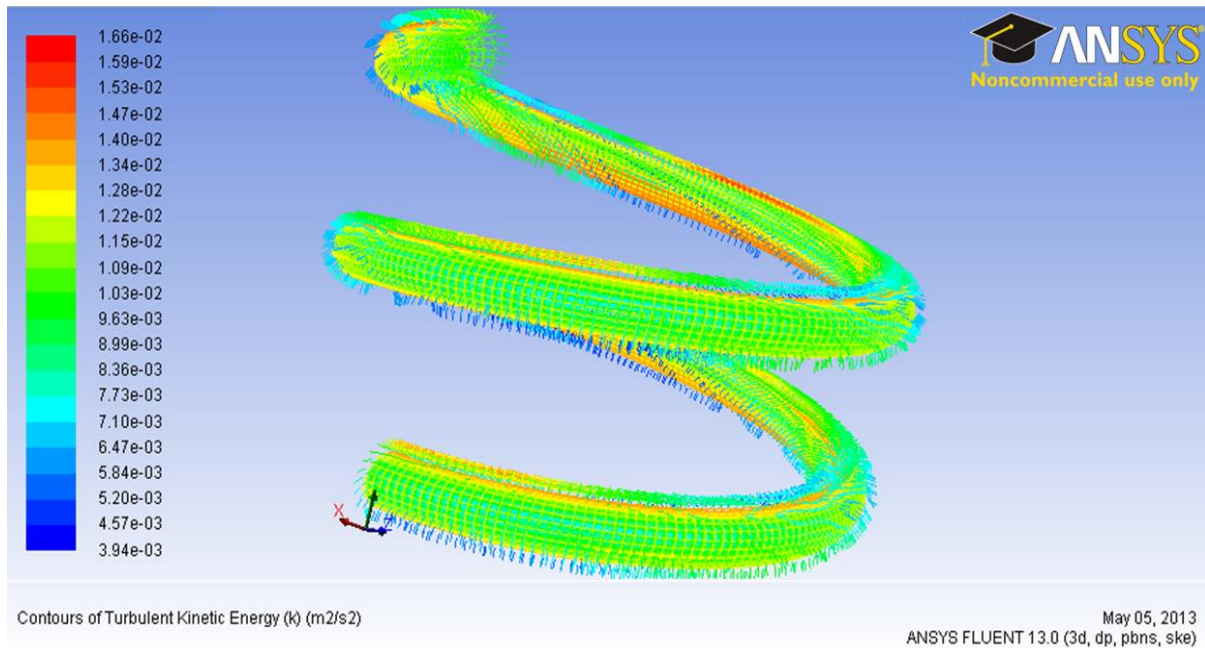
Figure 12 Contours of Turbulent Kinetic Energy k (m 2 /s 2 )
