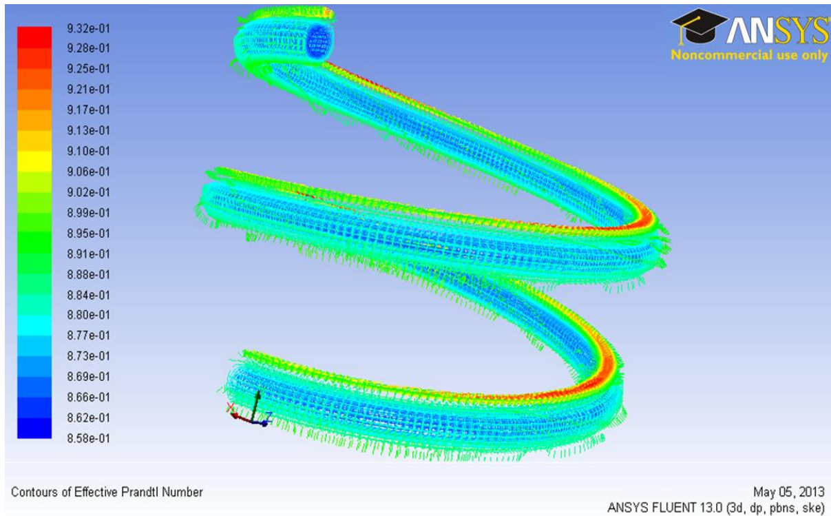
Figure 16 Contours of Effective Prandtl Number
