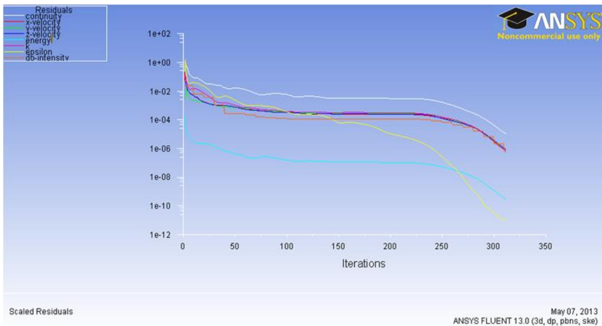
Figure 20 Scaled Residuals
