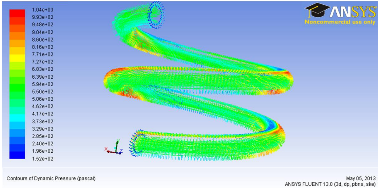
Figure 8 Contours of Dynamic Pressure in Pascal
