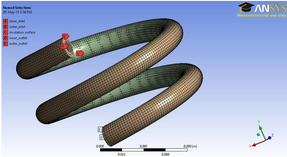
Figure 7 Named Selection
