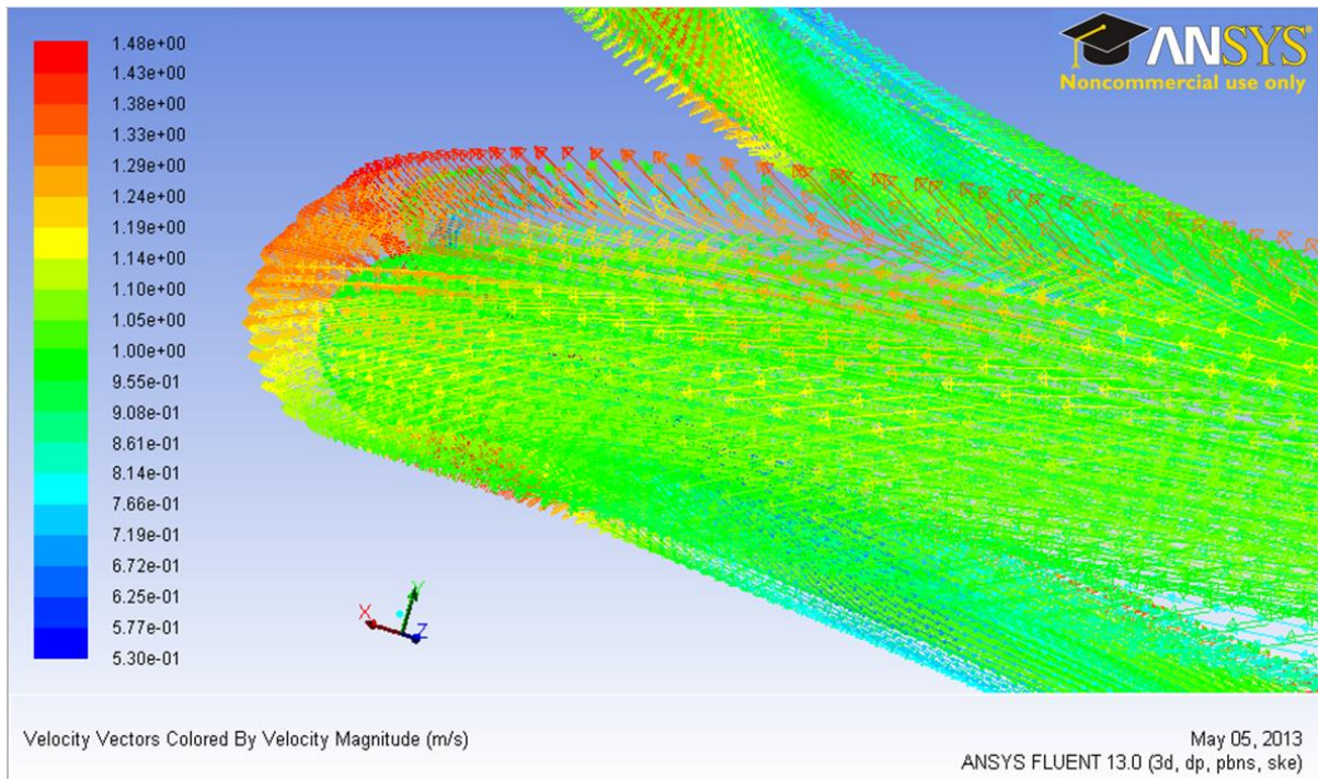
Figure 18 Close View of Velocity Vectors Colored by Velocity Magnitude (m/s)
