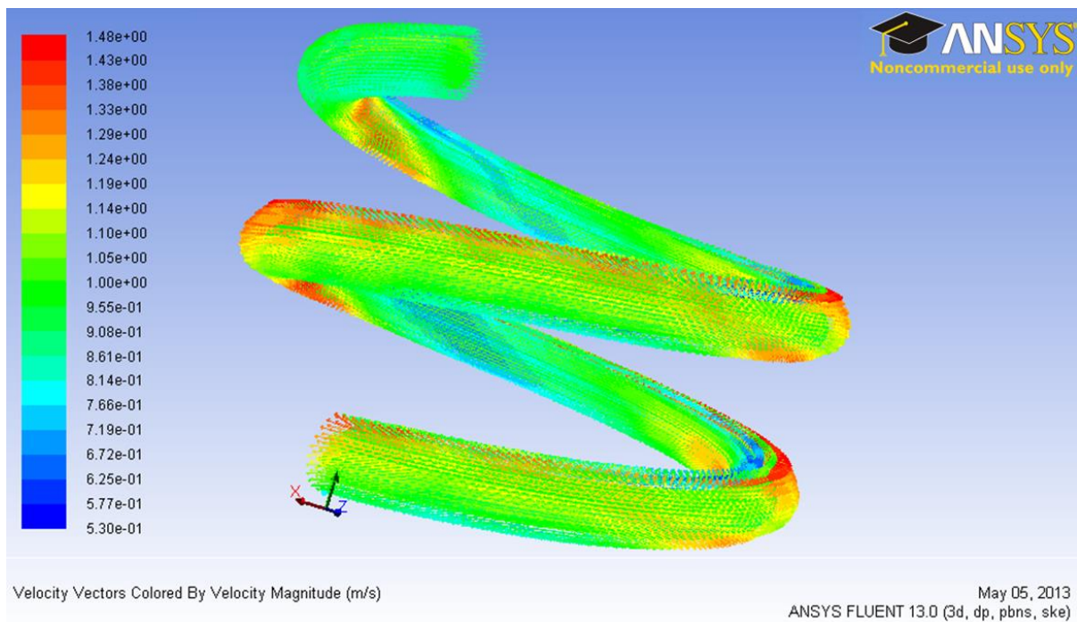
Figure 17 Velocity Vectors Colored by Velocity Magnitude (m/s)
