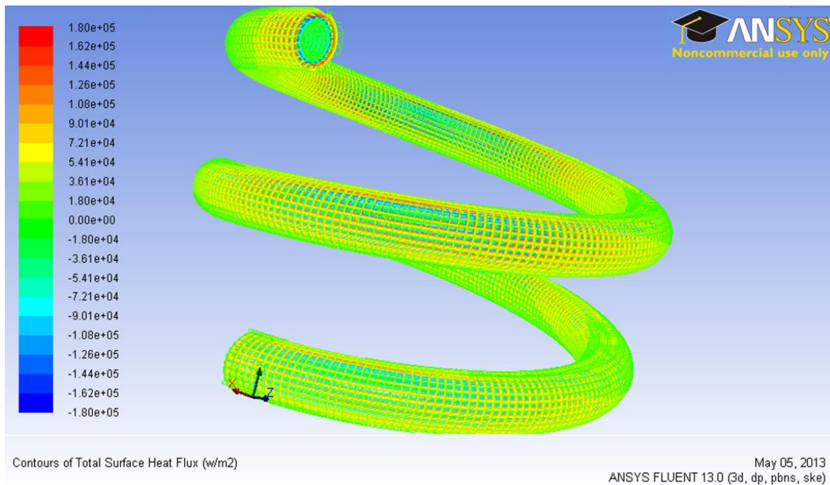
Figure 14 Contours of Total Surface Heat Flux (w/m 2 )
