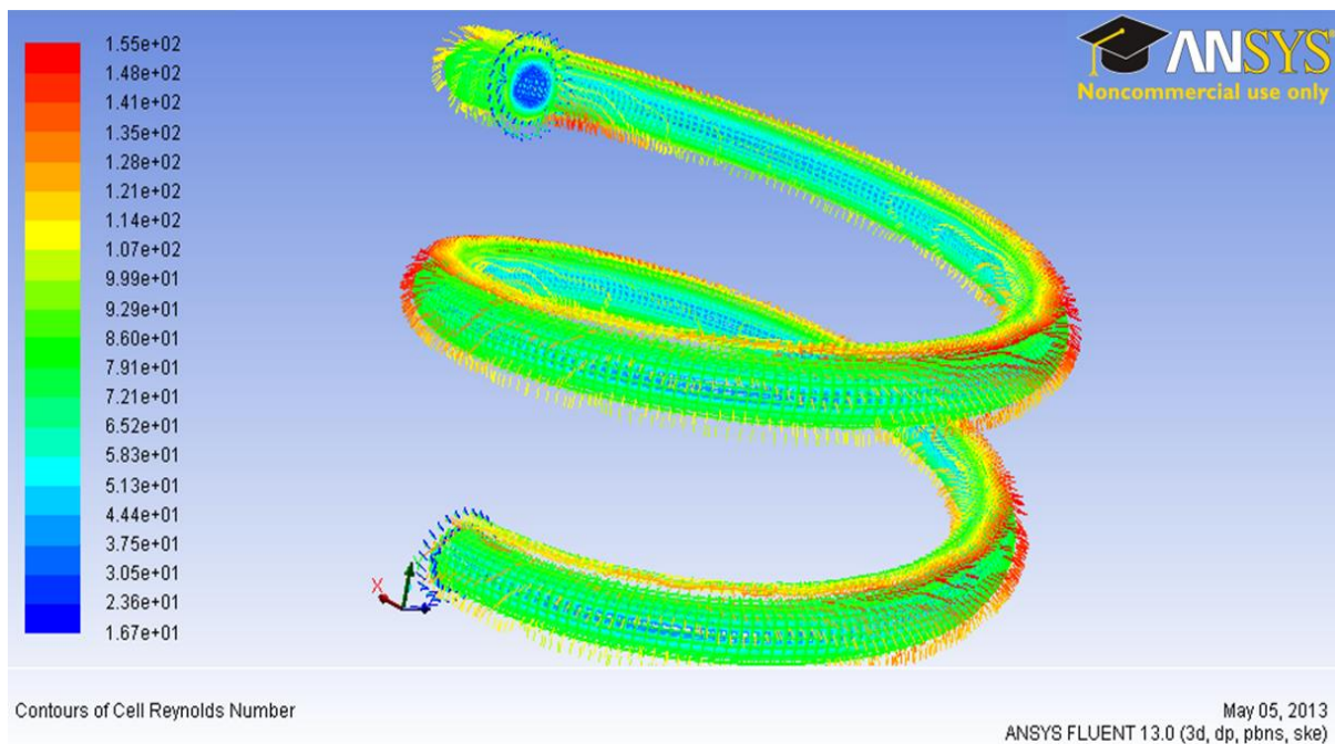
Figure 15 Contours of Cell Reynolds Number
