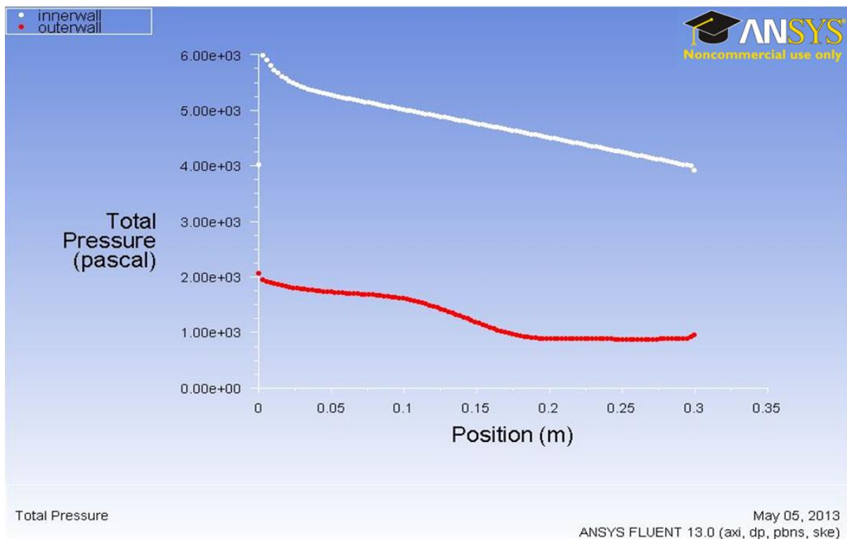
Figure 22 Total Pressure Plot for Innerwall And Outerwall
