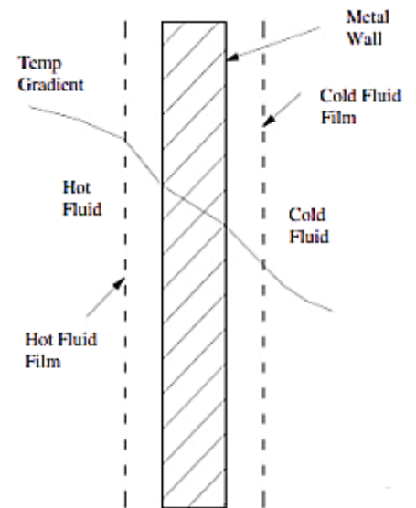
Figure 2 Wall Convection
