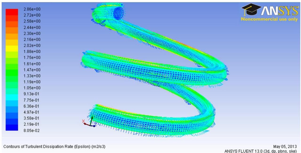
Figure 11 Contours of Turbulent Dissipation Rate (Epsilon) ( m^2/s^3 )
