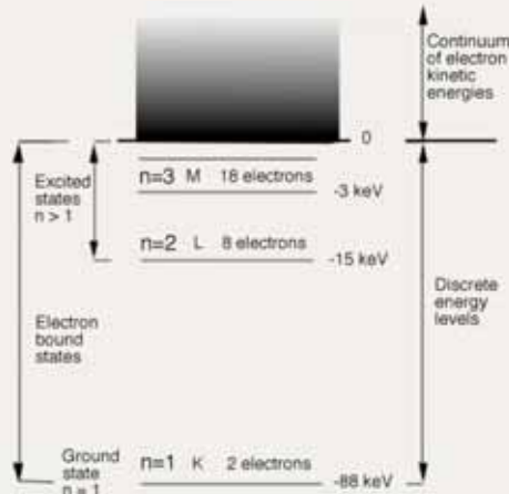
Energy level diagram for multi-electron atom (lead)
