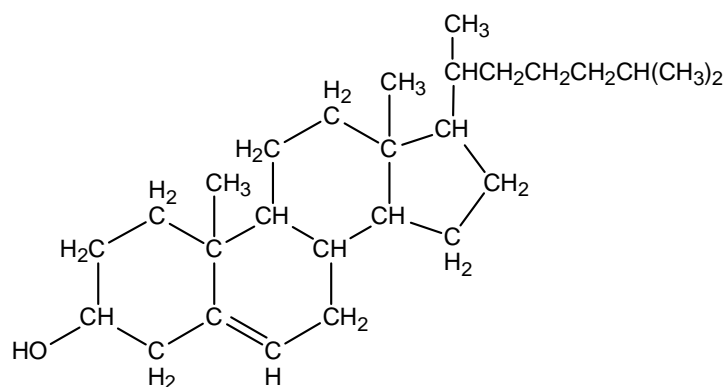
Condensed Structure
