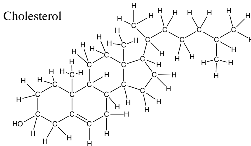
Expanded Structural Formula
