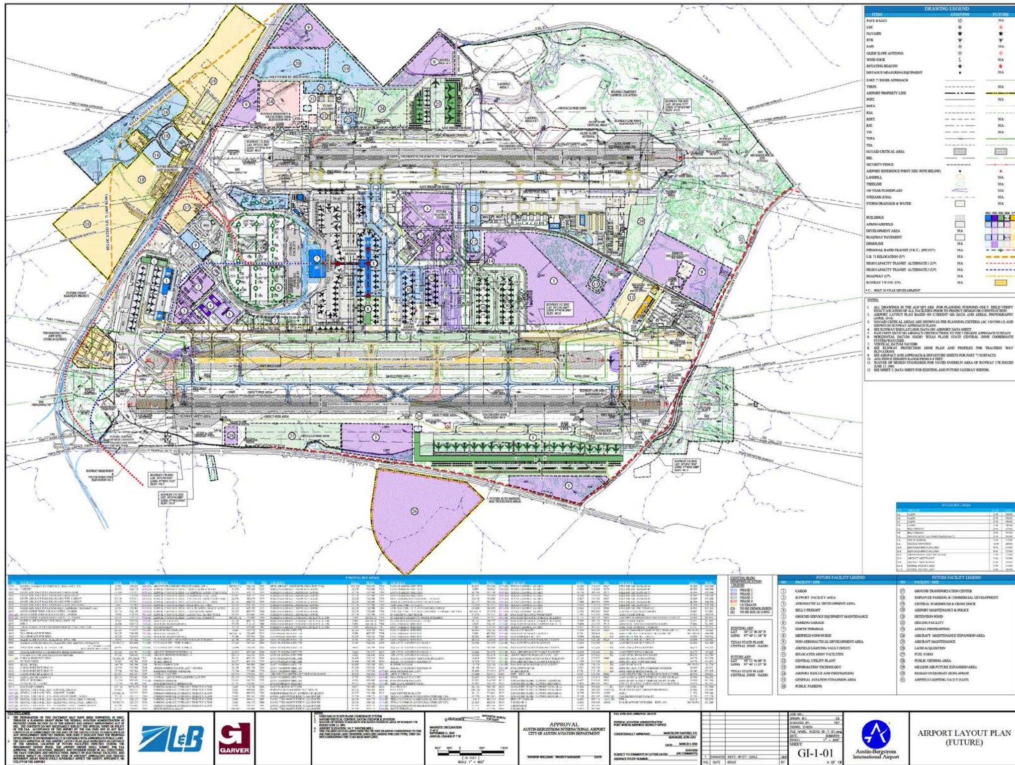
Exhibit 10.2-4: Airport Layout Plan – Future
