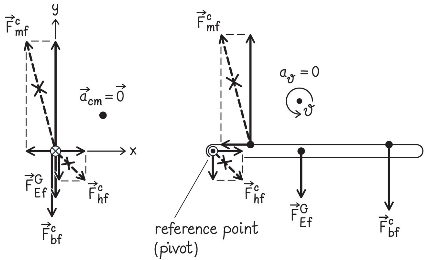
(a) Free-body diagram
