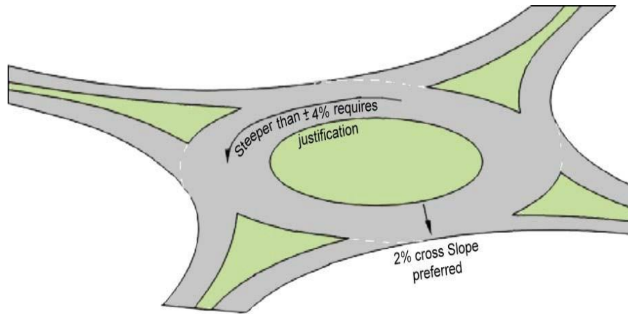
Preferred grades and cross slopes
