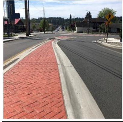
Roundabout showing red concrete with brick texturing for the splitter island and central island, and river rock buffer between the roadway and sidewalk. Location is West Alder St at 1 st St in Shelton, WA
