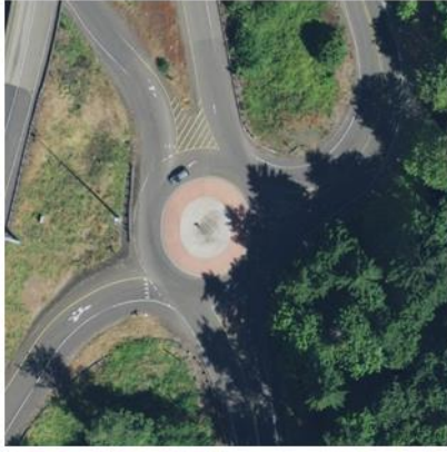
Roundabout showing two-color mountable central island. Location is State Route 432 at Exit 36 on Interstate 5 in Kelso, WA
