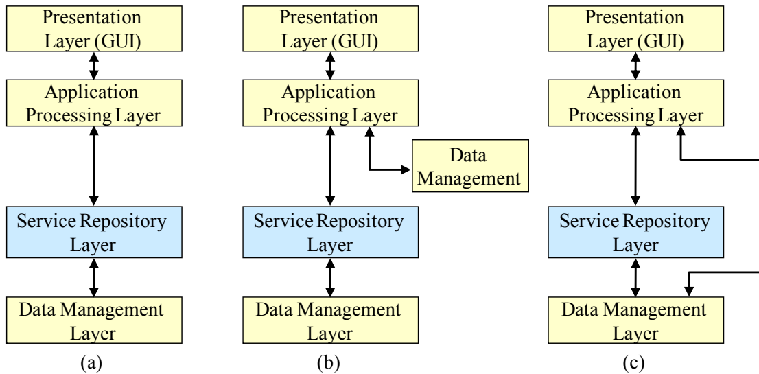
Figure 1.6 Four-tier architecture and its variations
