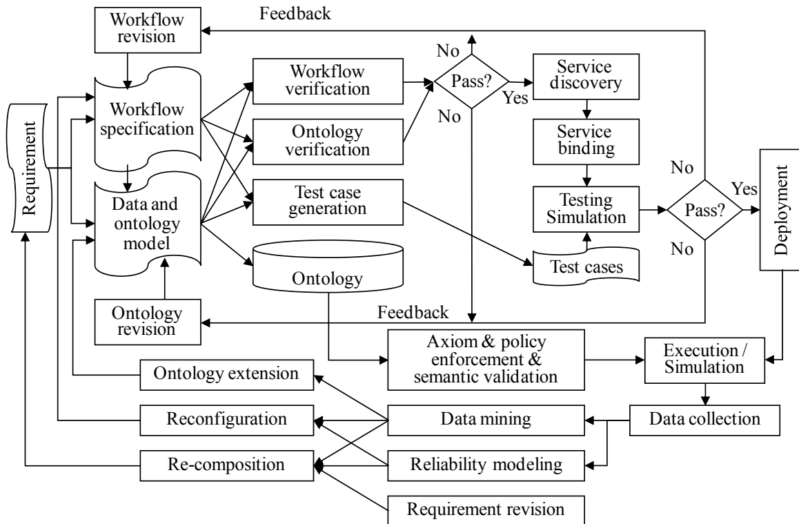
Figure 1.15 Service-oriented application development process
