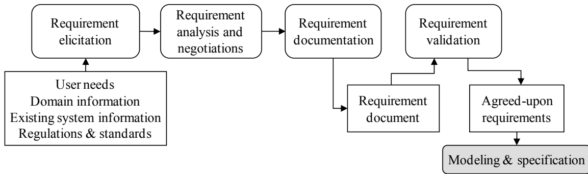
Figure 1.14 Requirement development process
