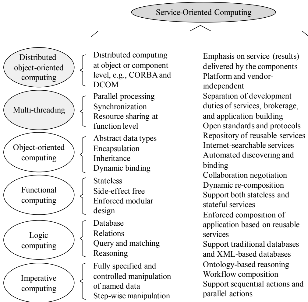
Figure 1.2 Features of different computing paradigms
