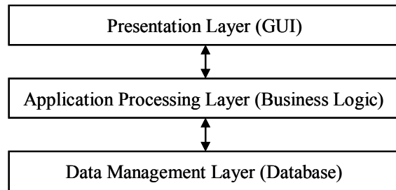
Figure 1.4 Three-tier architecture
