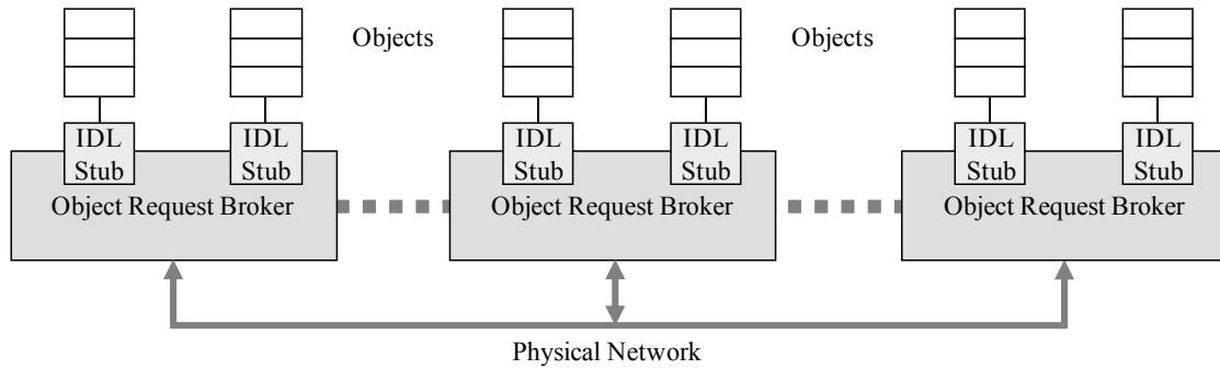
Figure 1.7 CORBA architecture
