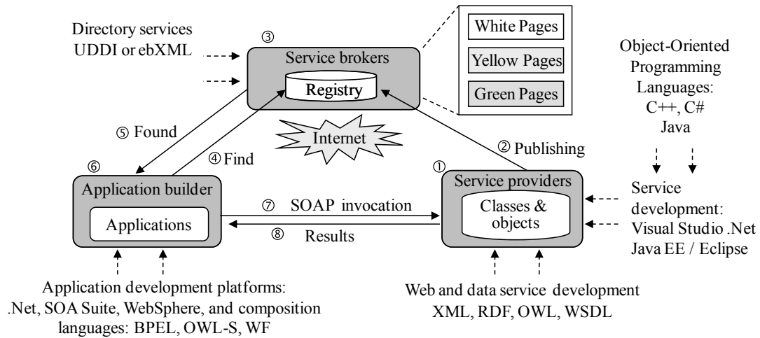
Figure 1.9 A typical service-oriented architecture
