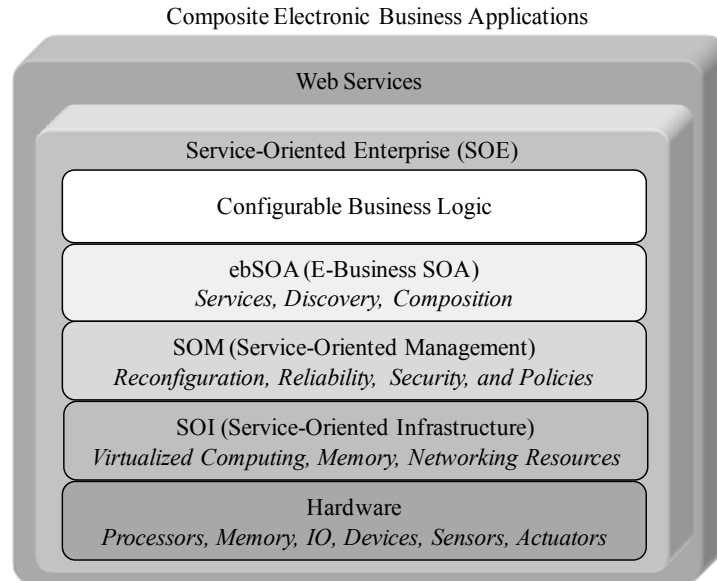
Figure 1.11 SOE framework
