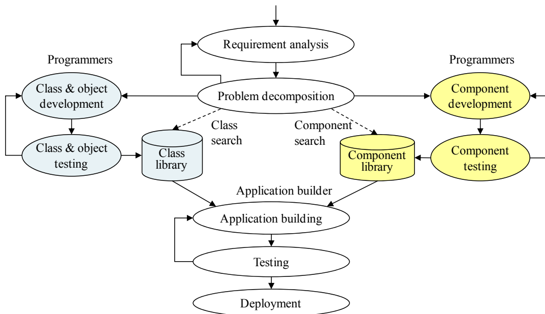
Figure 1.12 Object-oriented and component-based software development processes
