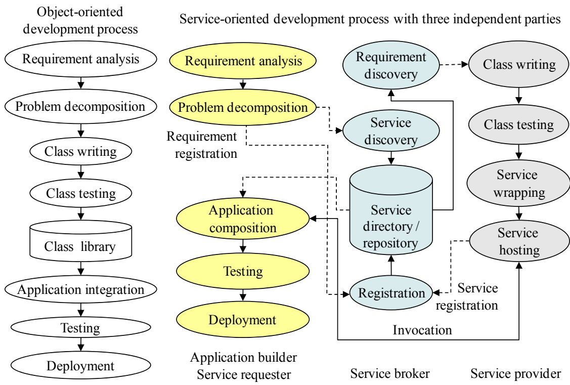
Figure 1.13 Object-oriented versus service-oriented software development process
