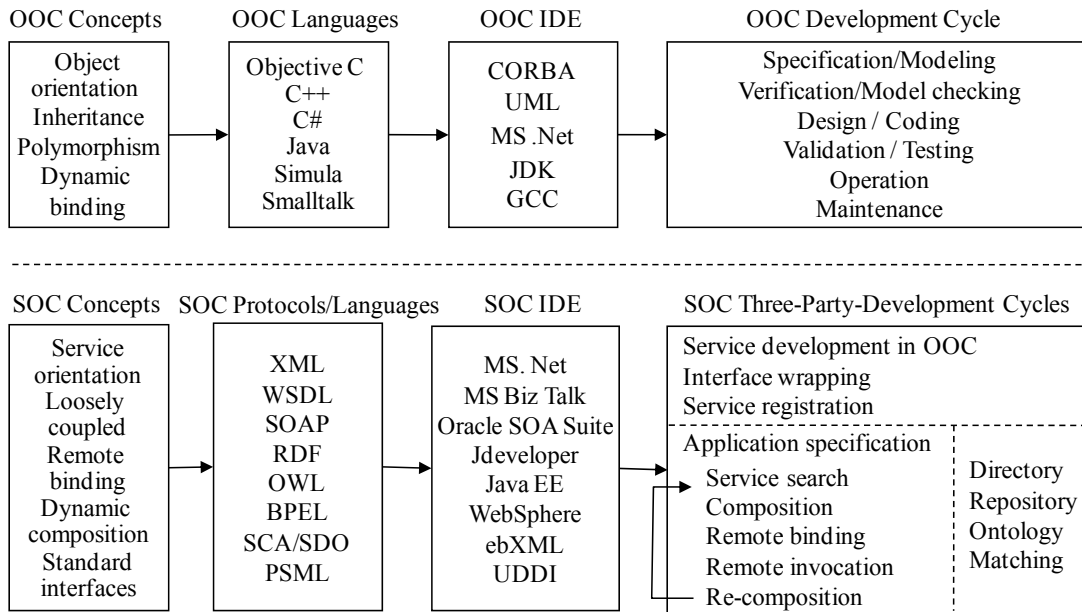
Figure 1.10 OOC and SOC concepts and technologies
