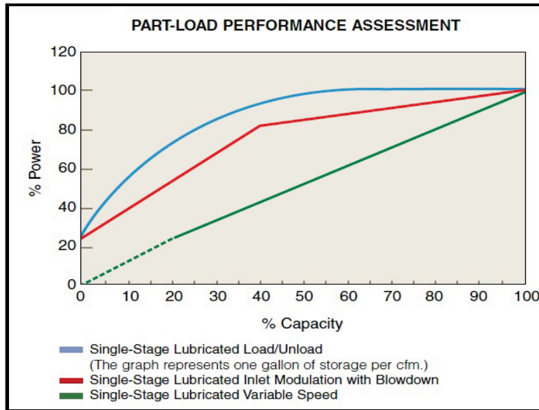
Figure 1. Example operation curve (% power versus % capacity curve) for lubricated rotary screw air compressor
