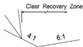
Preferred Side Gutter Section if Within CRZ
