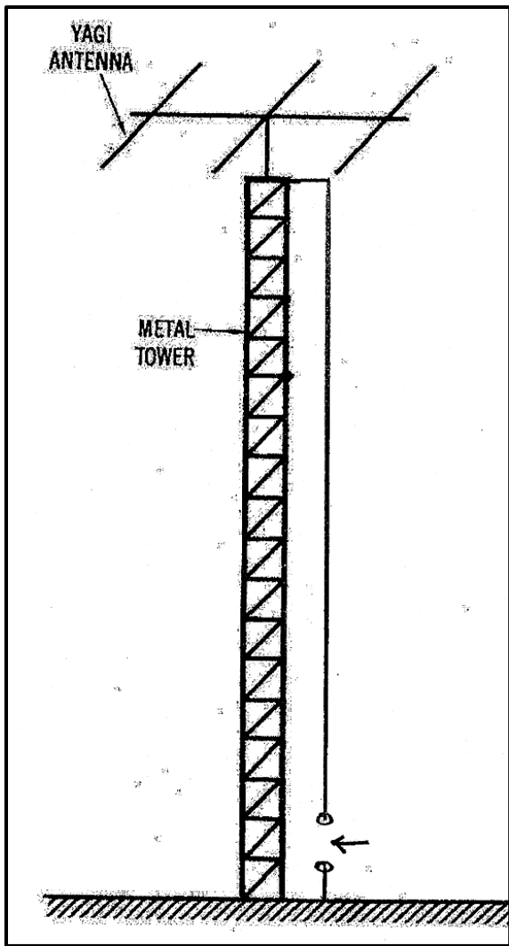
Figure 4.10 - Shunt fed tower.
