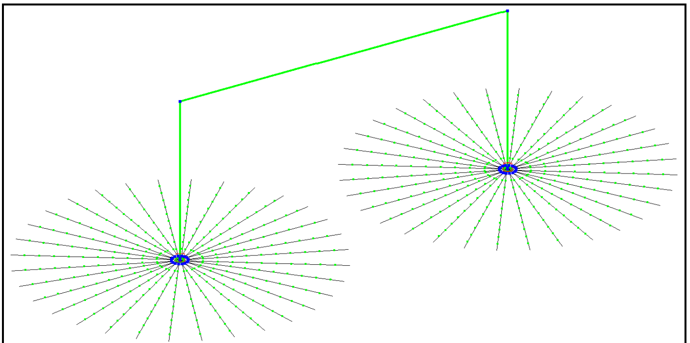
Figure 4.23 - Antenna with two downleads and a loading inductor at the base of each downlead.
