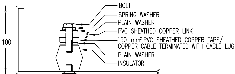
Sectional Elevation A-A'
