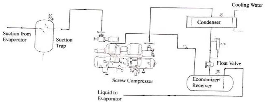
FIG. 6.7 Screw Compressor with Economizer/Receiver
