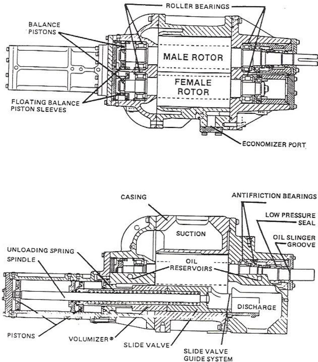
FIG. 6.1 Typical Twin-Rotor Screw Compressor Construction
