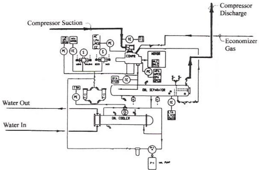
FIG. 6.15 Screw Compressor with Water Cooled Oil Cooler
