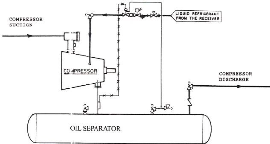
FIG. 6.16 Liquid Injection Oil Cooling
