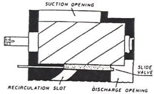
HIGH FIXED V_i COMPRESSOR Long Slide Valve
