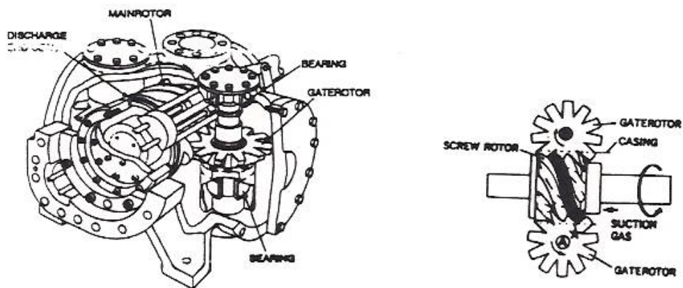
FIG. 6.3 Typical Single-Rotor Screw Construction
