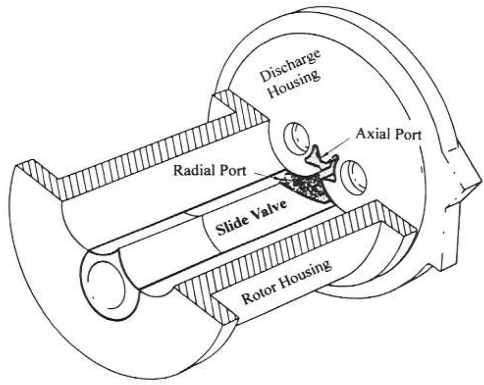
Screw Compressor Slide Valve
