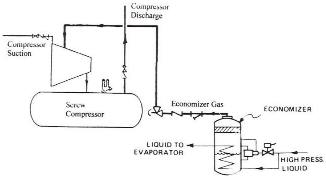
FIG. 6.9 Screw Compressor with Shell-and-Coil Liquid Subcooling Economizer
