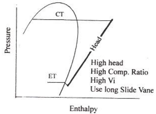
FIG. 6.21 Internal Volume Ratio ( V_i ) & Slide Vane
