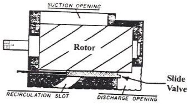
Screw Compressor Slide Valve
