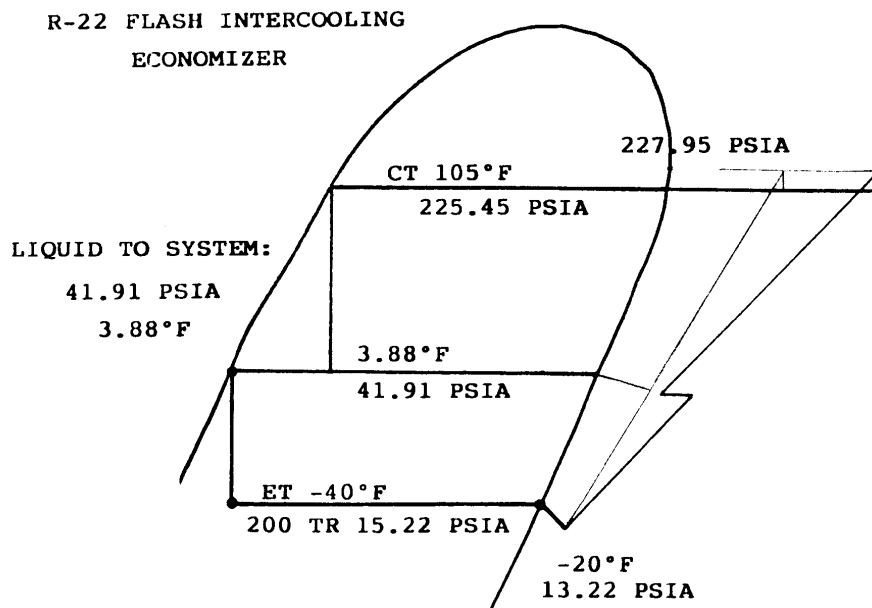
FIG. 6.8 P-H Diagram for Screw with Flash Economizer
