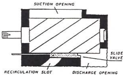
LOW FIXED V_i COMPRESSOR Short Slide Valve
