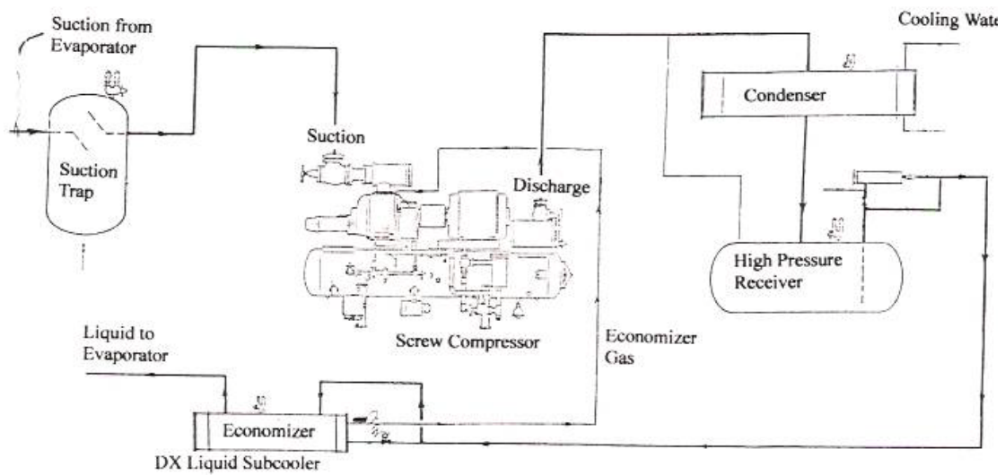
FIG. 6.10 Screw Compressor with DX Liquid Subcooling Economizer
