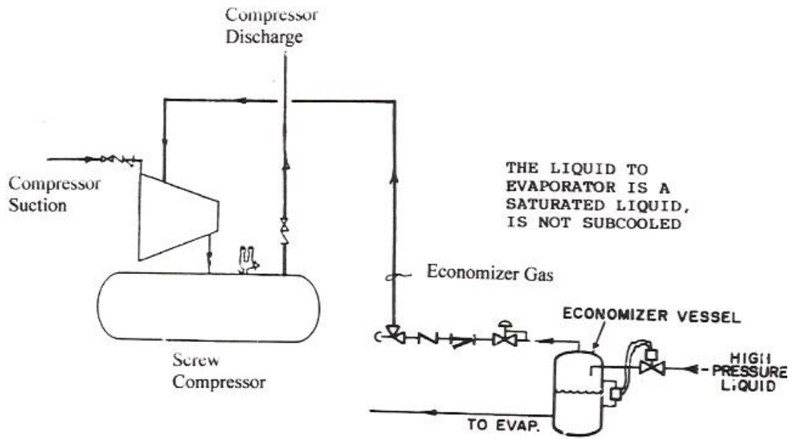
FIG. 6.6 Screw Compressor with Flash Economizer
