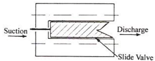
FIXED HIGH V_i Long Slide Valve
