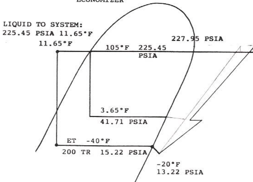
FIG. 6.11 P-H Diagram for Screw with Liquid Subcooling Economizer
