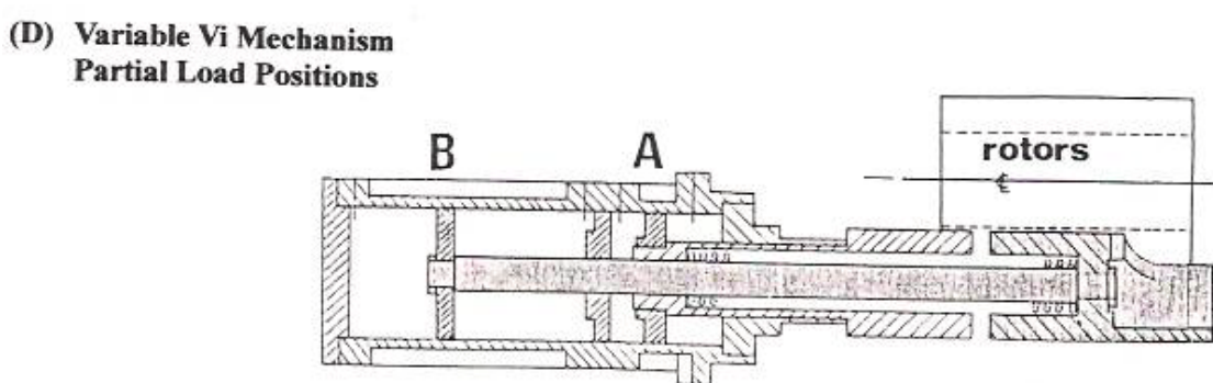
FIG. 6.23 Fixed Vi and Variable Vi Slide Vanes
