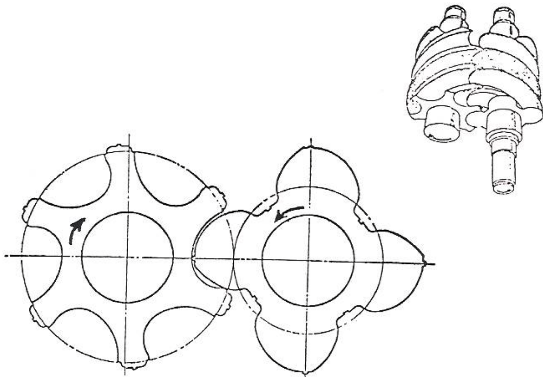
FIG. 6.2 Typical Asymmetric Twin-Rotor Profile
