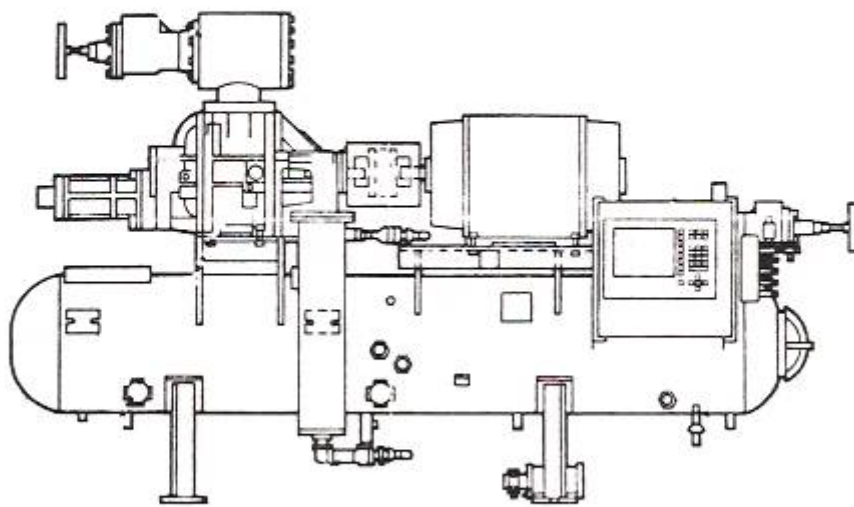
FIG. 6.13 Screw Unit with Horizontal Oil Separator
