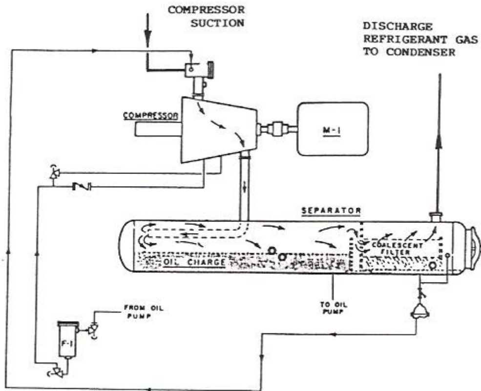
FIG. 6.12 Oil Separator – Screw Compressor Unit
