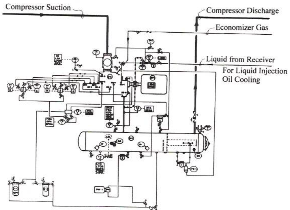
FIG. 6.17 Screw Compressor with Liquid Injection Oil Cooling
