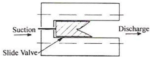
FIXED LOW V_i Short Slide Valve
