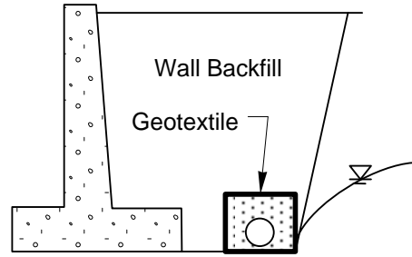
E. Underground Drainage: Low Survivability (Wrapped Drain Behind Foundation)
