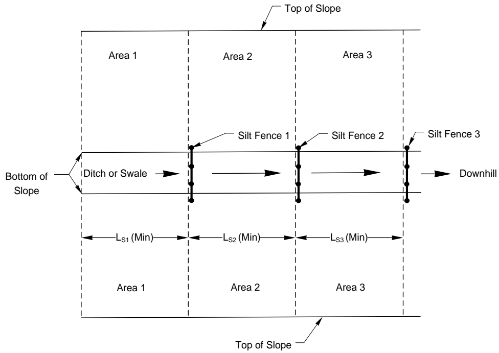
Method to keep contributing area to ditch or swale within allowable limits if contributing area is too large based on Exhibit 630-3.
