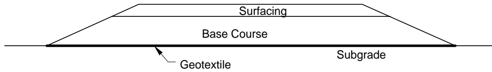
G. Separation or Soil Stabilization for New Roadway (Depends on Subgrade Condition)
