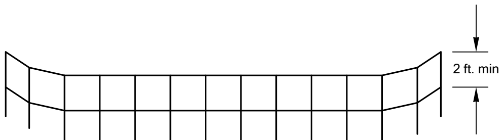
Silt Fence Profile
