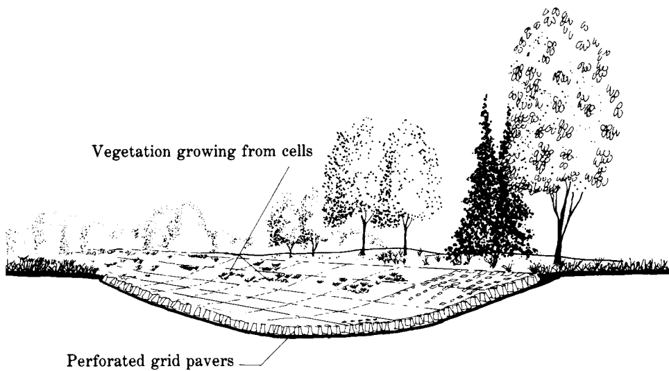
Figure 7-4.—Cross section showing perforated grid pavers.
