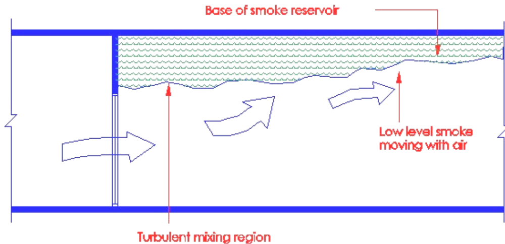
Diagram 7.6.13 - 2
