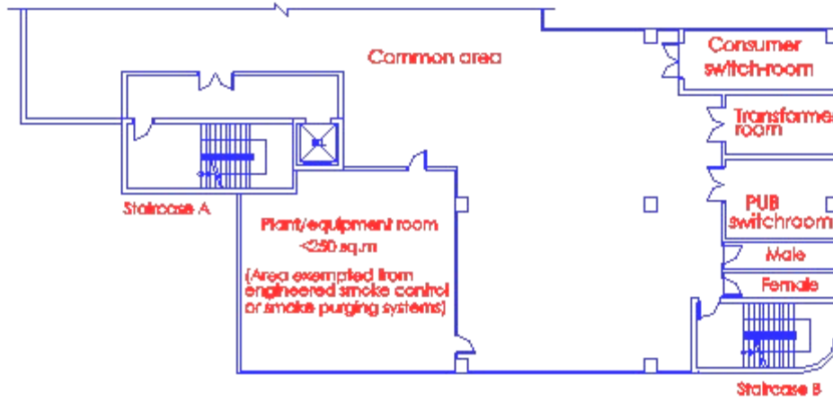
Part plan of basement storey
