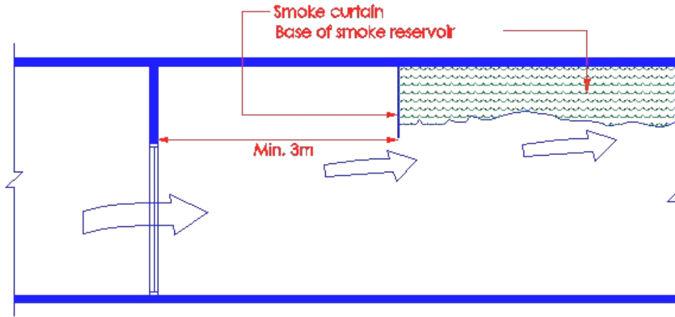
Diagram 7.6.13 - 3
