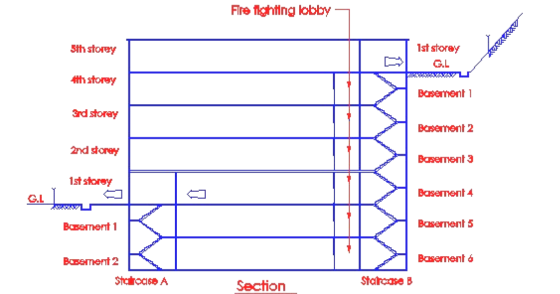
Diagram 7.2.1-5
