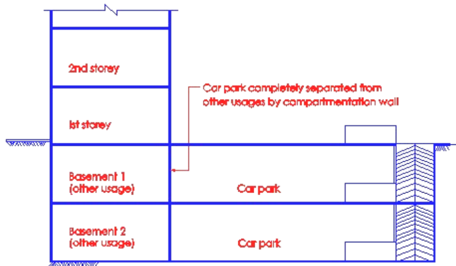
Diagram 7.4.1 (b)(i)
