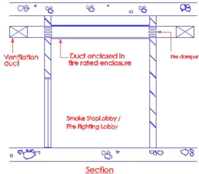
Diagram 7.1.1(e)- 1
