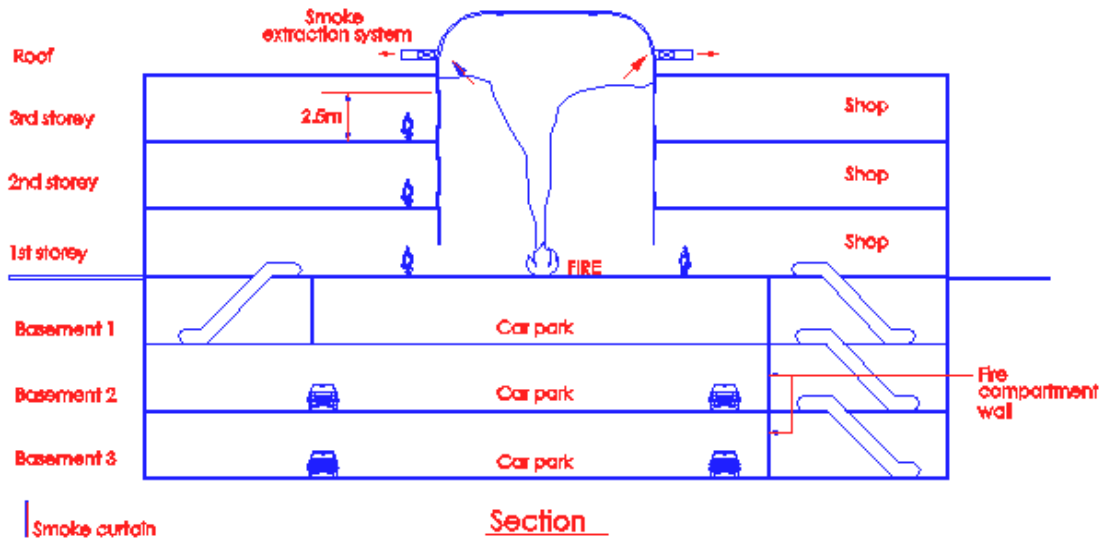
Diagram 7.6.4 - 1
