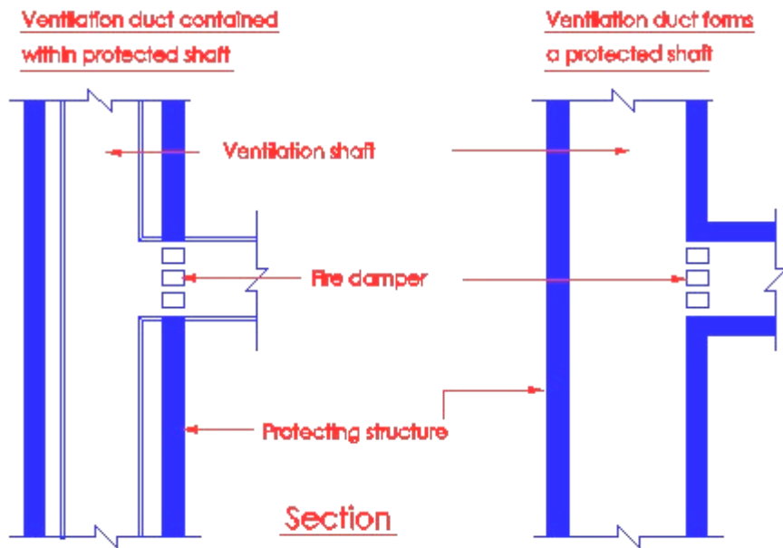
Diagram 7.1.1(i) - 2
