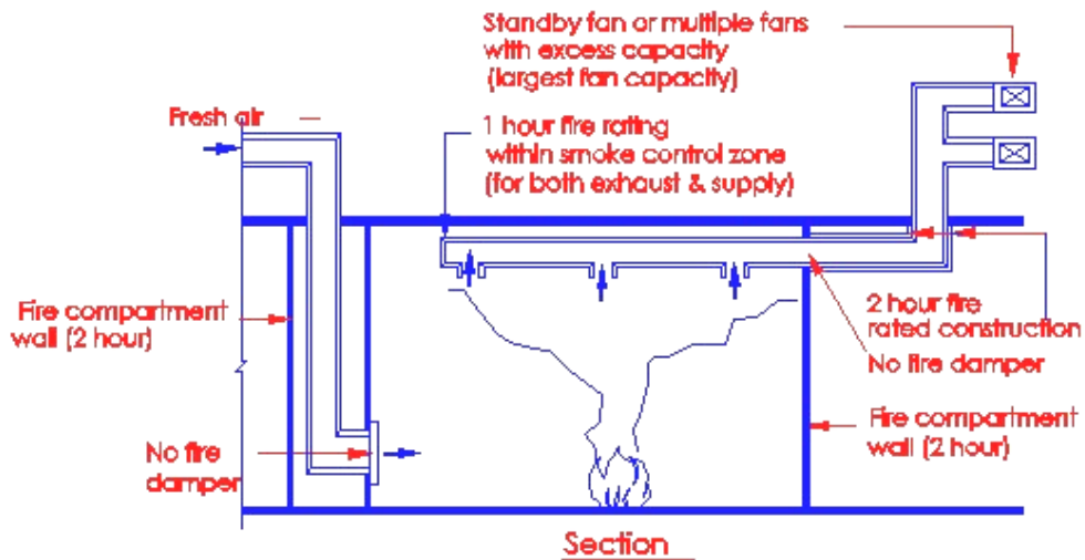
Diagram 7.6.20
