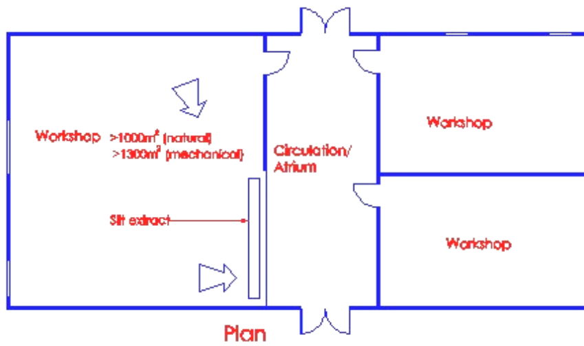
Drawing 7.6.9(b)
