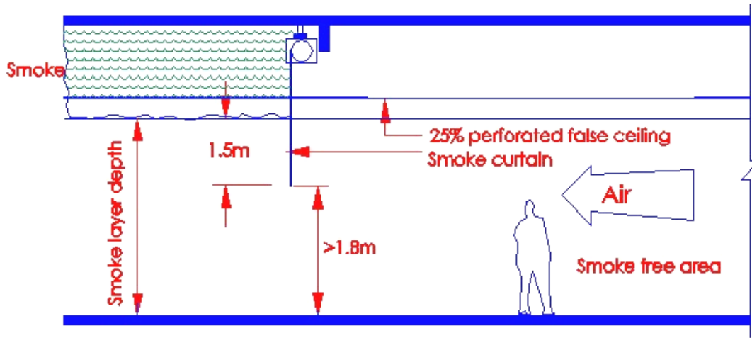
Diagram 7.6.13 - 1
