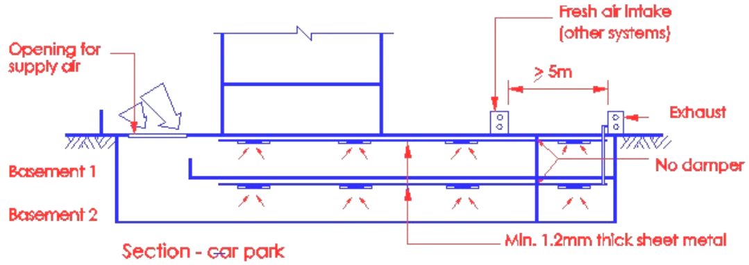
Diagram 7.1.9 - 2
