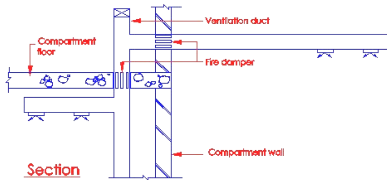
Diagram 7.1.1(i)- 1
