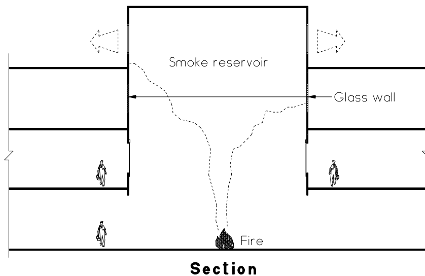
Diagram 7.6.31 – 1
