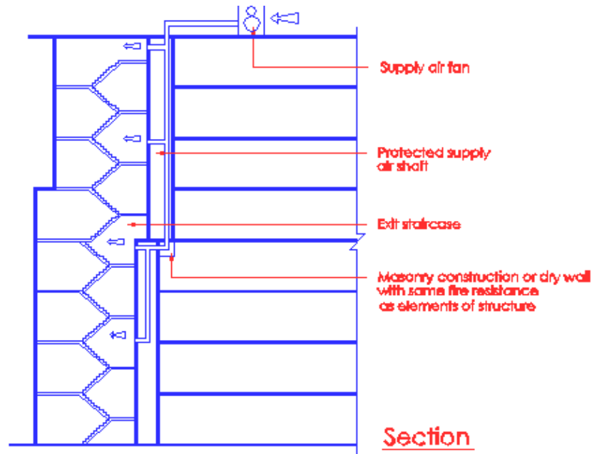
Diagram 7.1.3(b)(iii)
