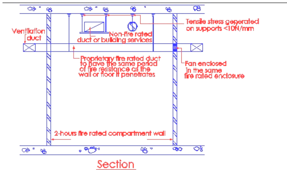
Diagram 7.1.1 (j) (iii)
