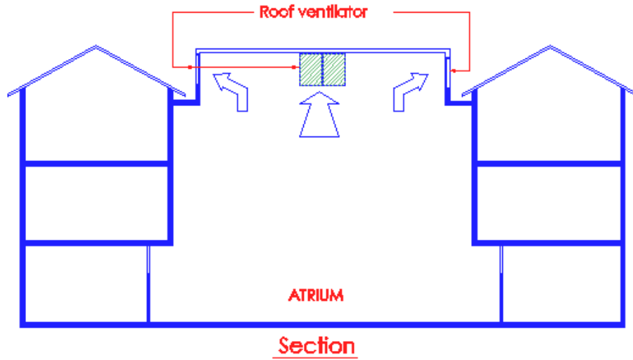
Diagram 7.6.27
