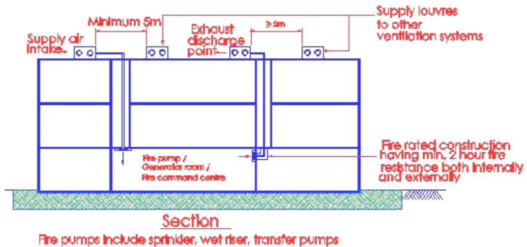
Diagram 7.1.5(a)
