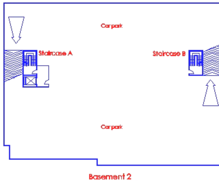
Diagram 7.4.1(a) - 1
