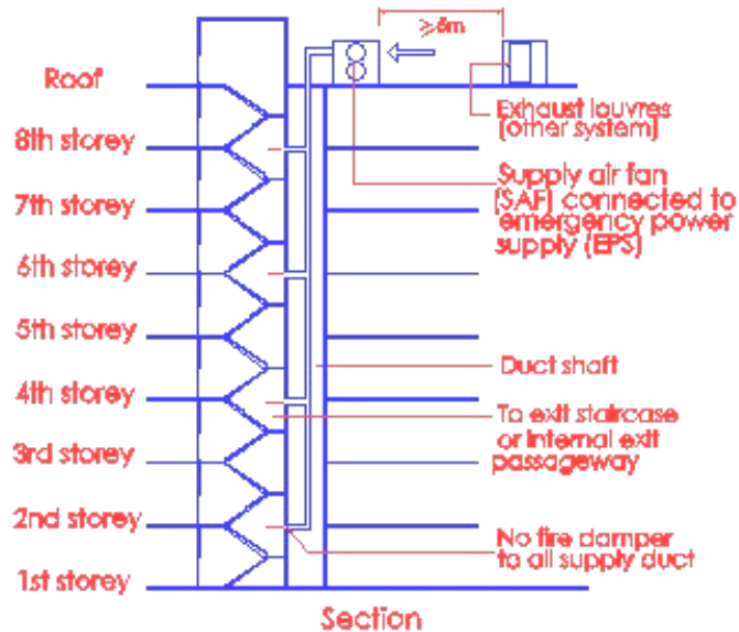
Diagram 7.1.3(b)(ii)
