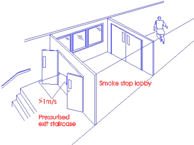
Diagram 7.2.3 - 2
