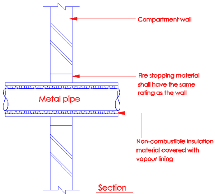
Diagram 7.1.1(c) - 2
