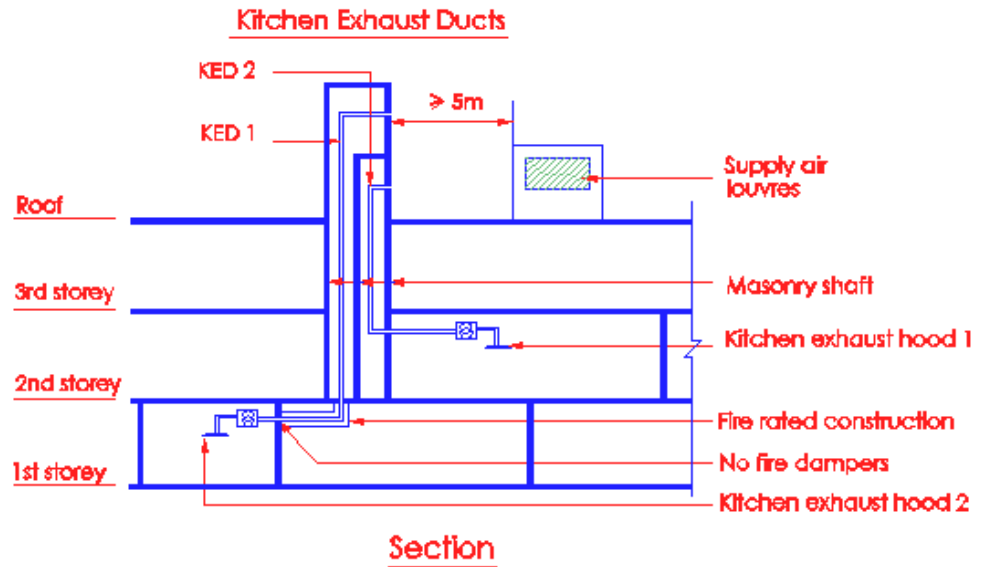
Diagram 7.1.7(a) - 1
