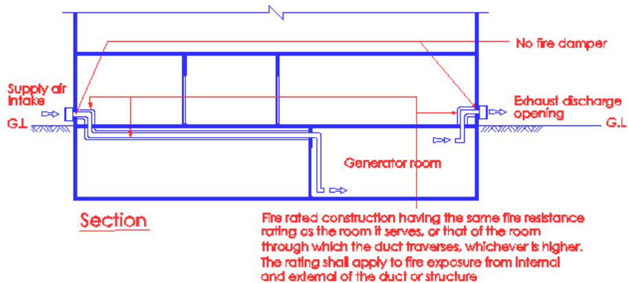
Diagram 7.1.5(c) - 1
