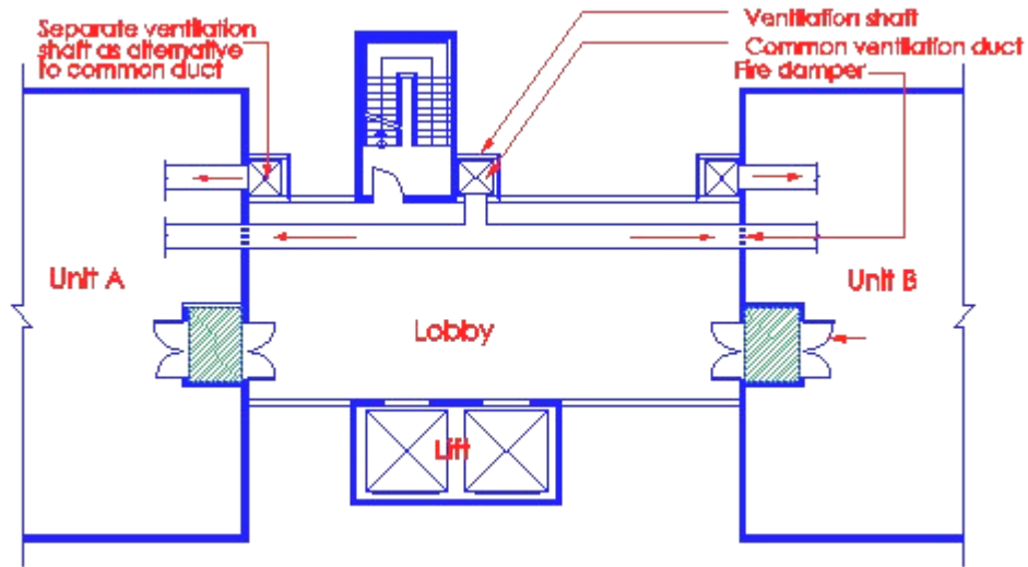
Diagram 7.1.1(e) - 1
