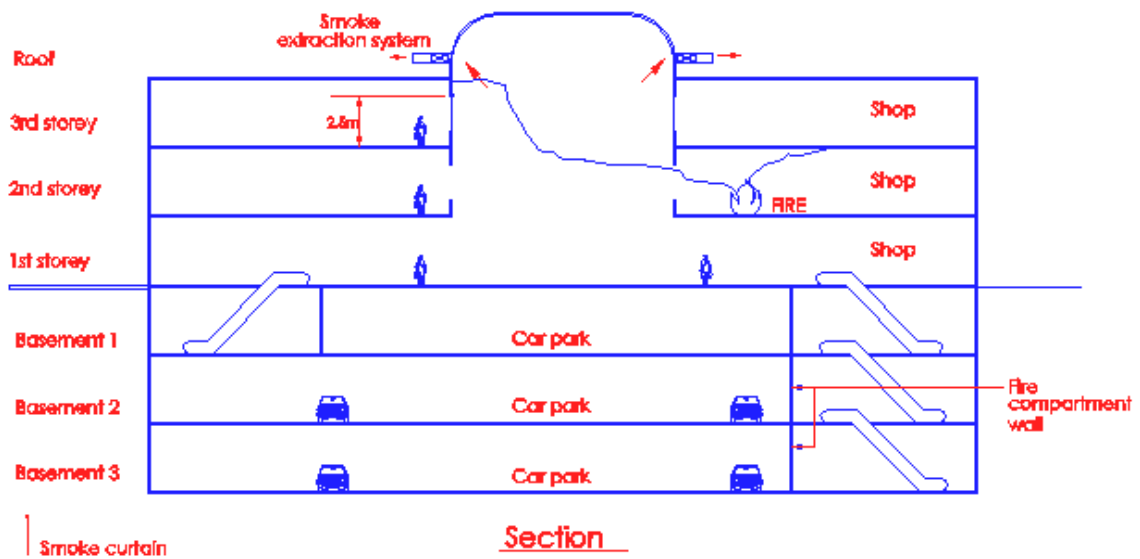
Diagram 7.6.4 - 2
