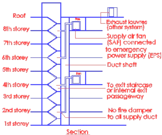
Diagram 7.1.3(b)(ii)
