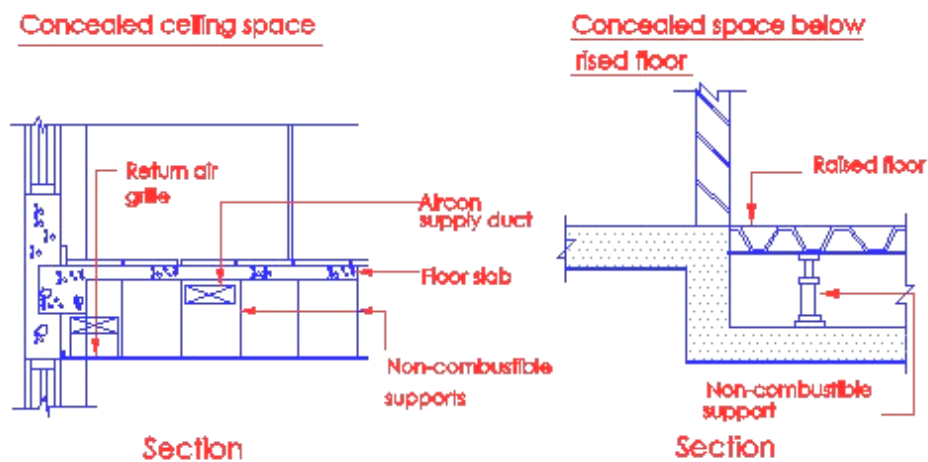
Diagram 7.1.1(f)
