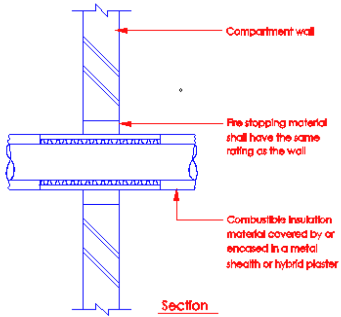
Diagram 7.1.1(c) - 1
