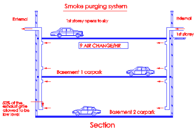
Diagram 7.1.1(h)(iii)
