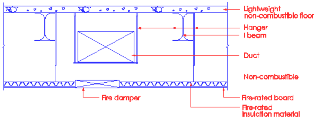
Diagram 7.1.1(i) – 2
