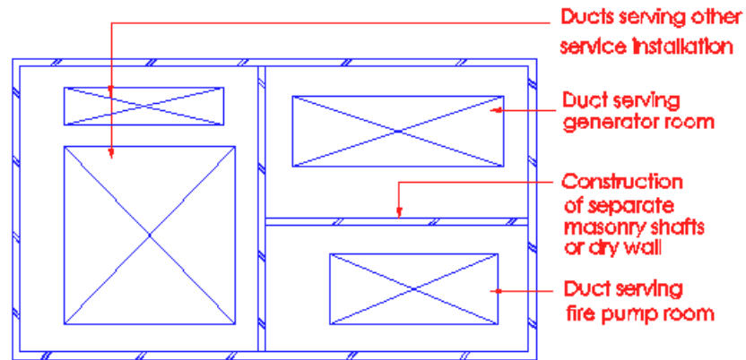
Plan of protected shaft
