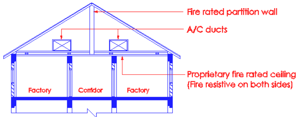
Diagram 7.1.1(i) - 1
