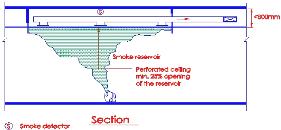
Diagram 7.6.14
