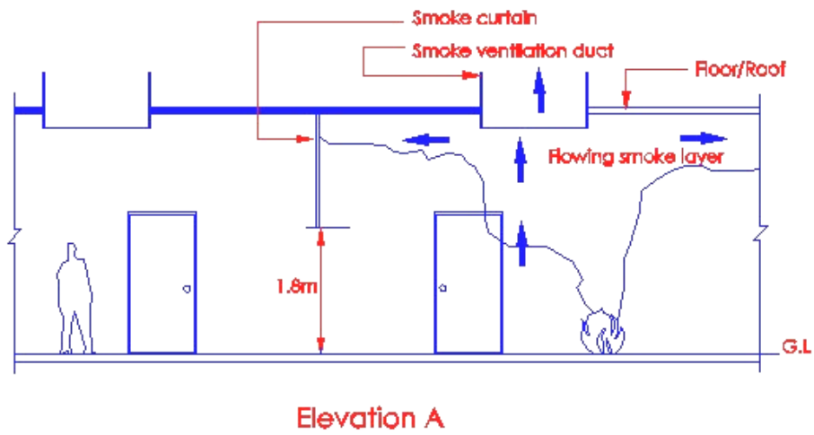
Diagram 7.6.8 - 3
