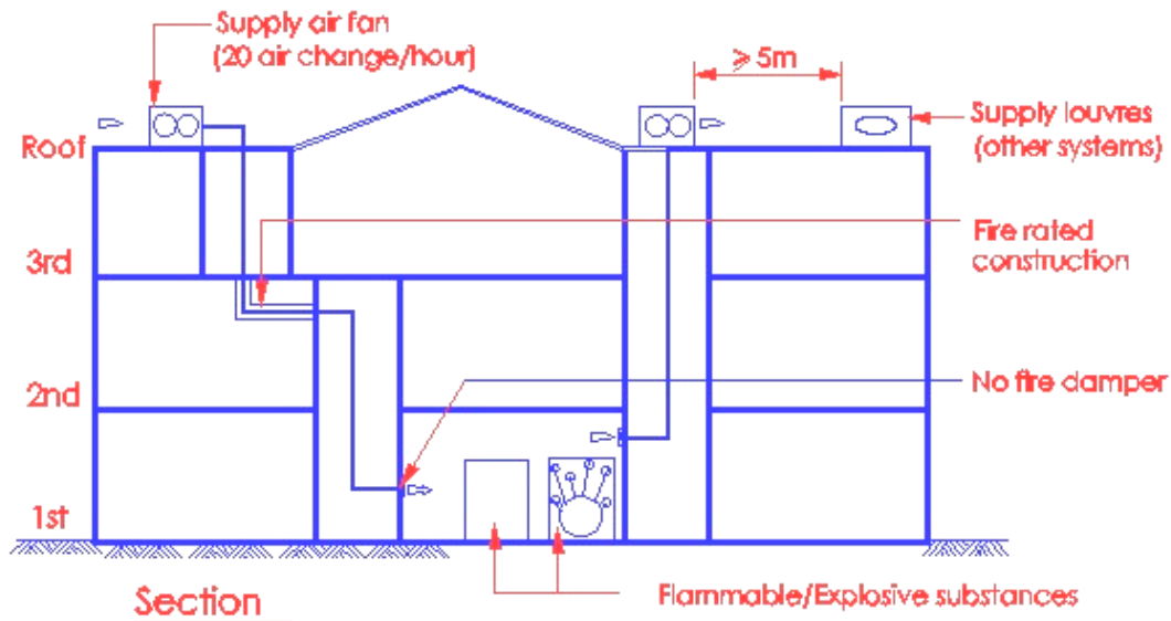
Diagram 7.1.8 - 1
