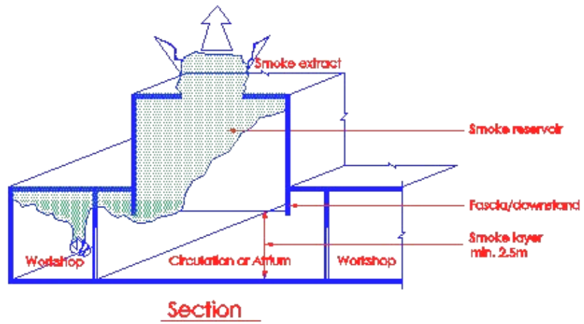
Diagram 7.6.8 - 1
