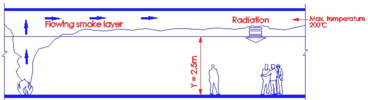
Diagram 7.6.5
