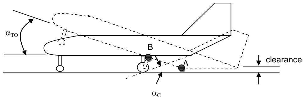
Figure 9.14. Take-off rotation and rear fuselage clearance
