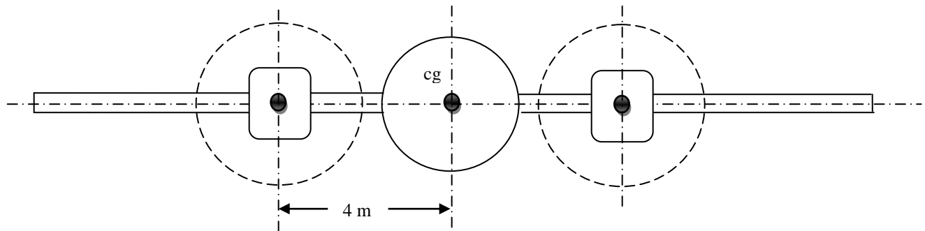
Figure 9.31. Aircraft in Example 9.8
