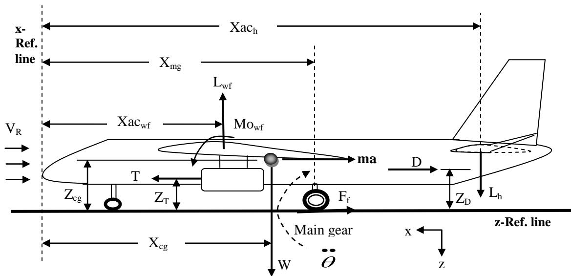
Figure 9.25. Forces and moments during take-off rotation
