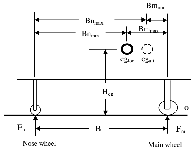
Figure 9.18. Wheel load geometry
