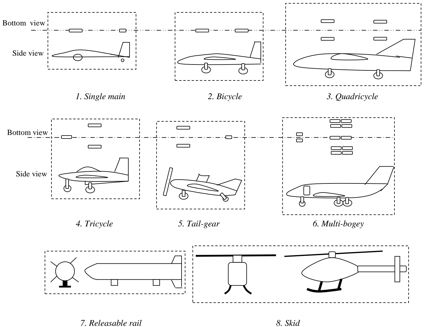
Figure 9.3. Landing gear types
