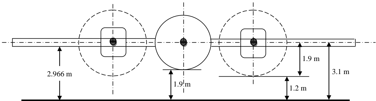
Figure 9.32. Prop clearance
