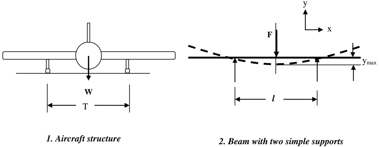
Figure 9.23. The aircraft structure at front view may be modeled as a beam with two simple supports
