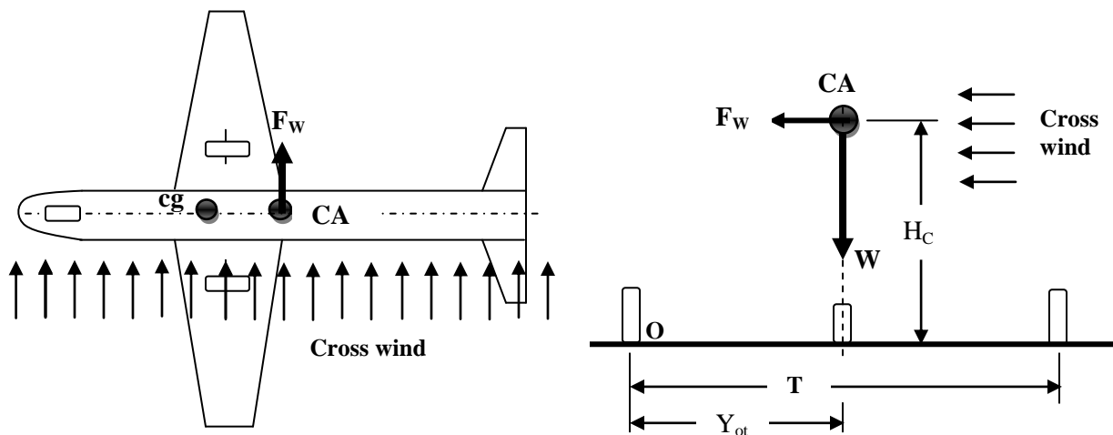
1. Top-view
