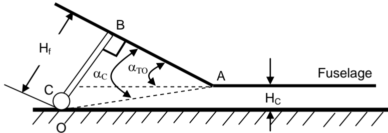
Figure 9.15. Examination of rear fuselage clearance during take-off rotation
