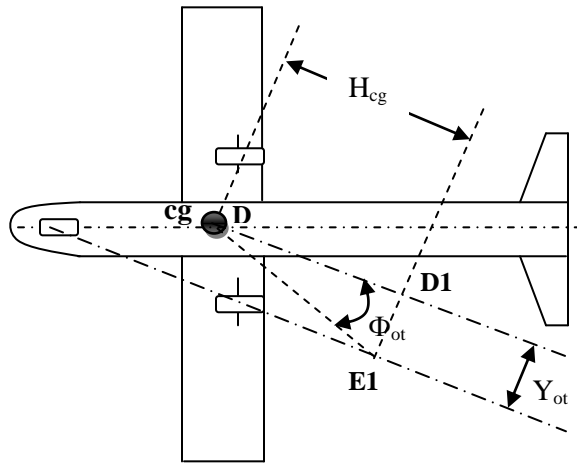
1. Aircraft top view
