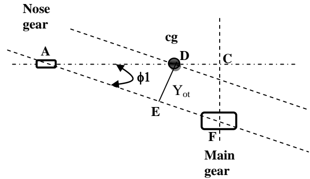
2. Top view (main gear and nose gear)
