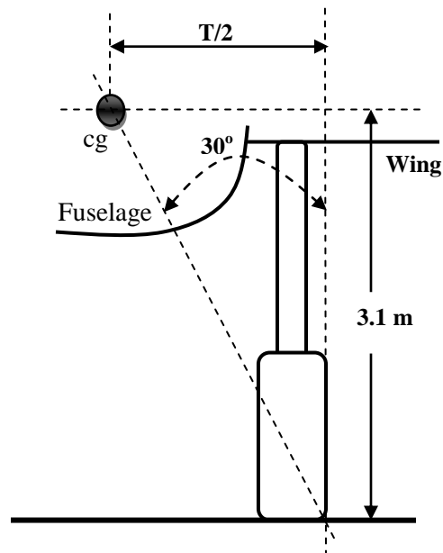
Figure 9.35. Wheel track (front view)
