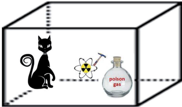
Figure 3. Inside the box we equipped a bottle of poison gas and a device (i.e., hammer) to break the bottle, triggered by the decaying of a radioactive particle, to kill the cat.
