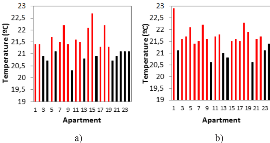
Figure 10. Average indoor temperature from group I ( N=24 ) during a) January 2005 and b) January 2006 (red bars are for temperatures above 21°C).
