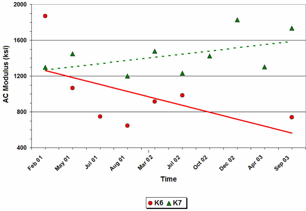
Figure F1. Corrected AC Moduli Using Eq. 7.2 (Group 1 FWD Stations).
