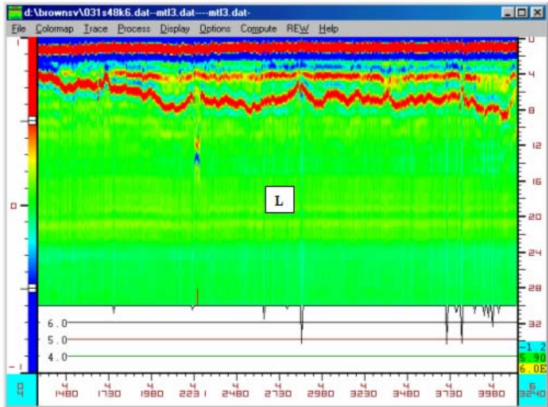
Figure A9. GPR Data on K6-L Section.
