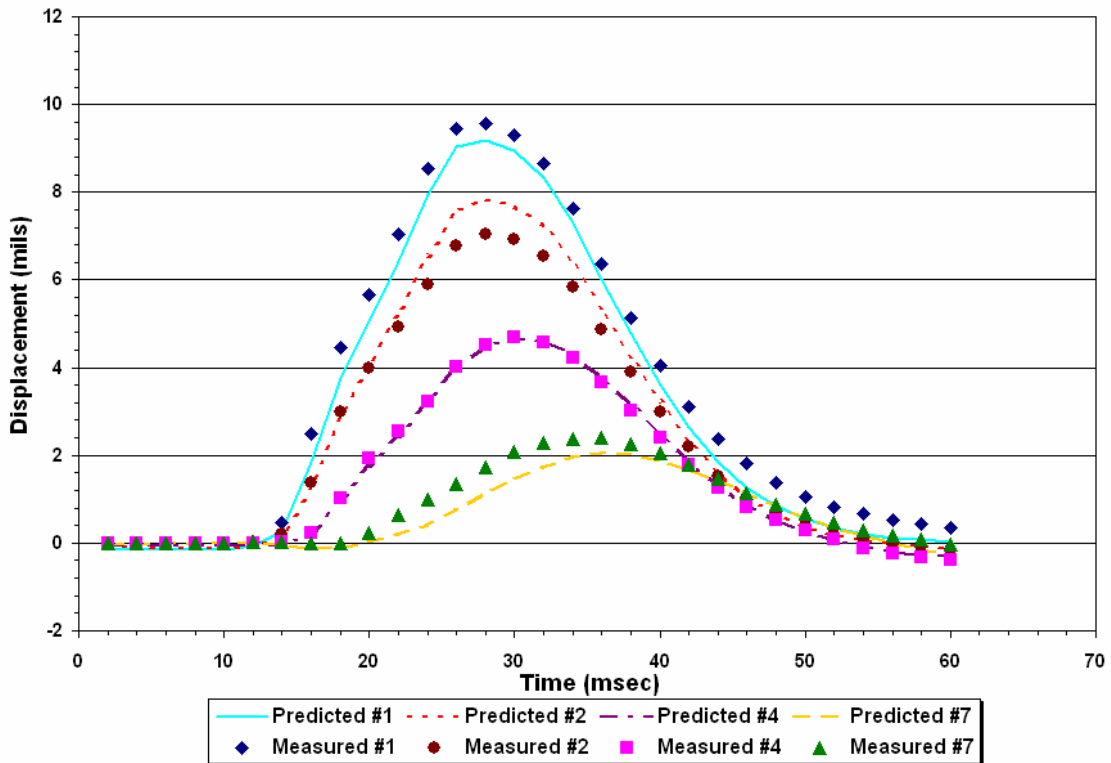
Figure D44. Comparison of Measured and Predicted FWD Displacement Histories on K7-9 (Data Collected in Aug 01).
