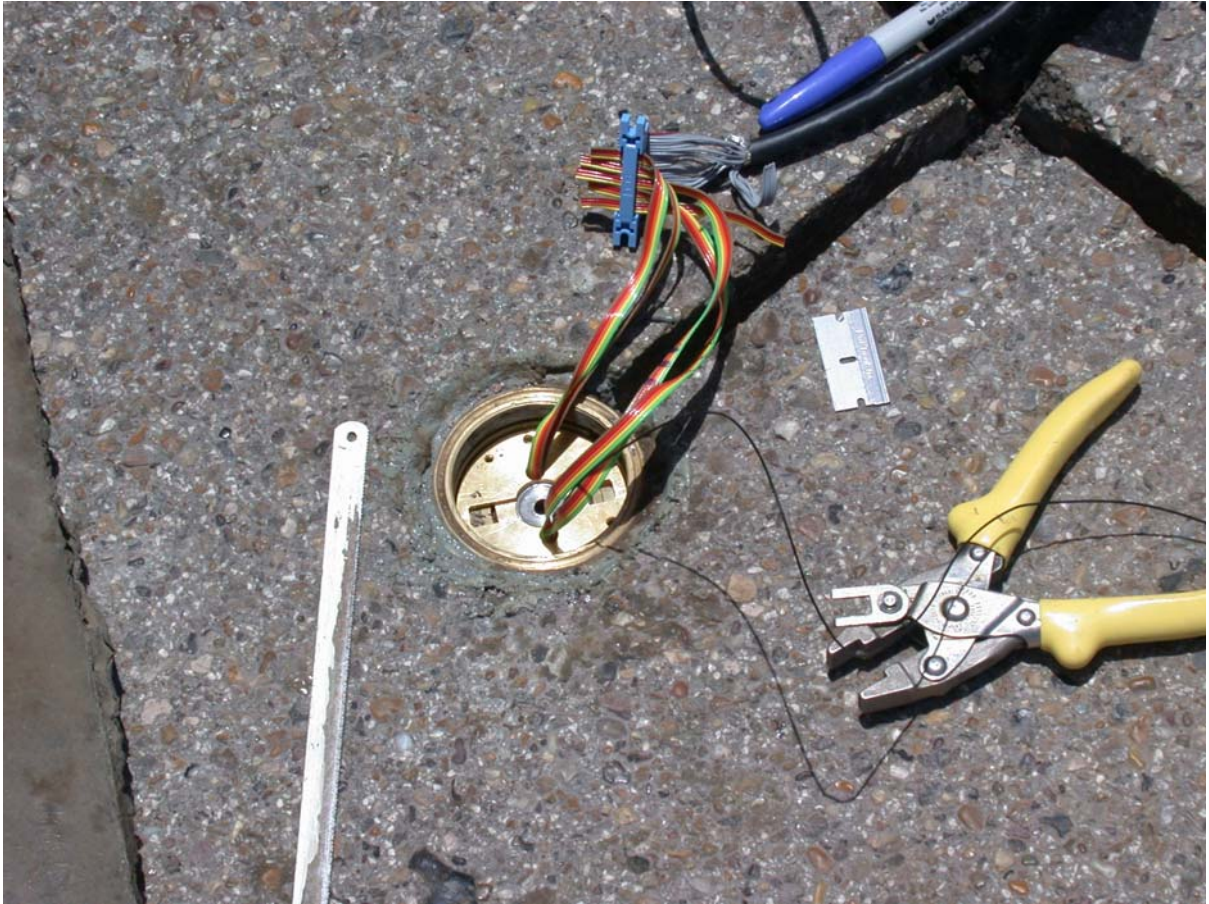
Figure B14. Setup after Installing All MDD Sensors Inside Hole.
