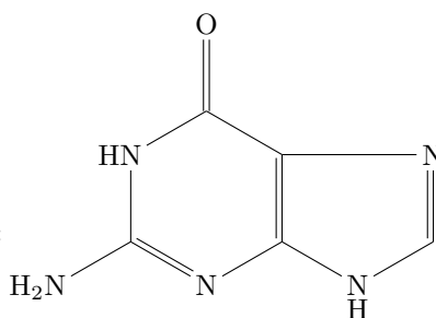
Guanine, structure
