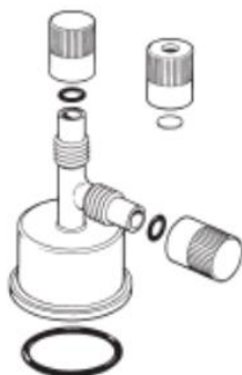
Fig. 1B. Sure/Seal septum-inlet transfer adapter
