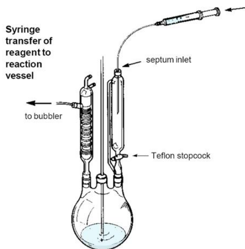
Fig. 2C Syringe transfer of reagent to reaction vessel
