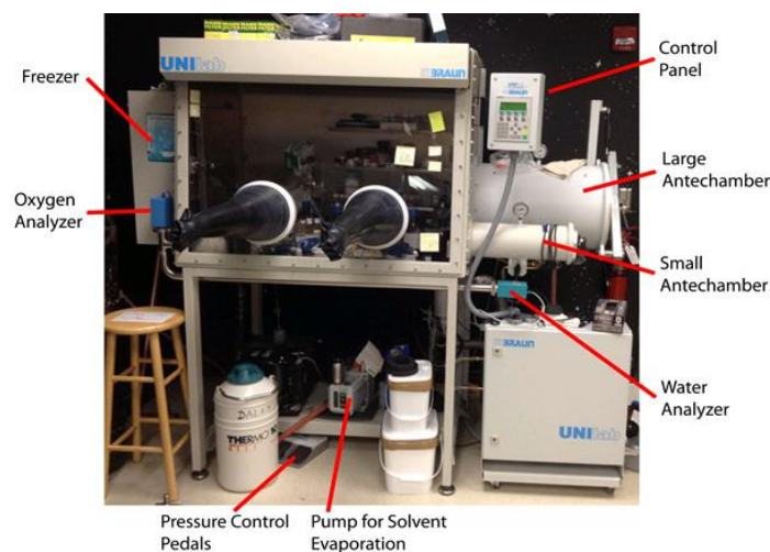
Figure 4.3 – Glovebox
