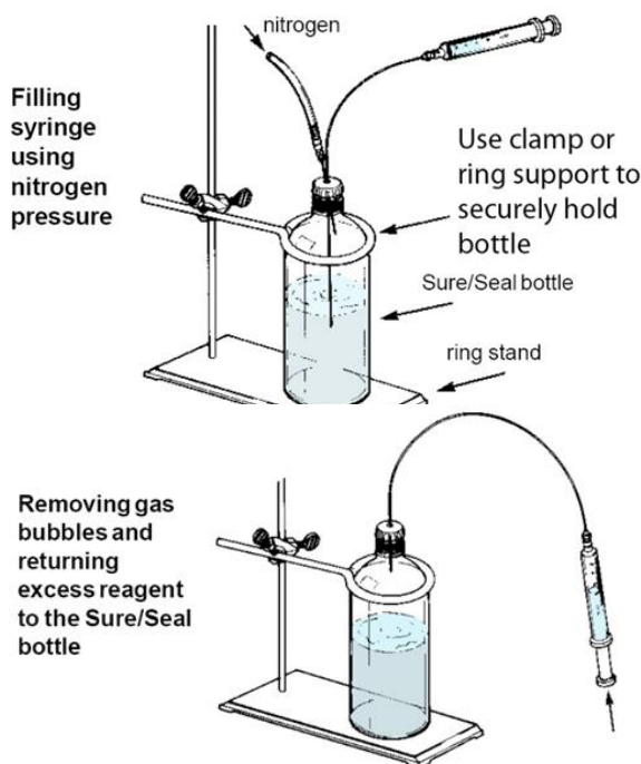
Fig. 2B. Removing gas bubbles and returning excess reagent to the Sure/Seal bottle
