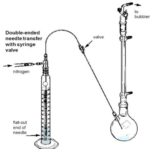
Fig. 3C. Double-ended needle transfer with syringe valve
