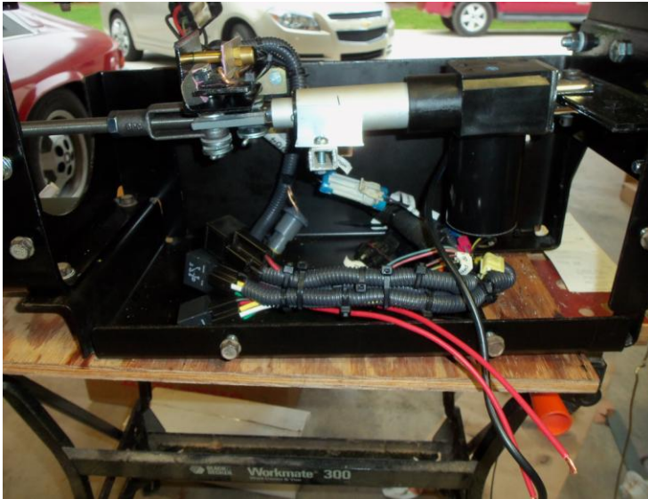
Completed assembly showing the uncomplicated design of the 12-volt linear actuator compared to the original hydraulic system, which was much more complex; see photo at right.
