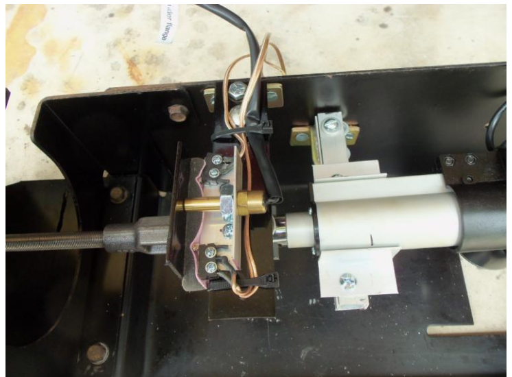
I used the other MB3 mounting bracket as a support for the piece I mounted the three switches to. The two side switches are for the RSG and the other pressure switch. The center switch is the switch that was mounted in the hydraulic cylinder at the spring to indicate when the brake was not fully on.
