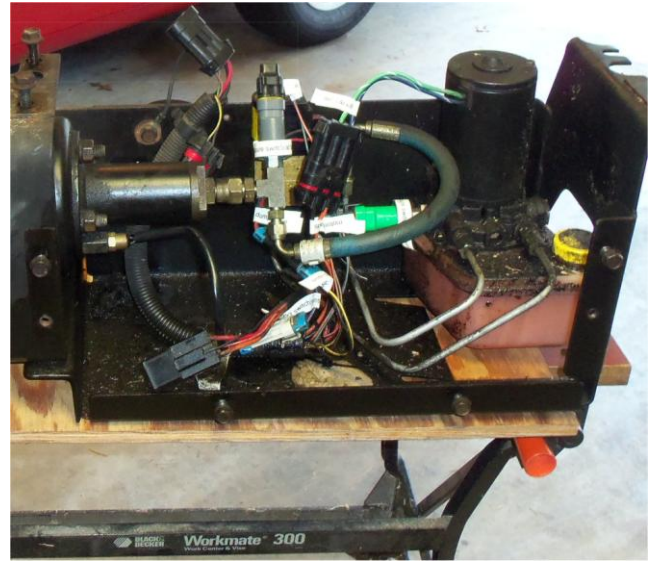
The original hydraulic system, which is prone to leaking and failure while driving.
