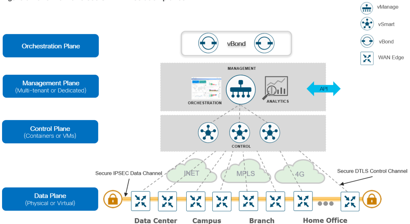
Figure 9. Overview of Cisco SD-WAN solution planes
