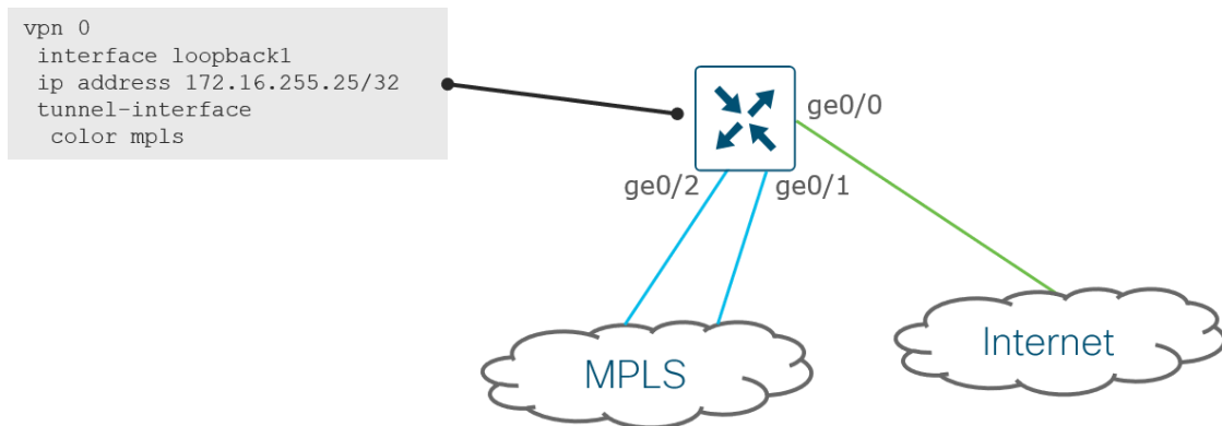
Figure 68. Loopback interface tunnel use case: scaling traffic to the same transport
