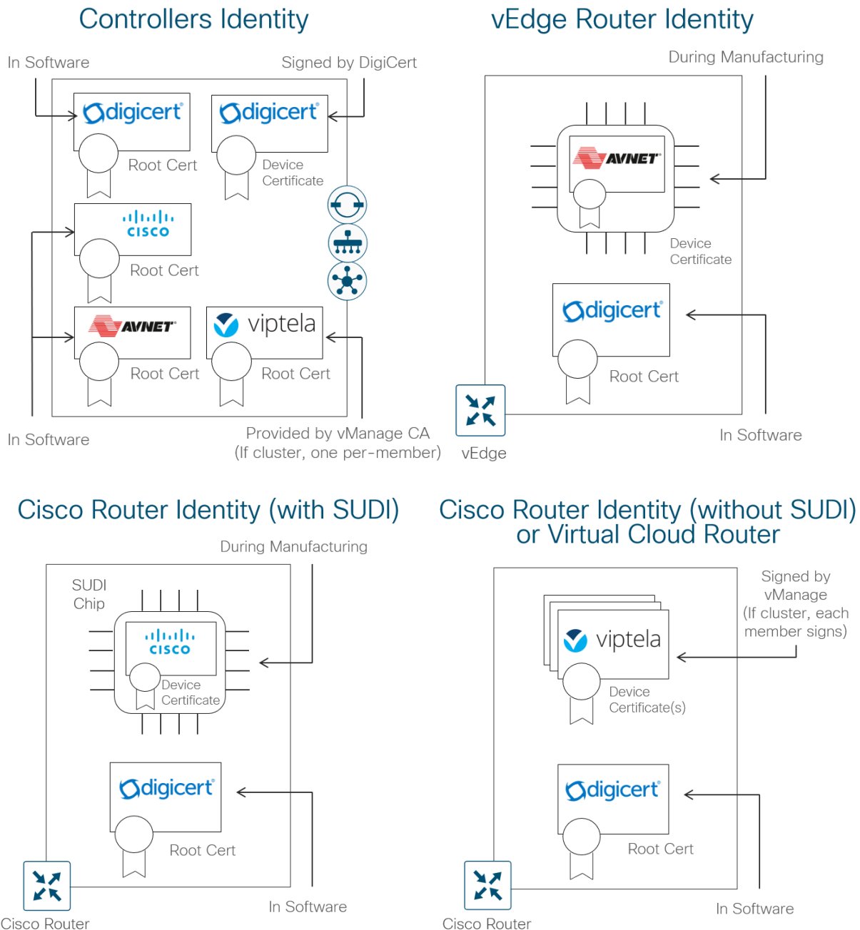
Figure 17. Certificates present for authentication purposes
