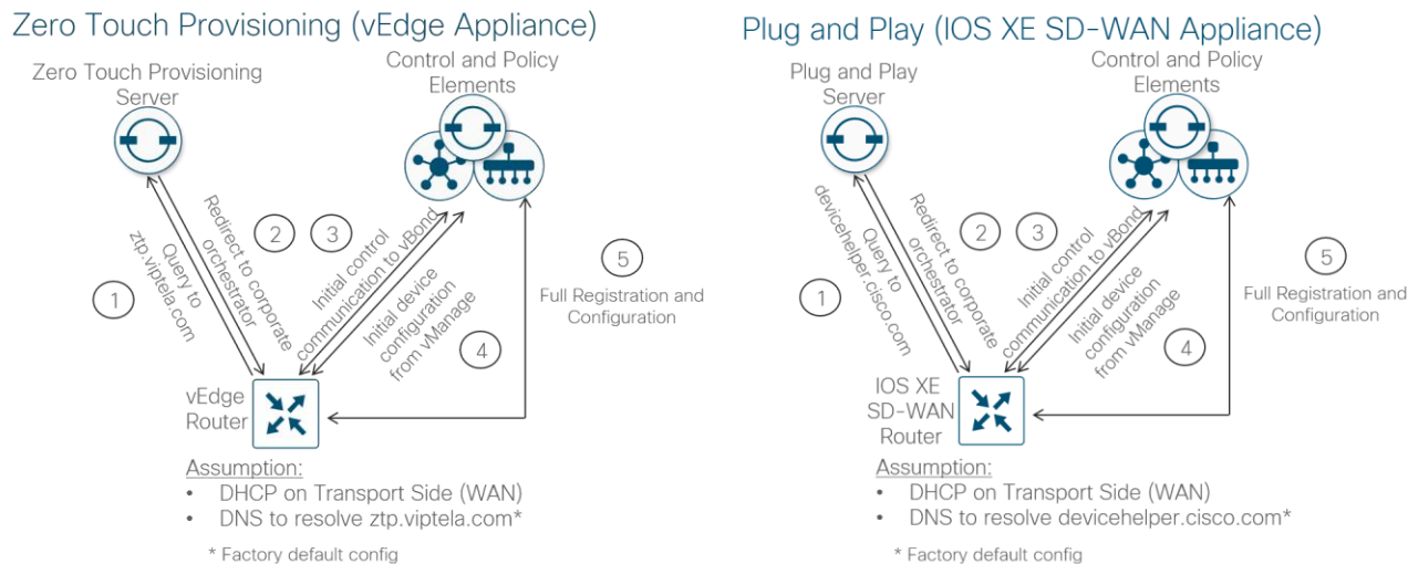
Figure 20. Automated device provisioning for a WAN Edge appliance
