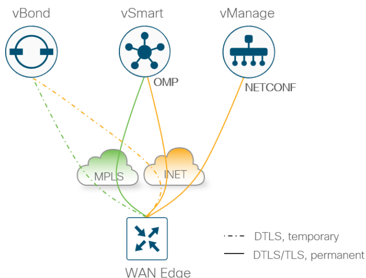
Figure 13. WAN Edge control connections
