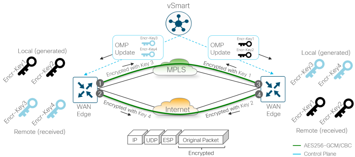
Figure 22. Data plane encryption keys
