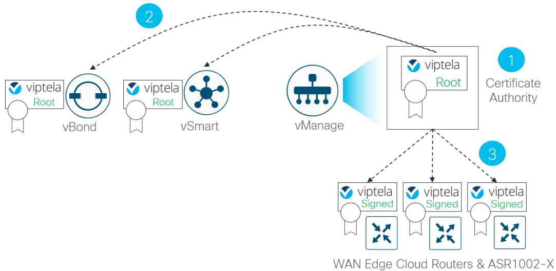
Figure 16. vManage root CA for WAN Edge cloud routers and the ASR1002-X
