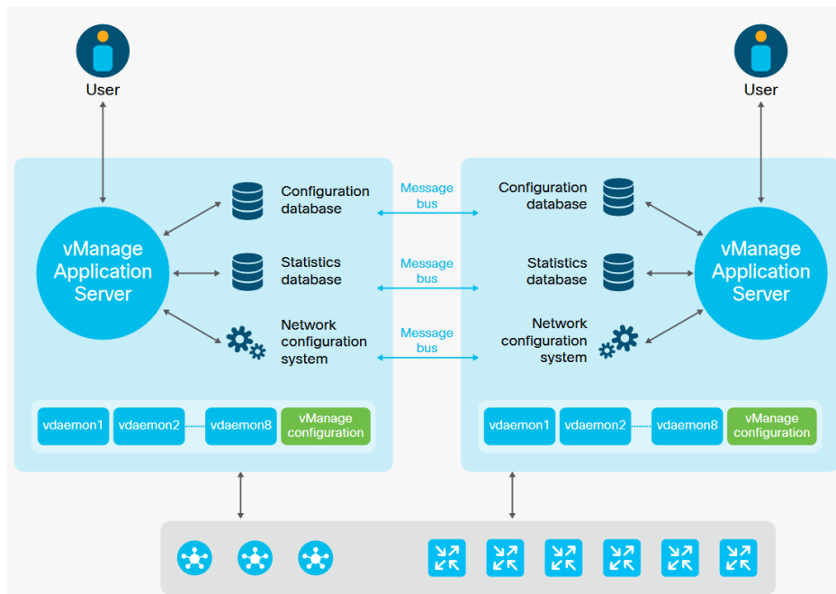
Figure 50. vManage cluster components
