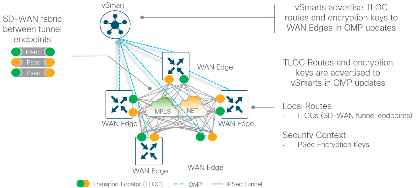
Figure 24. Data plane establishment
