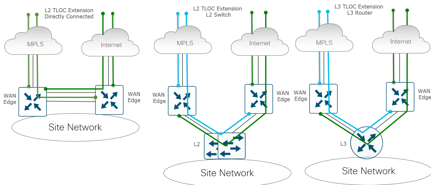
Figure 60. L2 vs L3 TLOC extension deployments
