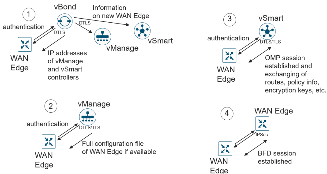
Figure 19. Bringing a WAN Edge into the overlay
