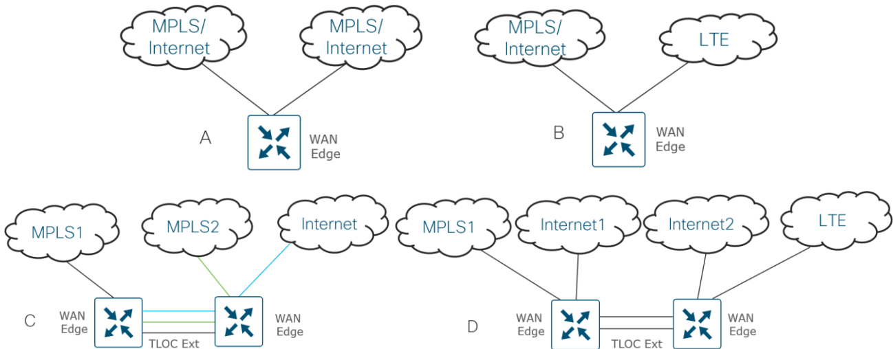
Figure 62. Multiple SD-WAN transport choices
