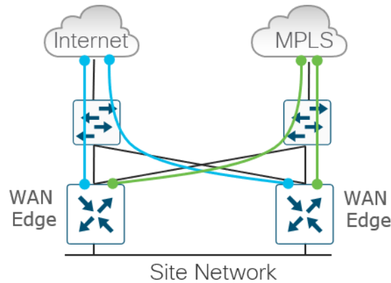
Figure 58. L2 switch front-end for connection to all transports option
