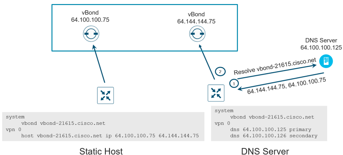
Figure 46. vBond orchestrator redundancy
