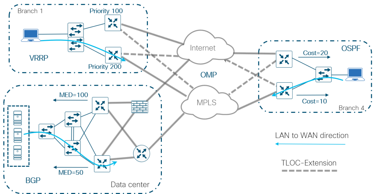
Figure 79. Influencing traffic in the LAN-to-WAN direction
