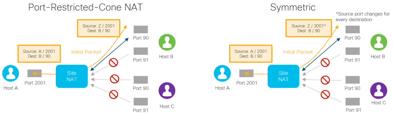
Figure 33. NAT types illustrated: Port-Restricted-Cone and Symmetric NAT
