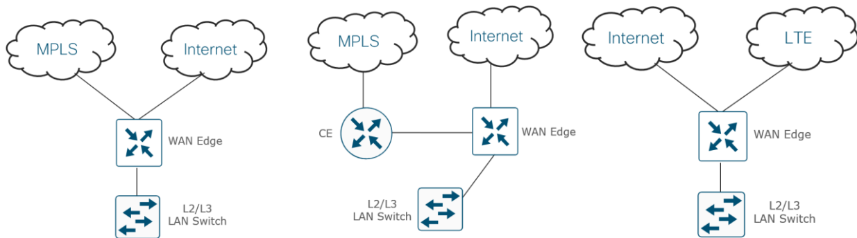
Figure 77. Single WAN-Edge branch deployment examples
