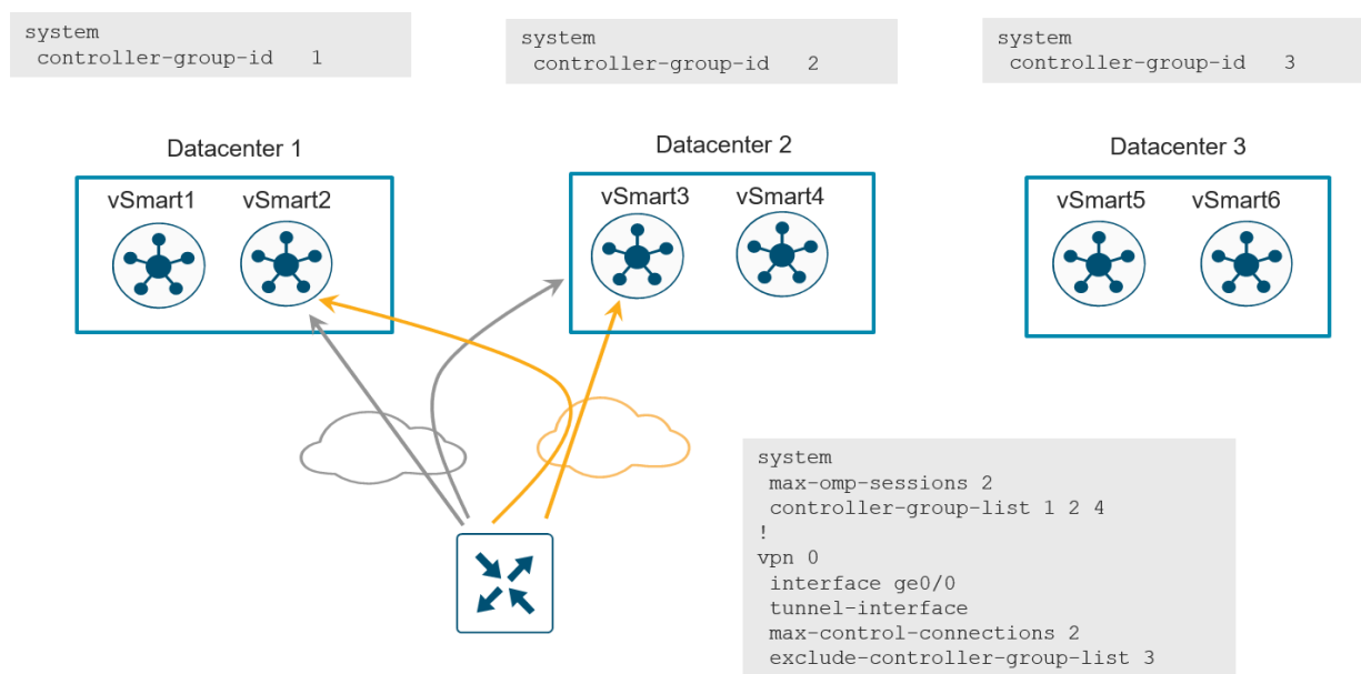
Figure 48. vSmart affinity example
