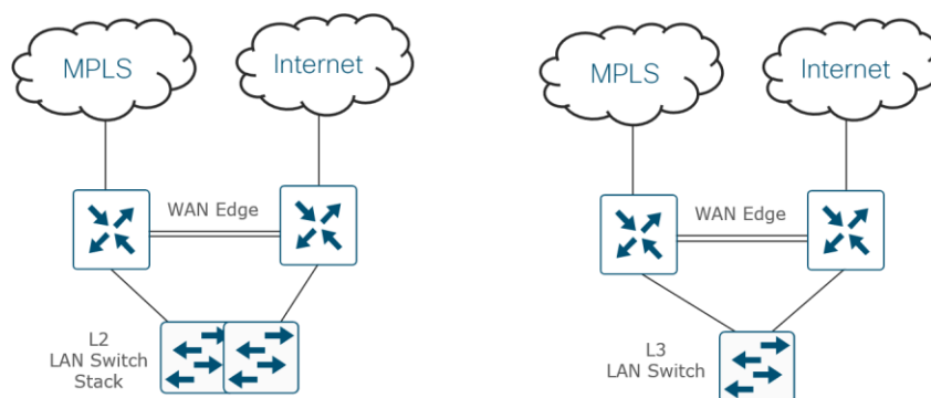
Figure 78. Dual WAN-Edge branch deployment examples
