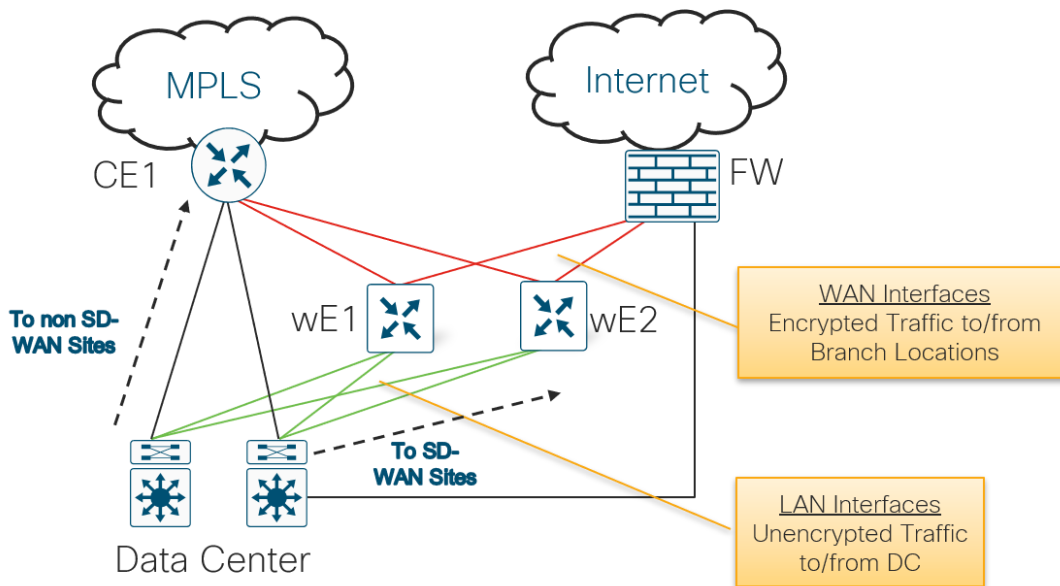
Figure 74. Data center deployment
