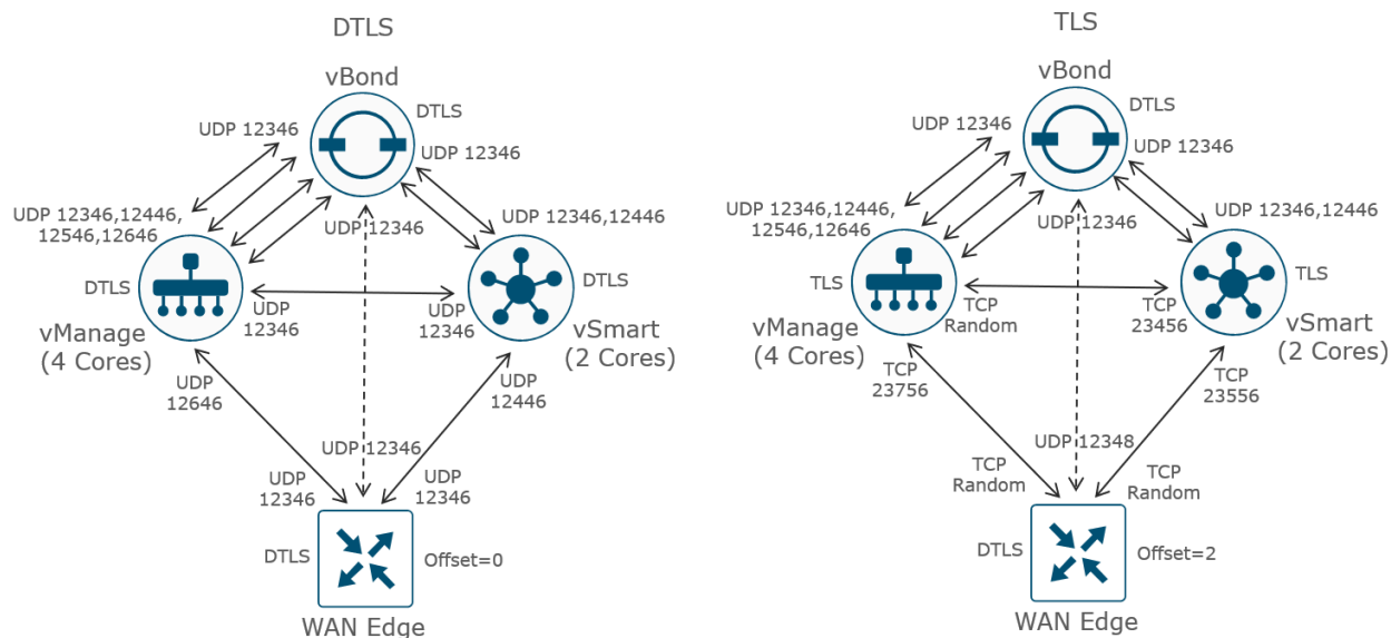
Figure 38. Control connections DTLS and TLS port examples
