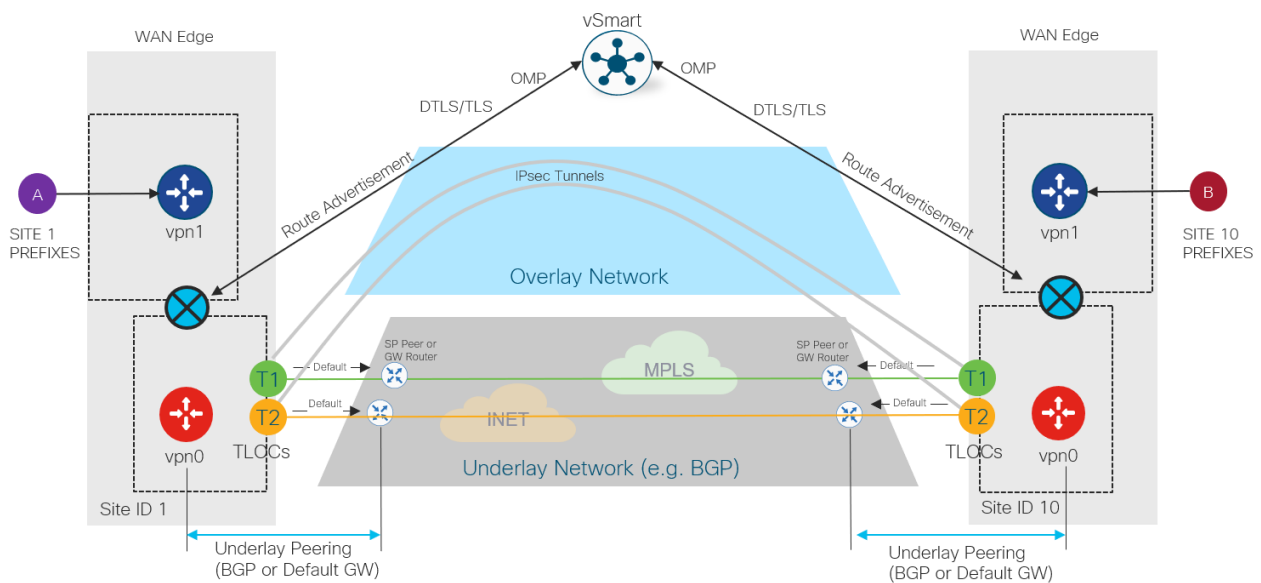
Figure 35. Underlay vs overlay routing
