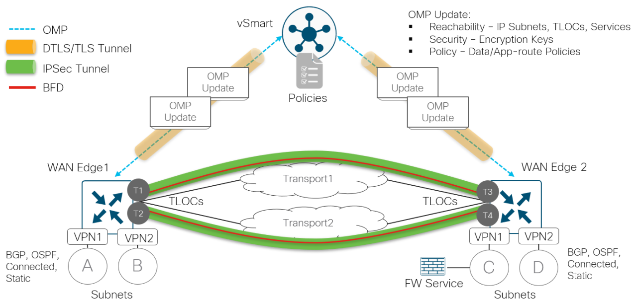
Figure 36. OMP operation
