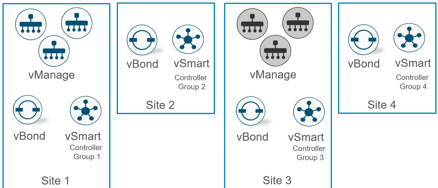
Figure 54. Small controller deployment example
