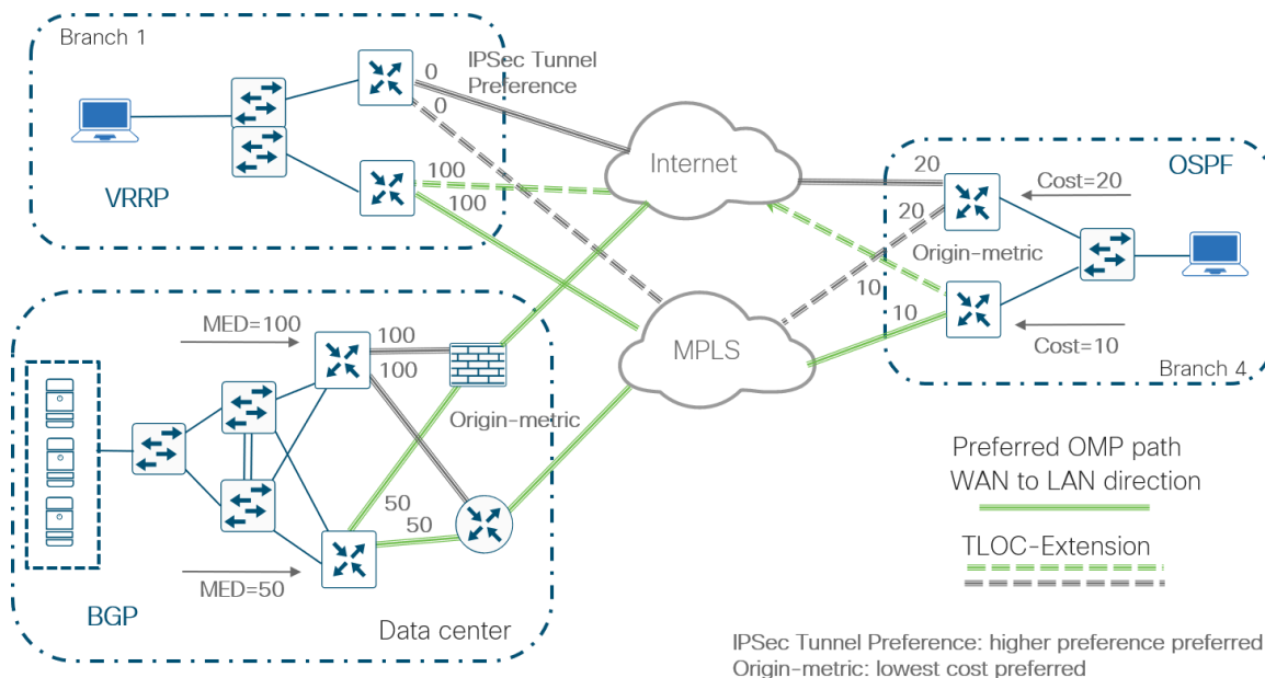
Figure 80. Influencing traffic in the WAN-to-LAN direction
