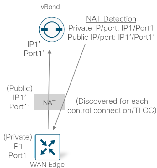
Figure 21. vBond facilitates NAT traversal
