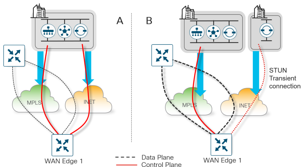
Figure 45. On-premise deployment control and data plane establishment
