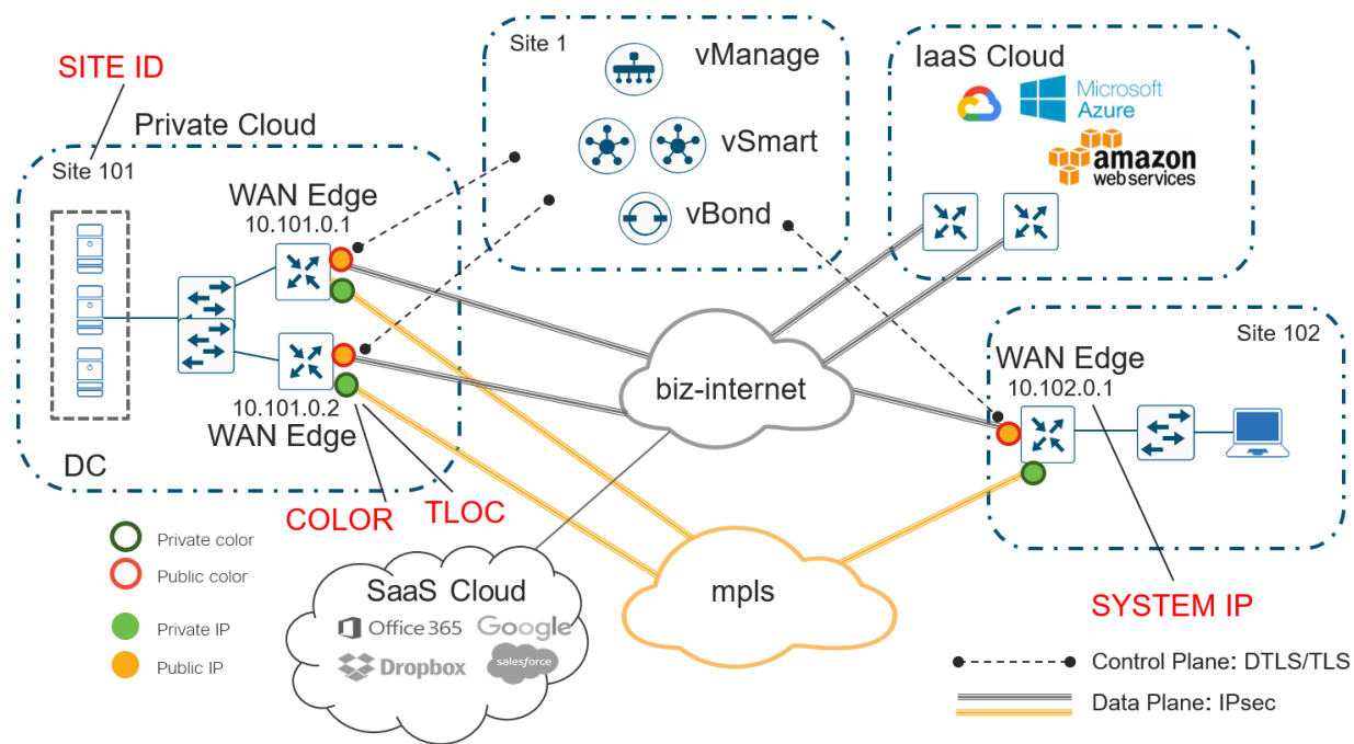
Figure 10. Example SD-WAN topology
