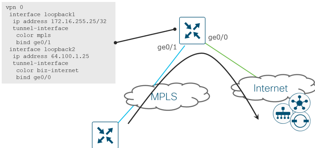
Figure 69. Loopback interface tunnel use case: MPLS Edge routers need access to controllers on Internet
