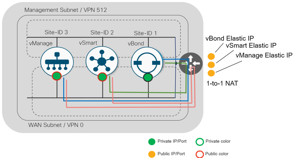
Figure 44. Cloud-hosted deployment: controller communication
