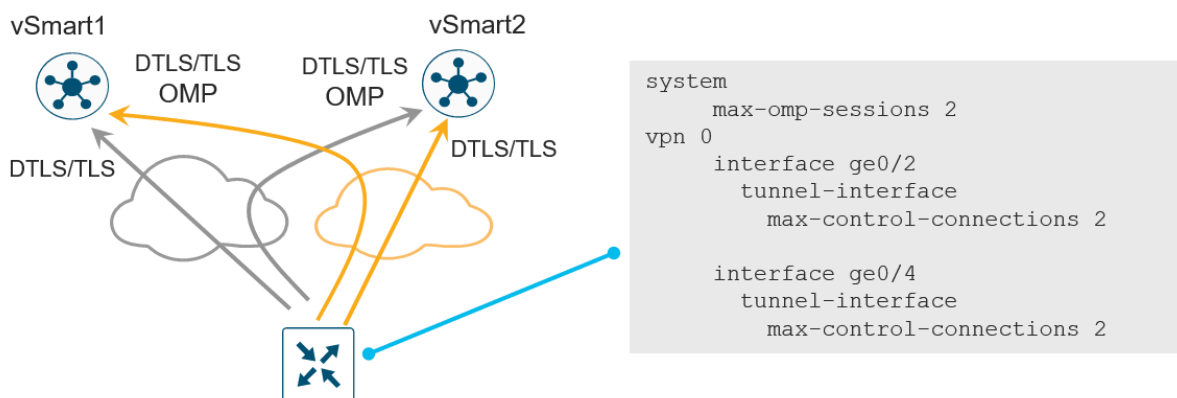
Figure 47. vSmart controller redundancy
