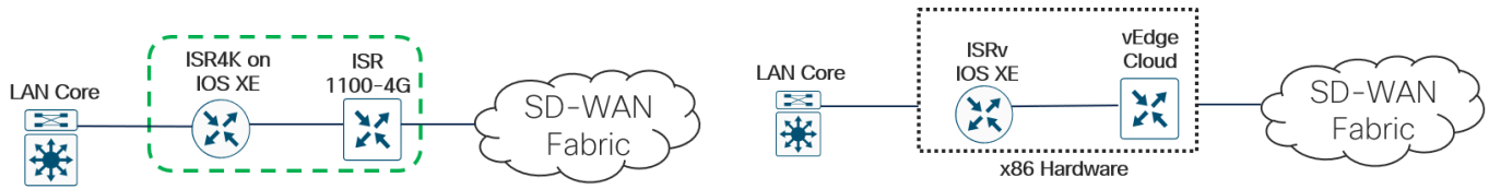
Figure 75. Hardware and virtualized SD-WAN LAN-side service-point deployment
