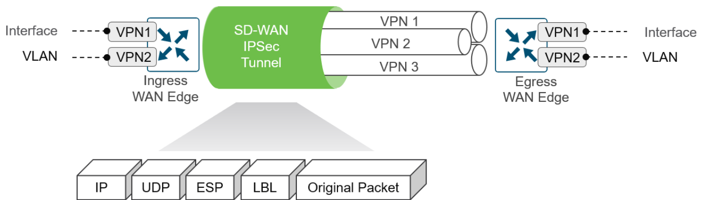
Figure 2. End-to-end segmentation
