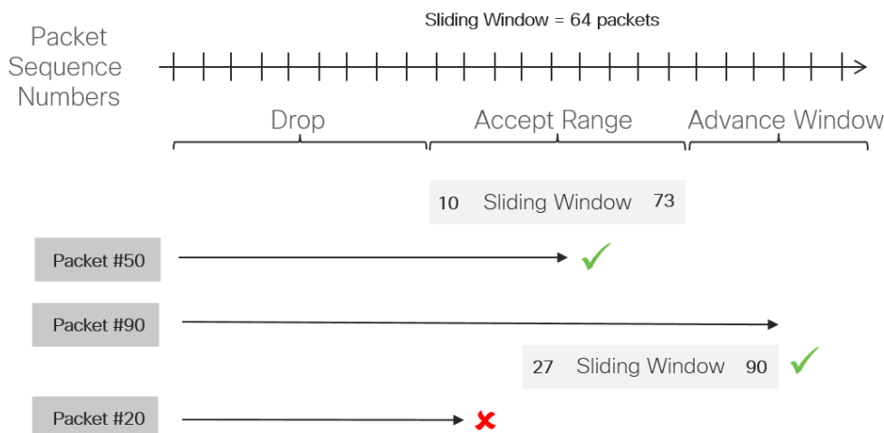
Figure 23. Anti-replay
