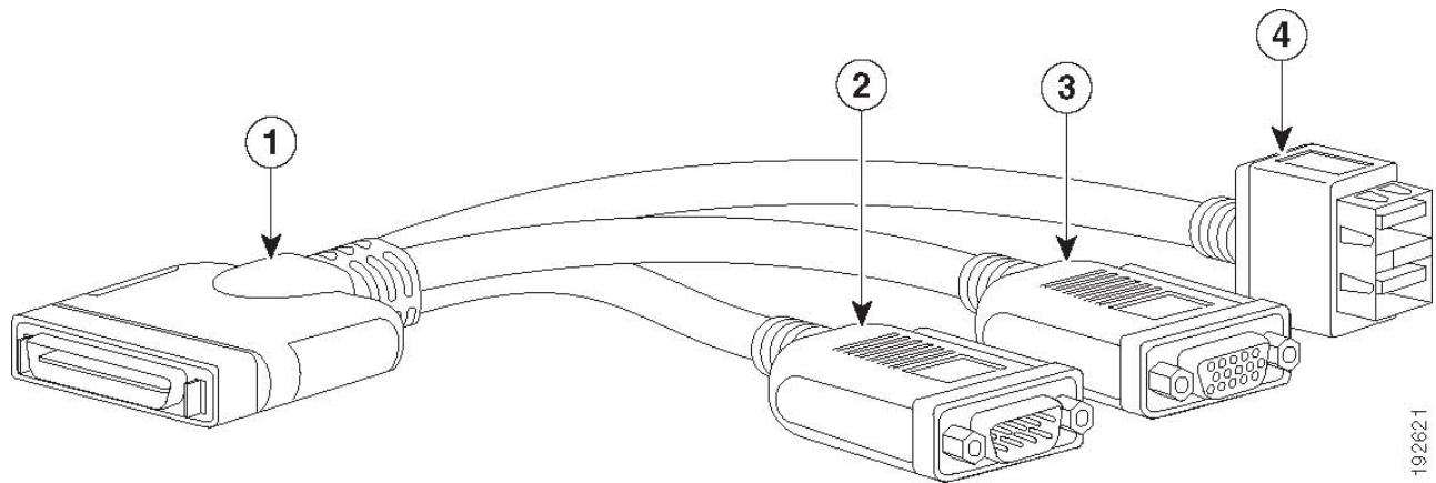
Figure 4 KVM Cable
