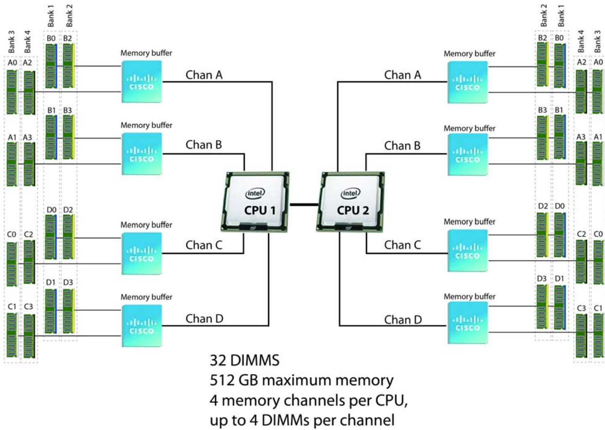
Figure 3 B230 M2 Memory Organization
