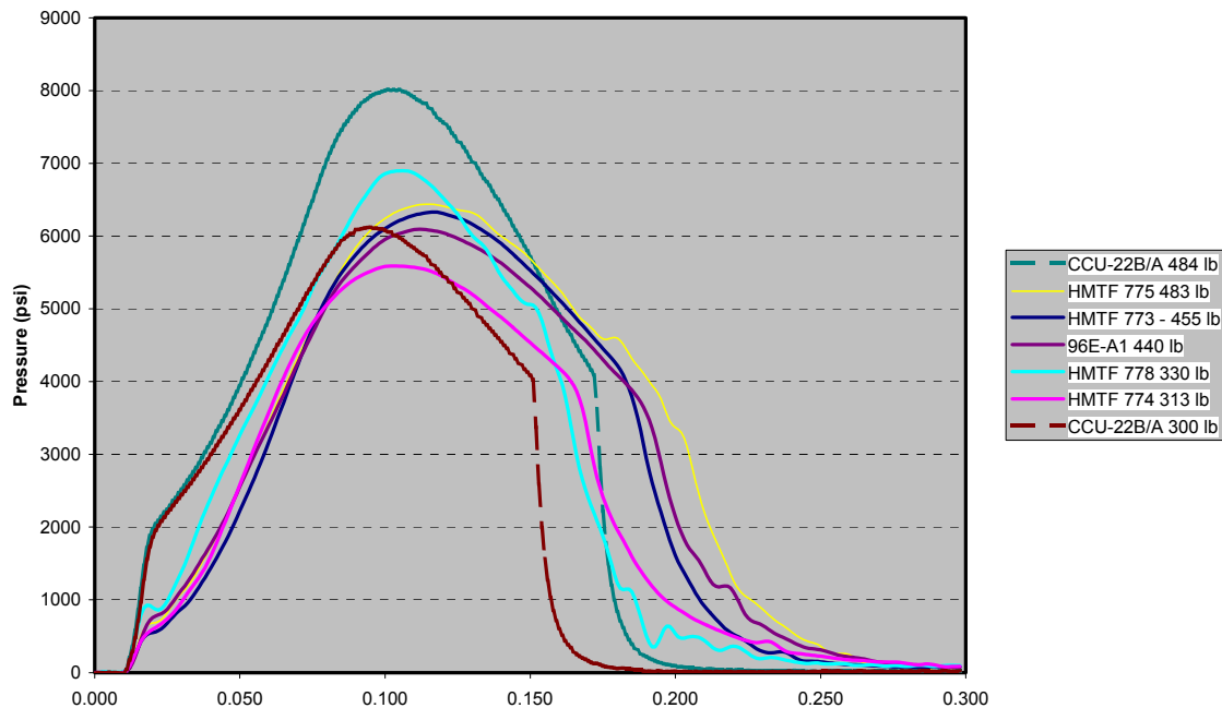
Figure 13. Comparison of Catapult Pressure Results
