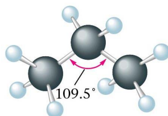
(a) Propane
