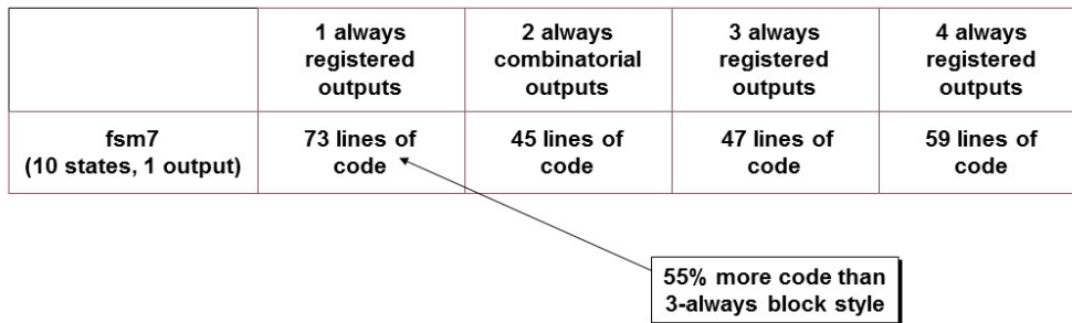
Figure 16 - fsm7 - Lines of code
