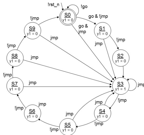
Figure 14 - FSM7 state diagram
