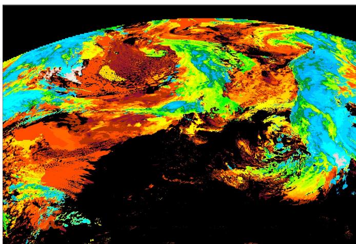
Cloud Top Pressure [hPa 1E-2]
