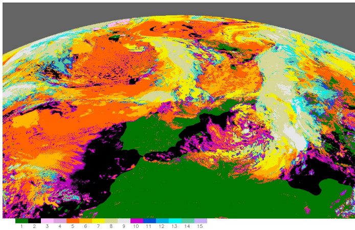
Cloud type number
