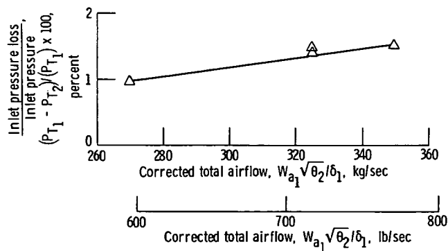
Figure 15. - Pressure loss of sound suppressing inlet.
