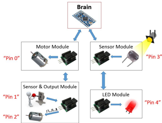
Fig. 5. As devices are added to the design, each one is automatically assigned a virtual pin number. Users can then control the robot using the virtual pin numbers, so that knowledge of the actual chain configuration is not required.
