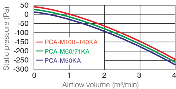
Outside-air intake characteristics
