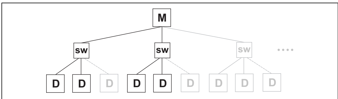
[4-4] Tree topology via switches (M = IO master, SW = switch, D = I/O device)
