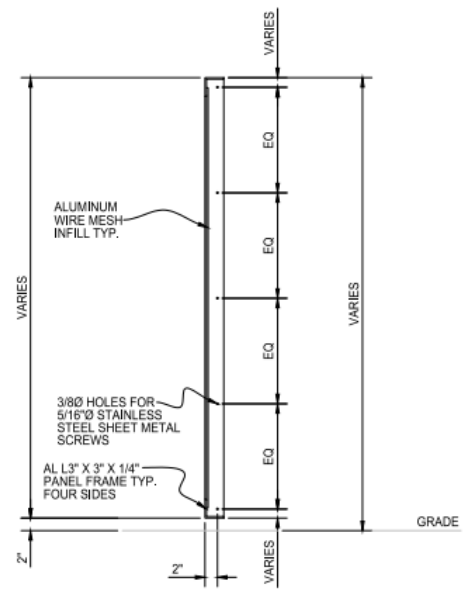
TYPICAL PANEL SECTION ALUM 2" X 2" SQUARE .25" WIRE WEAVE MESH
