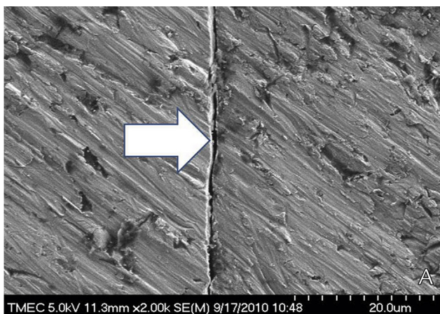
Figure 3. A, Microgap (white arrow) of conventional hexagon connection ( \times 2000 ). B, Microgap (white arrow) of Octatorx connection ( \times 2000 ).
