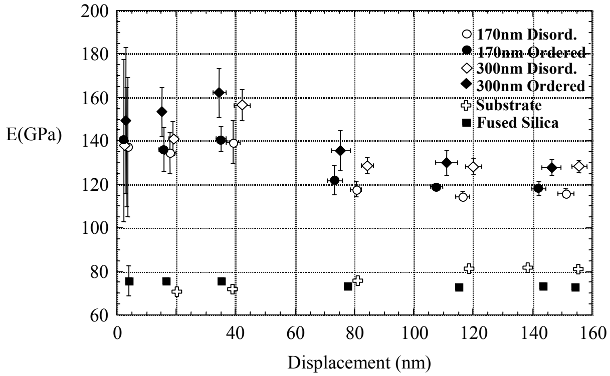
Fig 7. Young's Moduli calculated from nano-indentation data of Ni 3 Al thin films with thickness 170 nm and 300 nm, on oxidized silicon substrate with 1 \mu\text{m} SiO 2 . Within experimental error, there is no observable difference in Young's modulus between the ordered and disordered films. Results for bare oxidized wafers and bulk fused silica are also shown.
