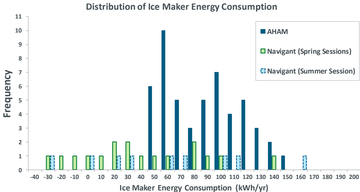
Figure 23. Distribution of ice maker energy consumption – AHAM vs. Navigant (Source: AHAM 2009)
