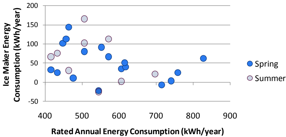
Figure 19. Ice maker energy consumption as a function of refrigerator rated annual energy consumption
