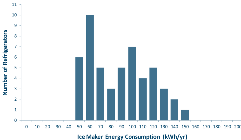
Figure 7. Distribution of Ice Maker Energy Consumption (Source: AHAM 2009)
