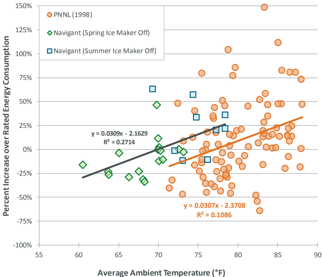
Figure 14. Comparison between rated energy consumption and actual energy consumption vs. average temperature – PNNL vs. Navigant (Source: PNNL 1998)
