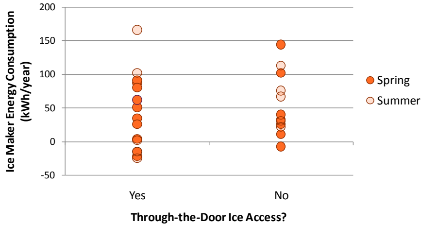
Figure 21. Ice maker energy consumption as a function of through-the-door ice access
