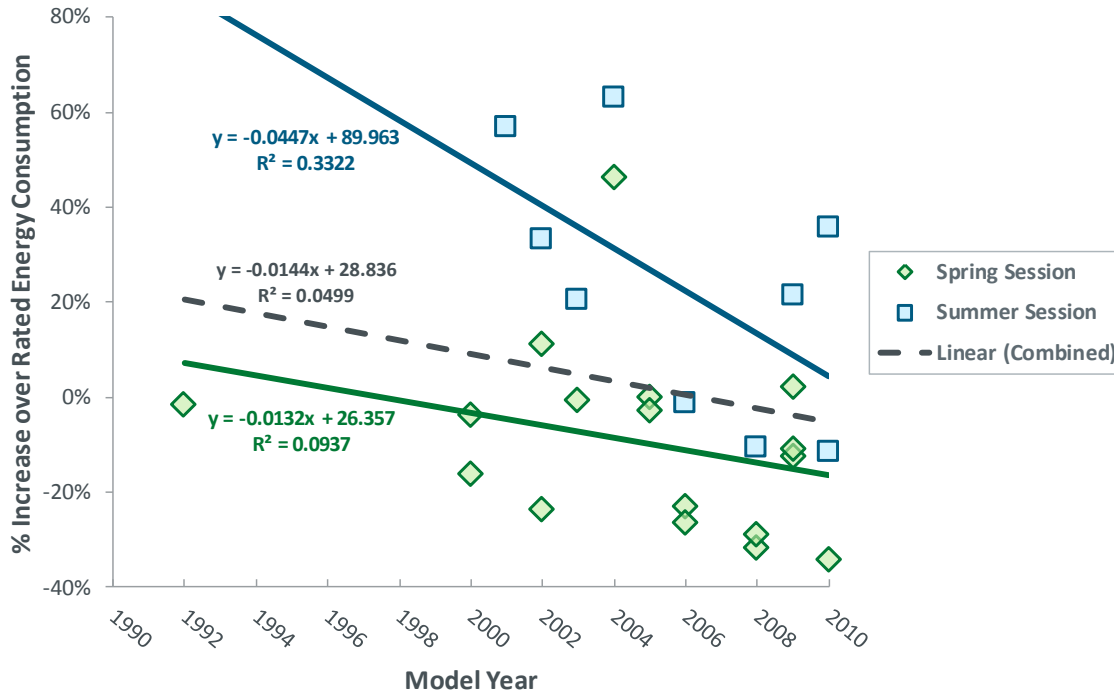
Figure 15. Percent increase over rated energy consumption as a function of model year
