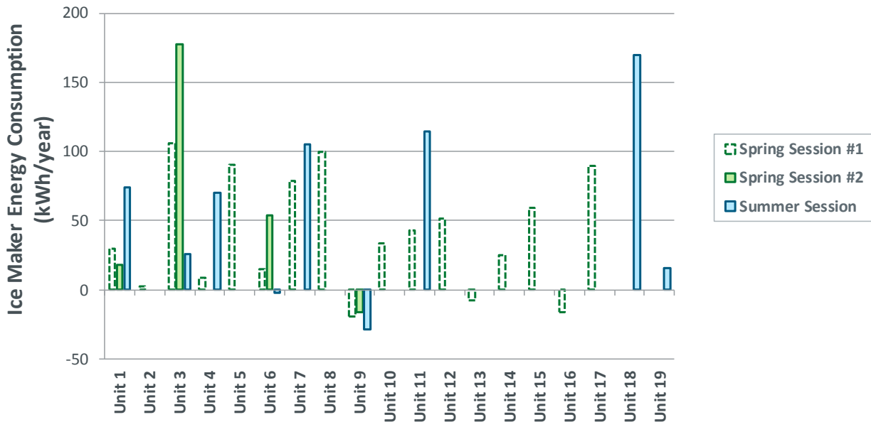
Figure 16. Ice maker energy consumption of each unit in the field study
