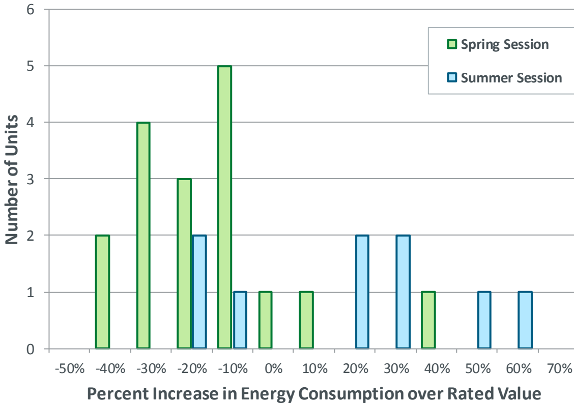
Figure 12. Distribution of percent increase in energy consumption over rated value
