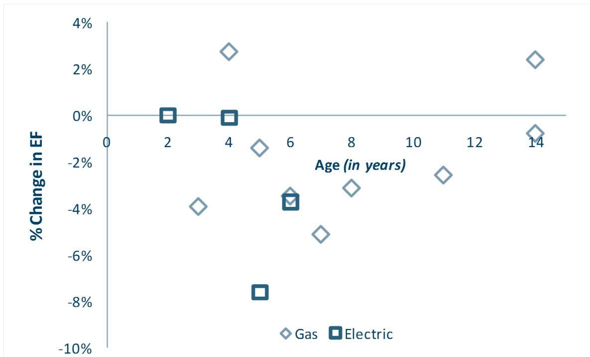
Figure 4: Plot of percent change in Energy Factor with age show no clear correlation between performance decline and age.
