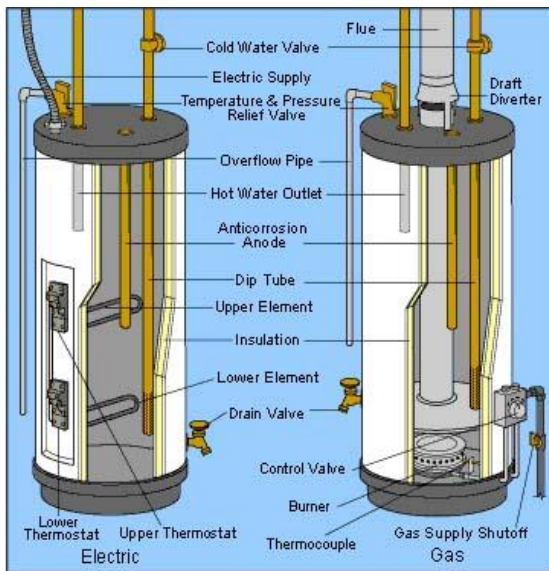
Figure 5: Components of storage water heaters – electric and gas (Source: www.theplumbinginfo.com )
