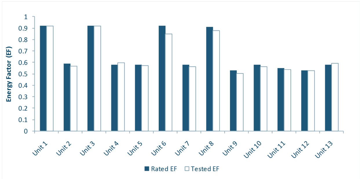
Figure 3: Comparison of Rated and Tested Performance of Water Heater Samples
