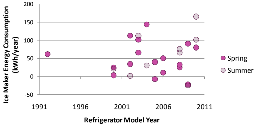
Figure 18. Ice maker energy consumption as a function of refrigerator model year
