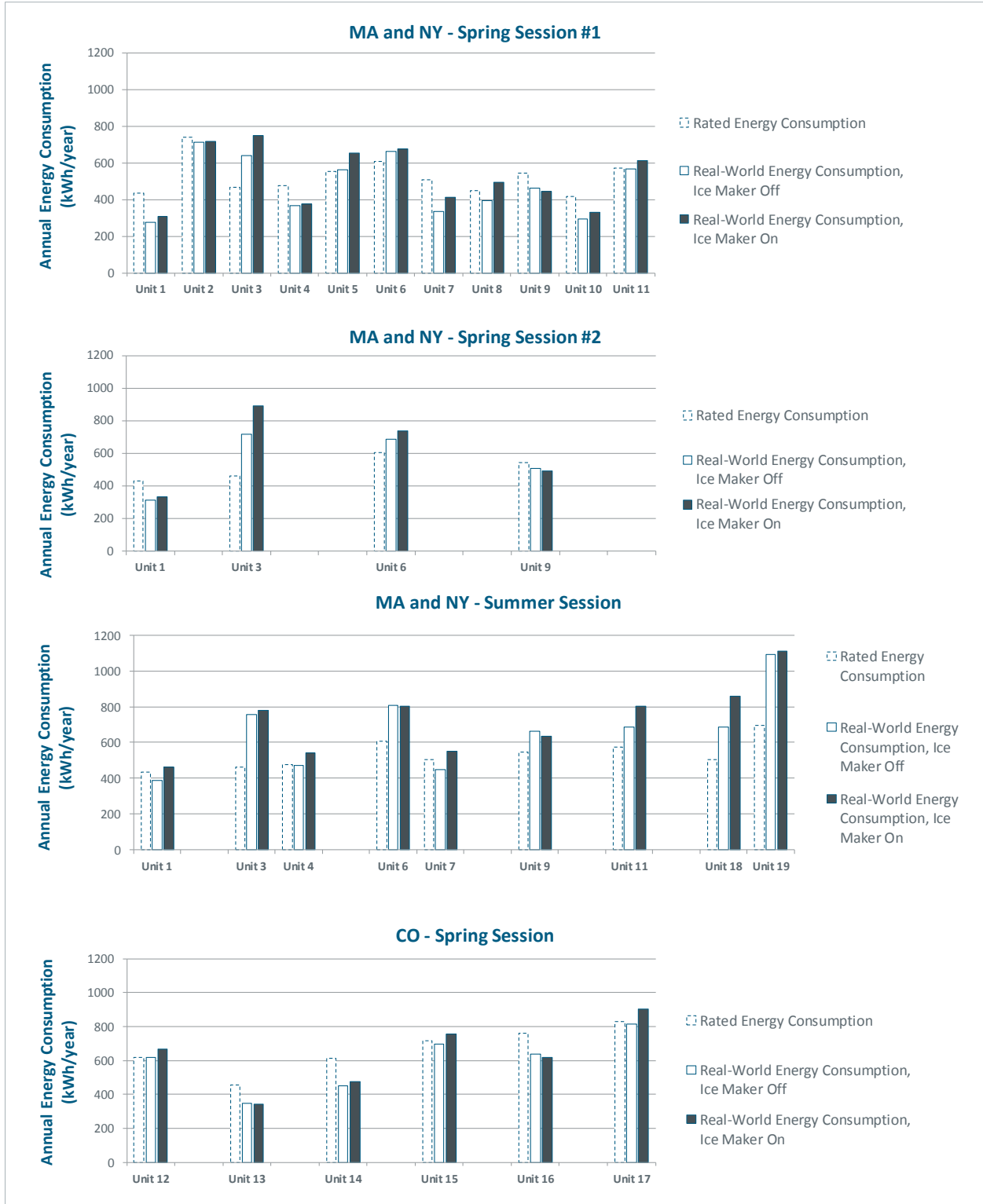
Figure 10. Comparison of rated energy consumption, energy consumption with ice maker off, and energy consumption with ice maker on
