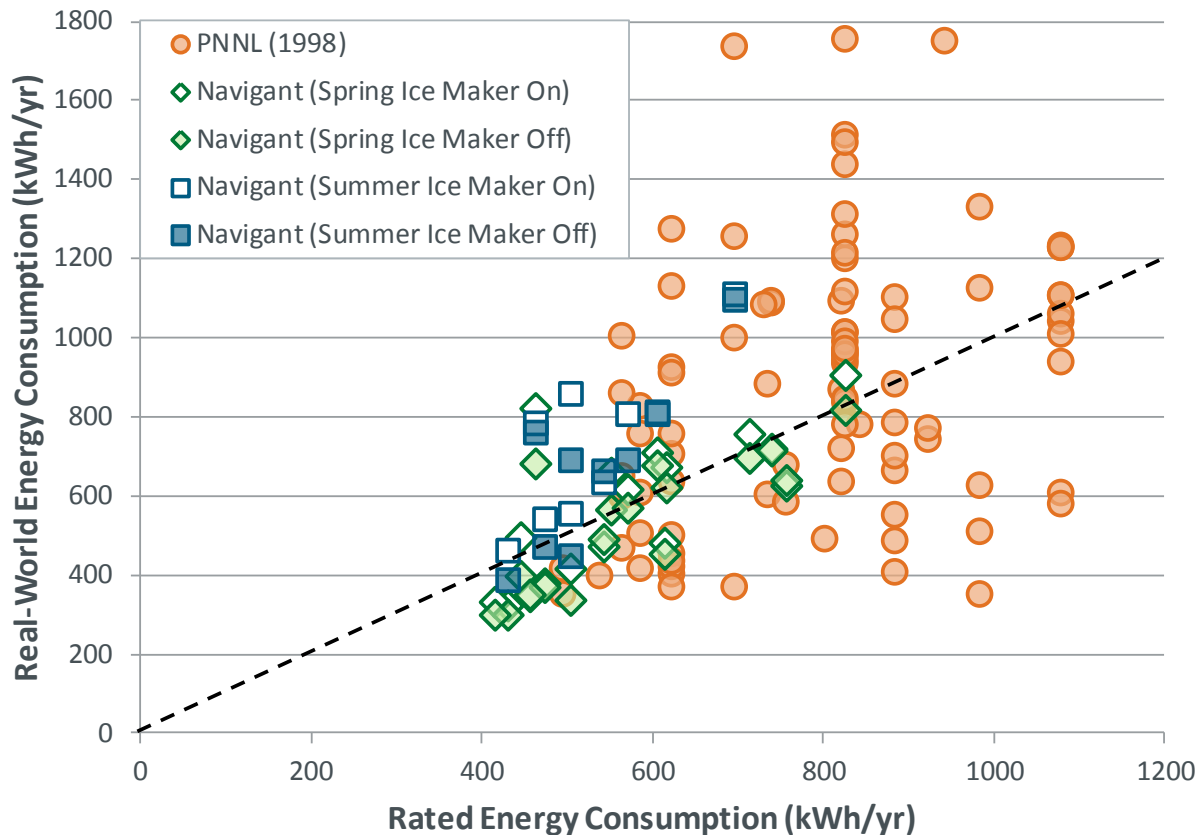
Figure 13. Comparison between real-world energy consumption and rated energy consumption – PNNL vs. Navigant (Source: PNNL 1998)
