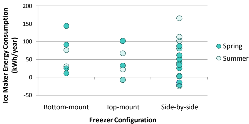
Figure 20. Ice maker energy consumption as a function of freezer configuration
